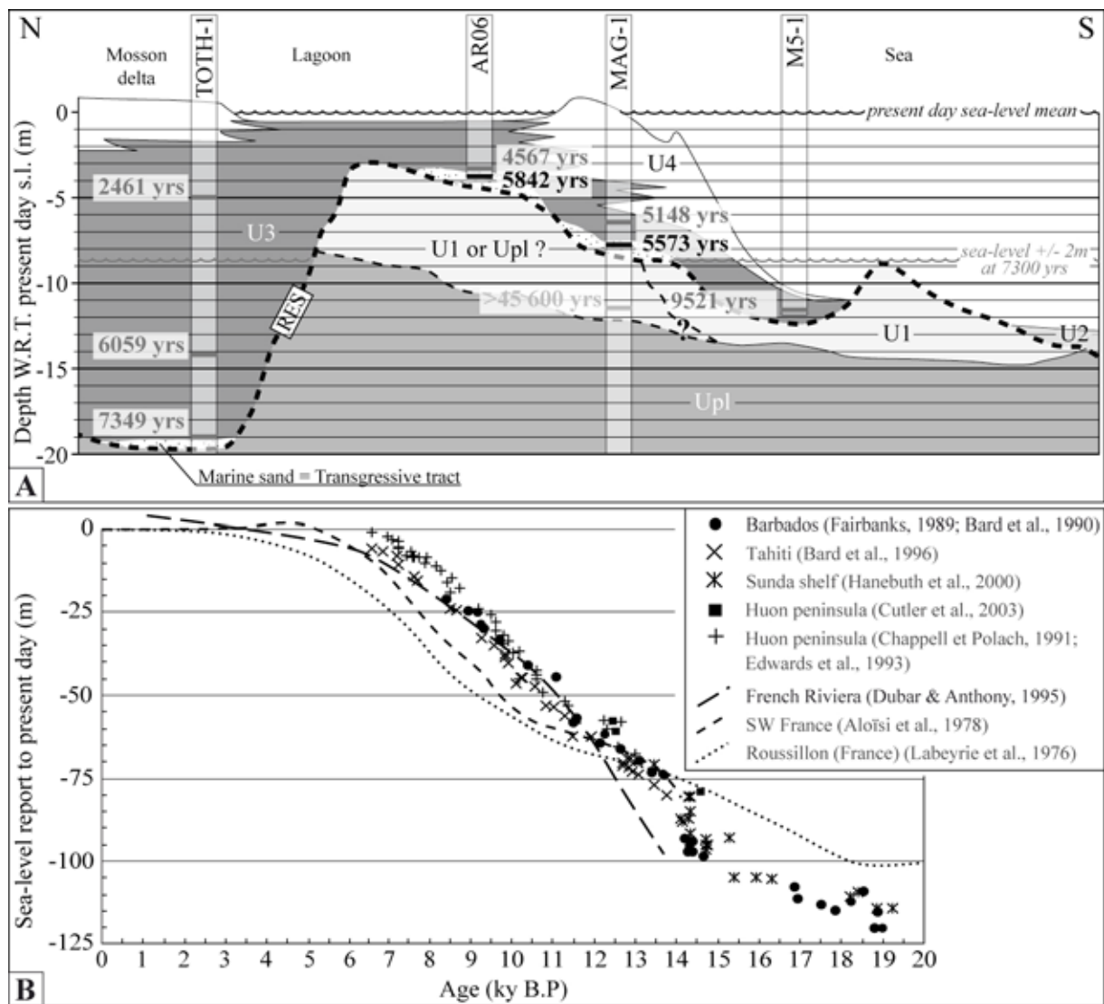
FIG. 4.8 – (A) Schematic representation of legs with position depth w.r.t. present-day sea-level of ^{14}\text{C} datings, in North-South section in Maguelone area. Datations in dark grey correspond to lagoonal deposits and in black to the transgressive tract. Dashed-line in bold corresponds to the RES. (B) Compilation of sea-level changes data showing the last deglacial evolution. The three dashed-lines correspond to Mediterranean sea-level studies. Others correspond to studies of global sea-level changes.
