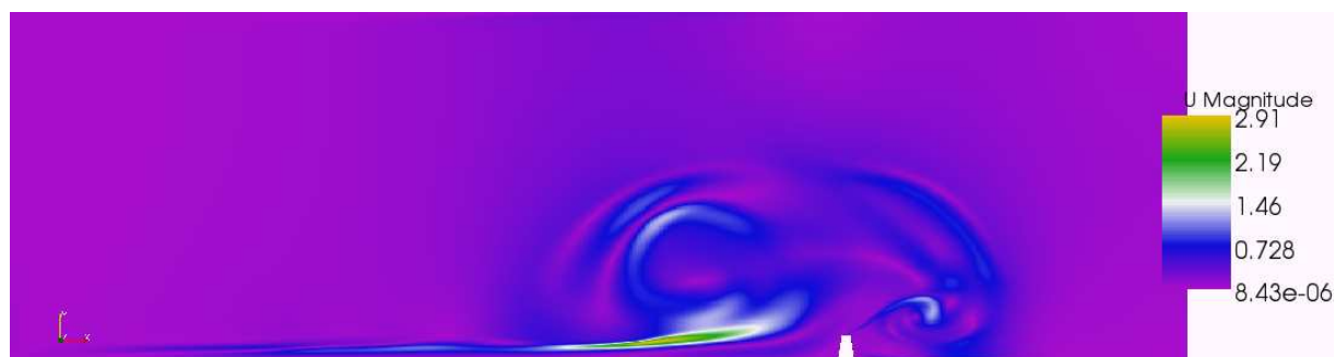
Figure 7.10: Magnitude of two velocity fields difference computed according to the standard and new models at t = 60 s. The color scale ranges from 0 m/s to the maximum value 2.91 m/s.
