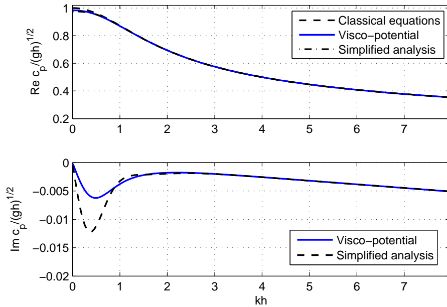
Figure 3.1: Real and imaginary parts of the phase velocity at t = 2 \text{ s} .
