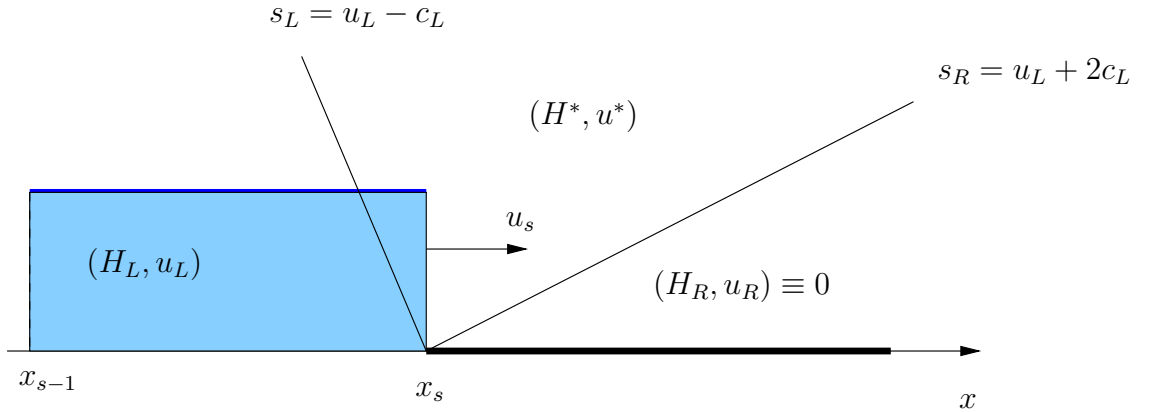
Figure 4.34: Shoreline Riemann problem (left) and wave propagation speeds.
