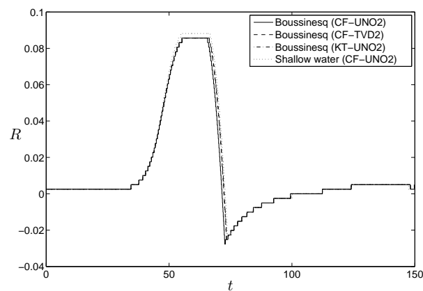
Figure 5.9: Runup value R as a function of time: A_s = 0.0185 case.
