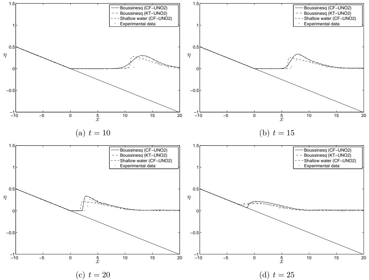
Figure 5.13: Solitary wave runoff on a sloping beach: A_s = 0.28 case.
