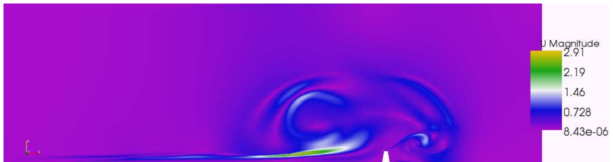
Figure 7.10: Magnitude of two velocity fields difference computed according to the standard and new models at t = 60 s. The color scale ranges from 0 m/s to the maximum value 2.91 m/s.
