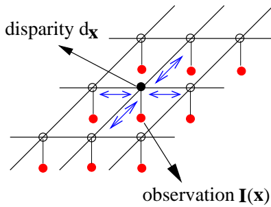
Figure 2.4: Disparity MRF: the observed data \mathbf{I}(\mathbf{x}) refers to the left and right image data and d_{\mathbf{x}} \in \mathbf{d} refers to the disparity at the pixel position \mathbf{x} = (x, y)
