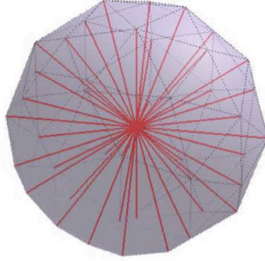
Figure 5.4: The red lines represent the directions for the normals from the origin, obtained by subdivided icosahedron.
