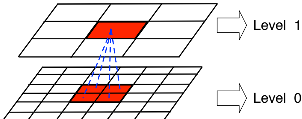
Figure 4.7: The two levels of the multi-grid method are illustrated. Each node at every level l corresponds to a 2 \times 2 block of nodes in the level l - 1 .
