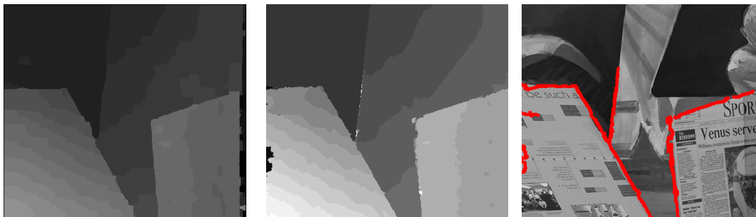
(a) BP results without cooperative boundary extraction (b) Disparity map using proposed approach (BP) (c) Object boundary with 4.14(b)
