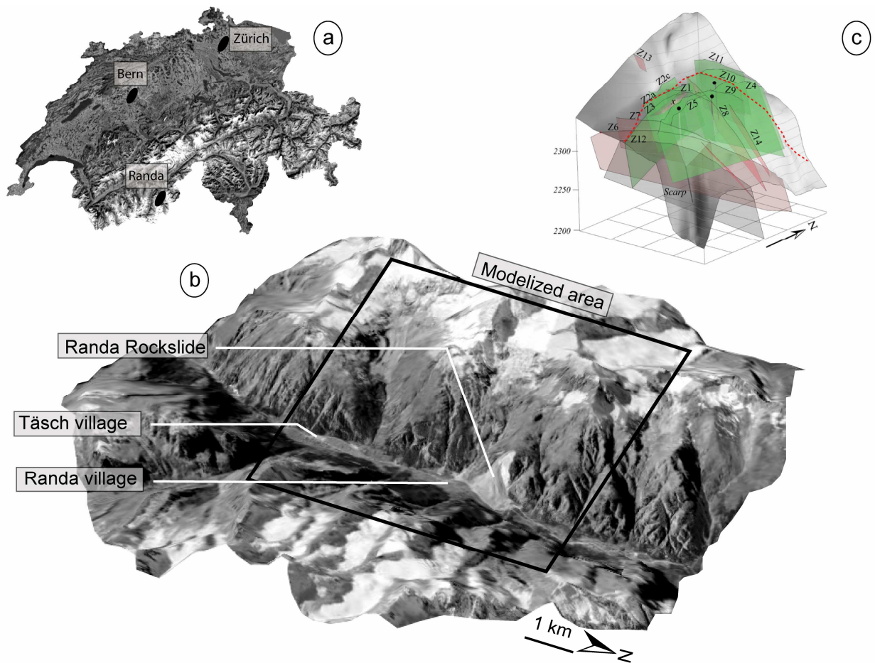
Figure 3-18: Geographical, geological and structural settings of the Grossgauer hillside. (a) Localization of the study area on a general view. (b) part of the Matter valley presenting the modeled zone.. (c) Structural setting of the Grossgauer hillside after Willenberg et al., 2008 (modified).
