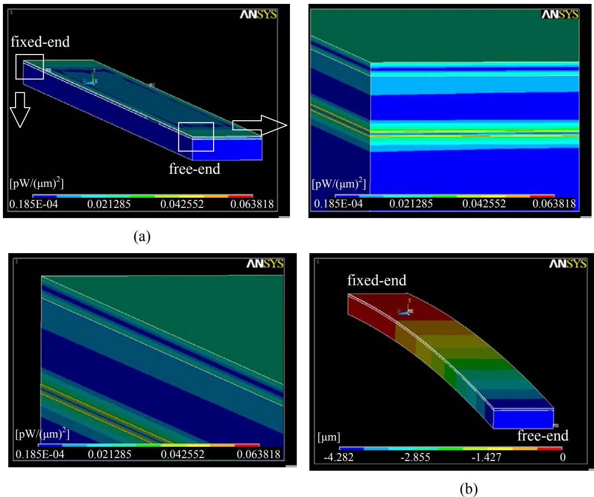
Fig.4.9: Temperature influence results obtained for 800 \mu m long cantilever modelling with h_{AIN} = 1.4 \mu m : thermal flux vector sum (a) and shape, i.e. out-of-plane displacement (b) distribution at 100^\circ C relating to T_{normal} = 20^\circ C
