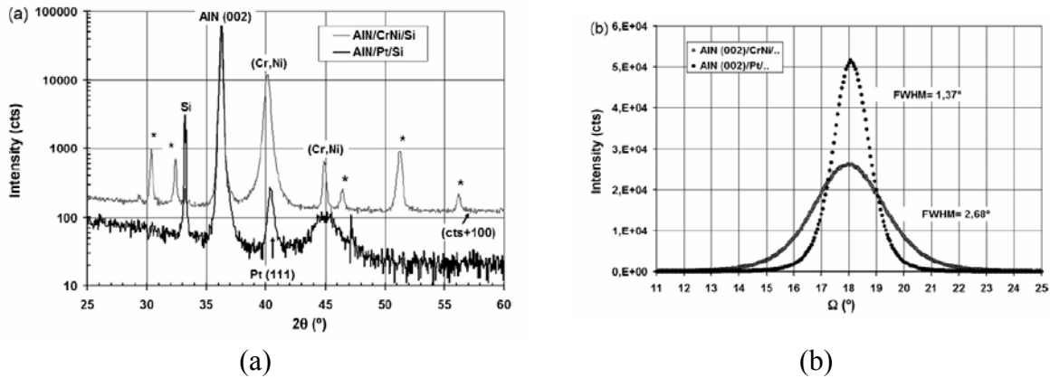
Fig.5.1: X-ray spectrums obtained for AlN on CrNi and Pt (a), rc FWHM for (002) oriented AlN (b)
