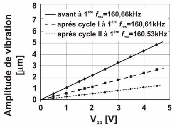
Fig.6.13: Changes of resonant vibration amplitude vs. sinusoidal voltage V_{pp} induced by aging under high humidity performed in the Institute of Aviation for 400 μm long sample with h_{AIN} = 1.0 \mu\text{m}
