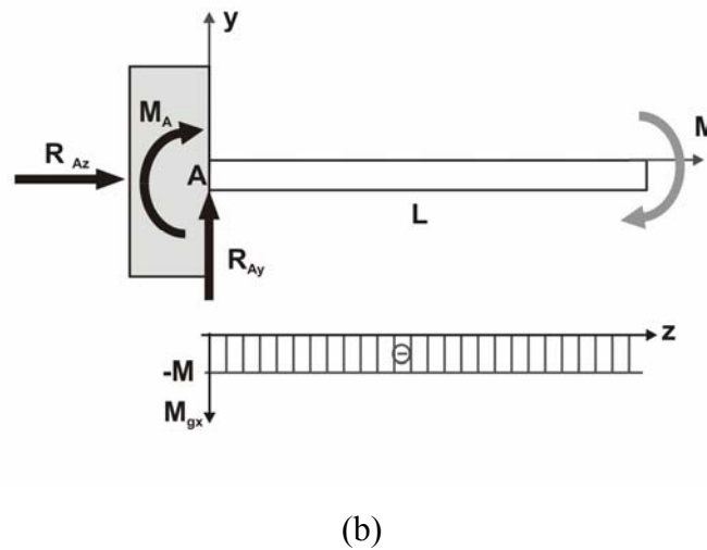
Fig.A4.2: Scheme of cantilever loaded by concentrated force applied to its free end (a) and constant moment (b) including constraint reactions
