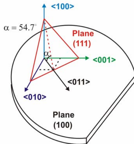
Fig.A2.2: Location of crystallographic planes and directions in (100) oriented silicon wafer [Madou 1997]
