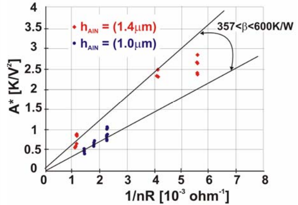
Fig.5.20: Coefficient A^*_{\text{exp}} vs. inverse of device resistance measured for 800 \mu\text{m} long cantilevers in short circuit
