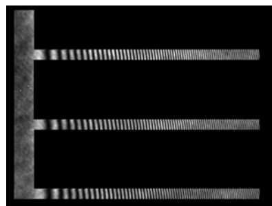
Fig.5.4: Initial deflection measurement of 800 \mu\text{m} long cantilever – exemplary interferogram
