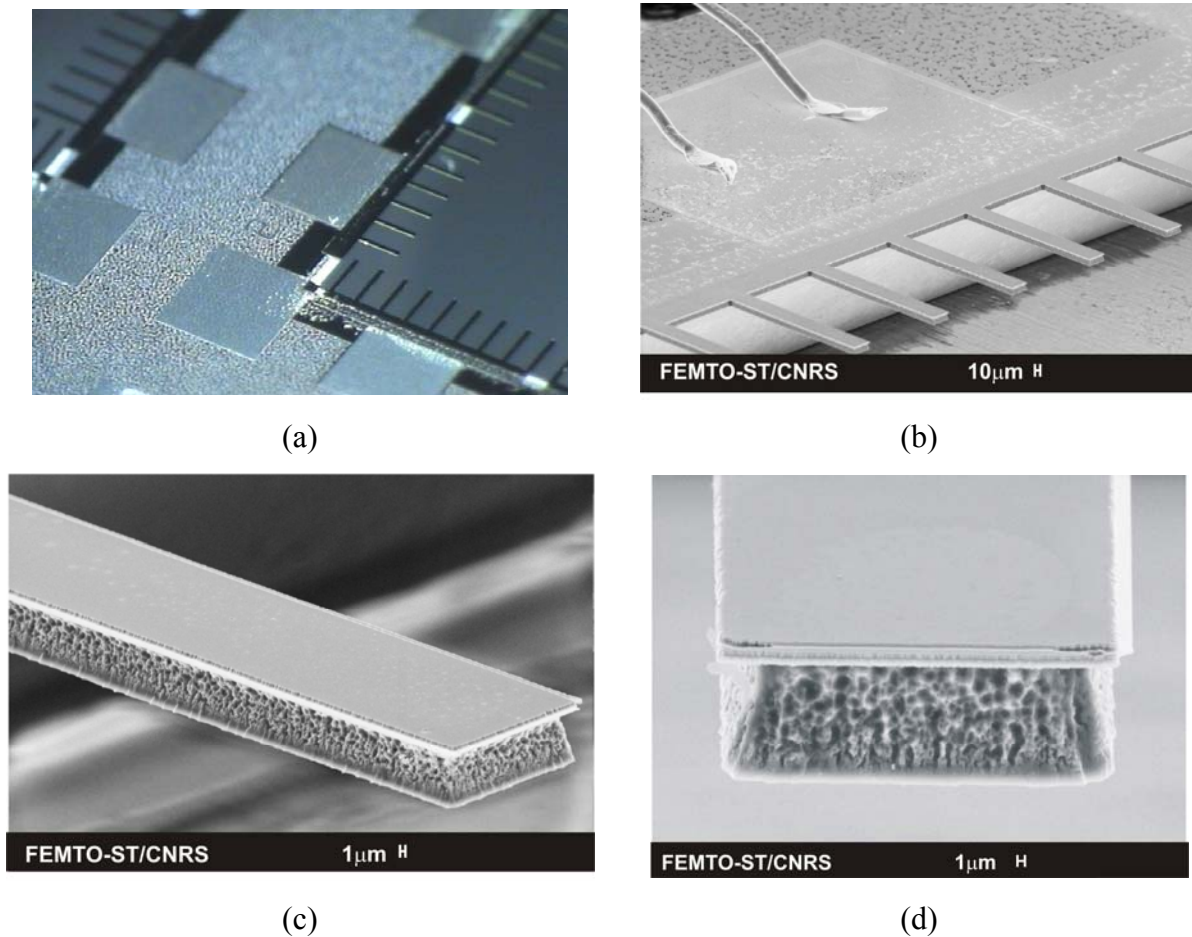
Fig.3.12: Optical microscope and SEM images obtained for 200 μm long microcantilevers fabricated during modified technological process
