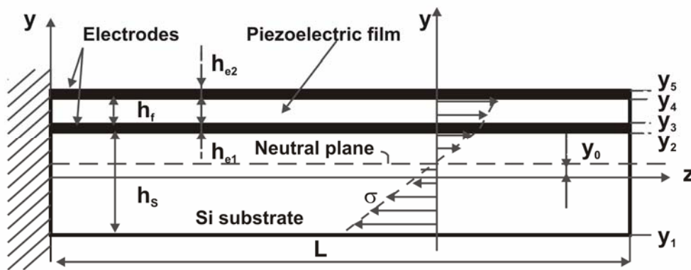
Fig.4.1: Stress distribution in cross-section of multilayer bending cantilever [Brissaud 2003]
