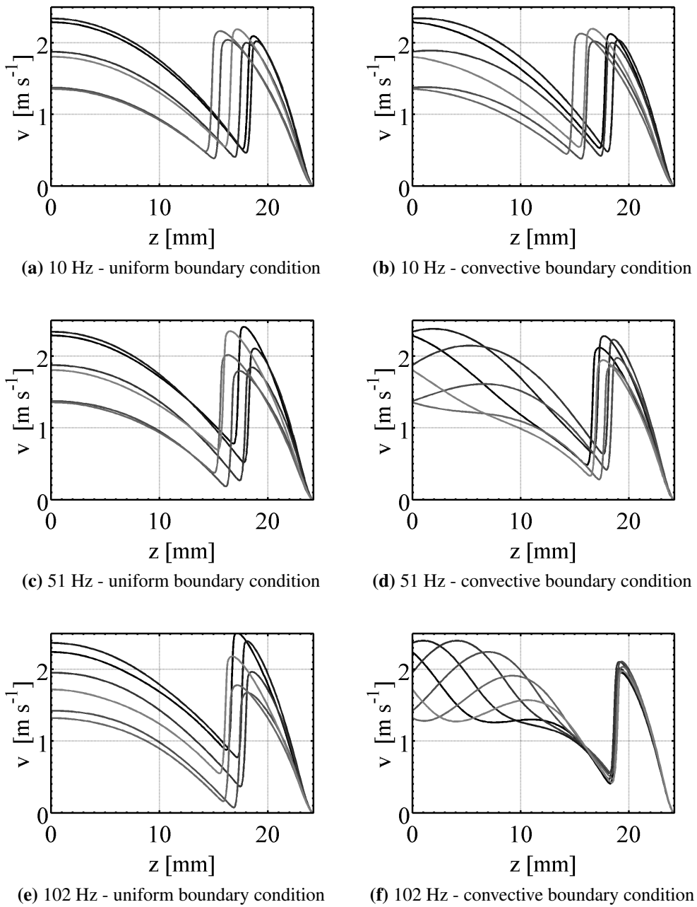
Figure 3.28: Axial velocities obtained from simulations of flame P versus z -coordinate. (v_{rms}/\bar{v})_R = 0.20 - Gray levels indicate different instants in the time period.
