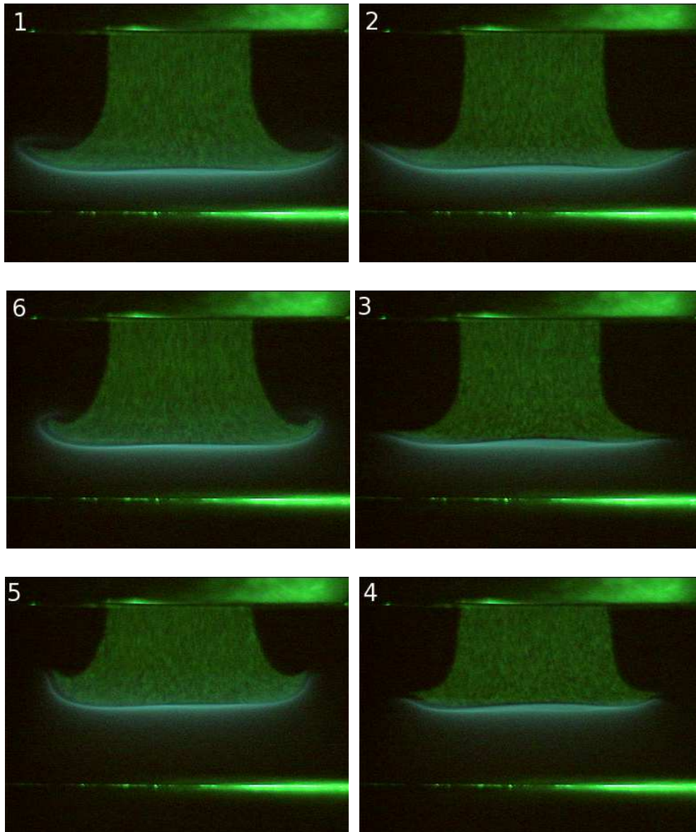
Figure 3.7: Tomographic views of the flow and flame structures in flame P configuration for a forcing frequency f = 10 Hz and a fluctuation level (v_{rms}/\bar{v})_R = 0.20 - Six images taken at instants separated by an equally phase shift describe a whole cycle clockwise. Distance between the plate and the burner outlet H = 24.2 mm.
