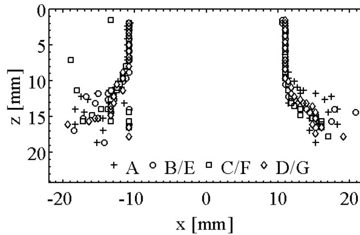
Figure 5.6: Trajectories of maxima of swirling strength \lambda_{ci} - on the right, flames A, B, C and D - on the left, flames A, E, F, G
