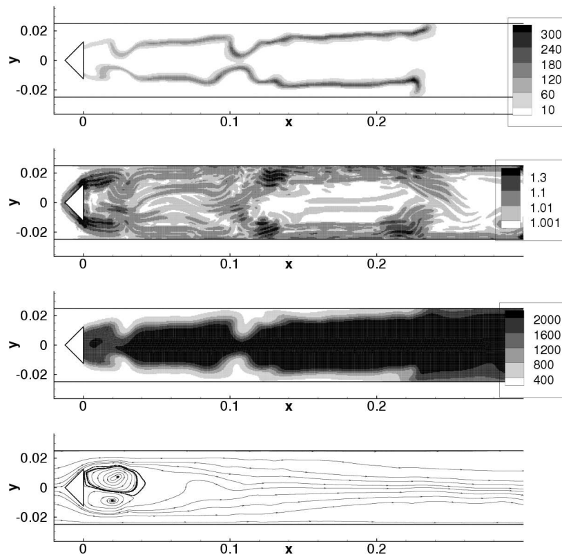
Figure 3.11 : Instantaneous resolved fields of the flame computed using Colin’s model. First reaction rate ( \text{kg/m}^3 \cdot \text{s} ), efficiency function, temperature ( \text{K} ) and the streamline (top to the bottom) thickening factor F = 20 .
