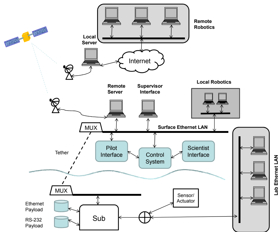
Figure 1.11: Communication Architecture for teleoperation of ROMEO ROV
