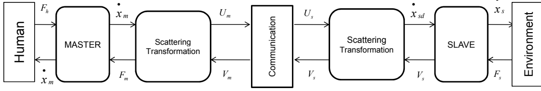
Figure 3.5: Bilateral Teleoperation with time delay
