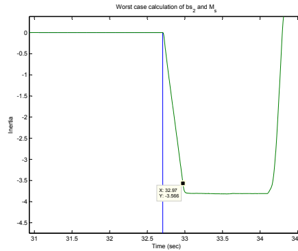
Figure B.1: Worst case approximation of M_s and Bs_2 (without wheels)
