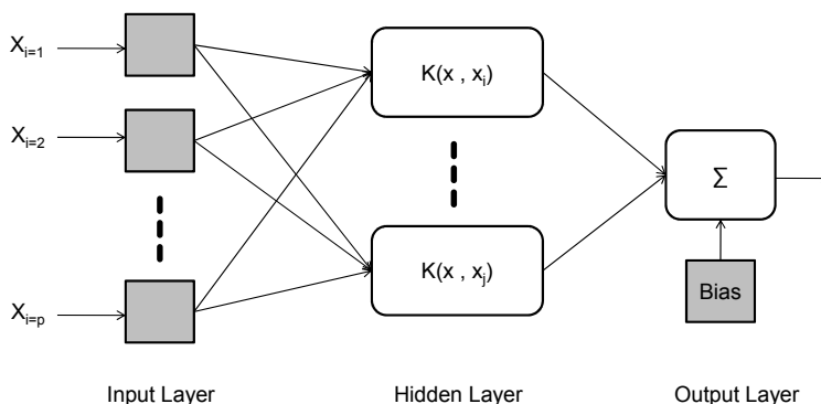
Figure 4.9: SVM Architecture
