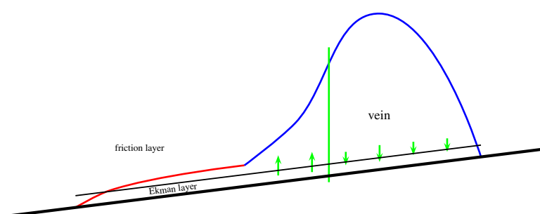
Fig. 2 Schematic of a cross section through a gravity current on an inclined plane as considered in this manuscript. The total gravity current consists of two distinct parts, the vein (the fluid under the blue line) and the friction layer (the fluid under the red line). In both parts, there is an Ekman layer close to the inclined
