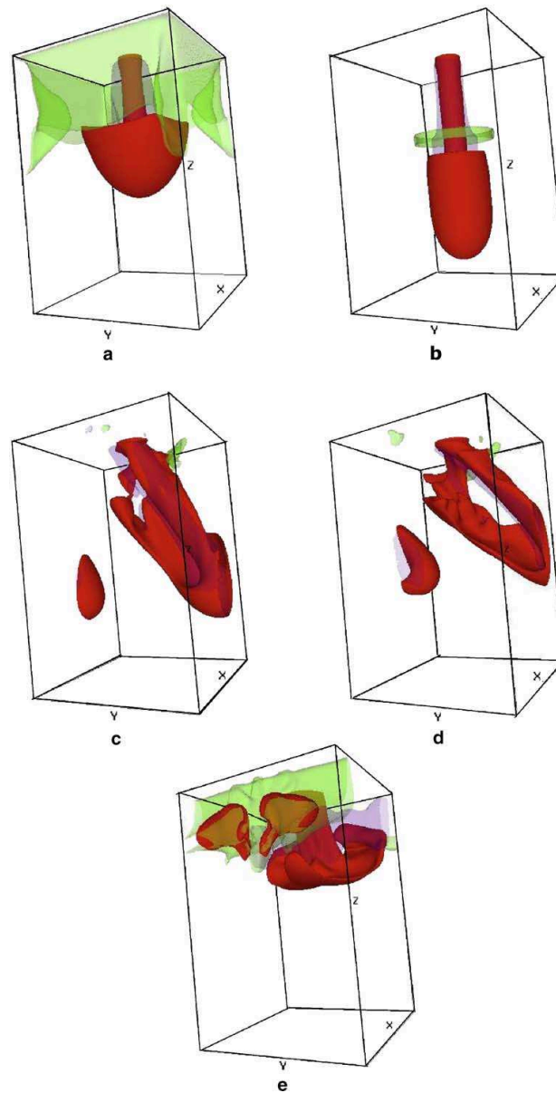
Fig. 1. Temperature isosurface \Delta T = 5.0 \times 10^{-4} K (red) and vertical velocity isosurfaces w = -.01 m/s (violet) and w = .01 m/s (green) at t = 1.5 days after the onset of cooling, for different latitudes on earth (a) NR (no rotation), (b) NP ( 90^\circ N), (c) LS ( 60^\circ N), (d) GL ( 45^\circ N) and (e) EQ ( 0^\circ N).
