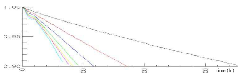
Fig. 6 The part of the gravity current in the vein. One sees a decrease in the volume of the vein differing between the experiments. The curves are, from left to right, for experiments
