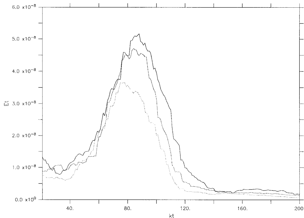
Figure 4. Temporal energy spectrum of \overline{\Psi_2} for k = 2\pi \cdot 11 in three experiments 1, 2 and 4 (from top to bottom) after a 35-point-wide boxcar smoother was applied. The peaks correspond to the time scale of about 200 days.
