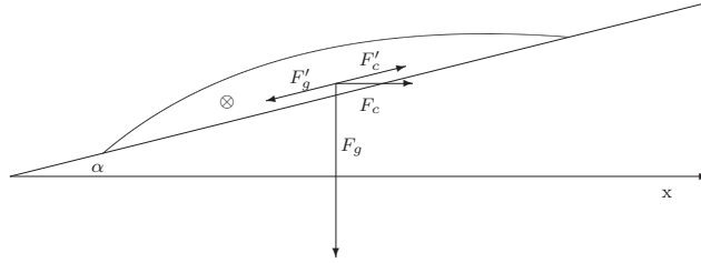
Fig. 1 Cross section of a gravity current with an average geostrophic velocity into the plane. The Coriolis force F_c and the buoyancy force F_g are shown. The fig. establishes the force balance between the projection of the Coriolis force F'_c and the projection of the buoyancy force F'_g onto the topographic slope, for a gravity current on a inclined plane, of angle \alpha , when dissipative processes are neglected.
