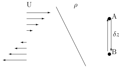
Figure 10.2: Exchanging volumes A and B in a sheared stably stratified flow.
