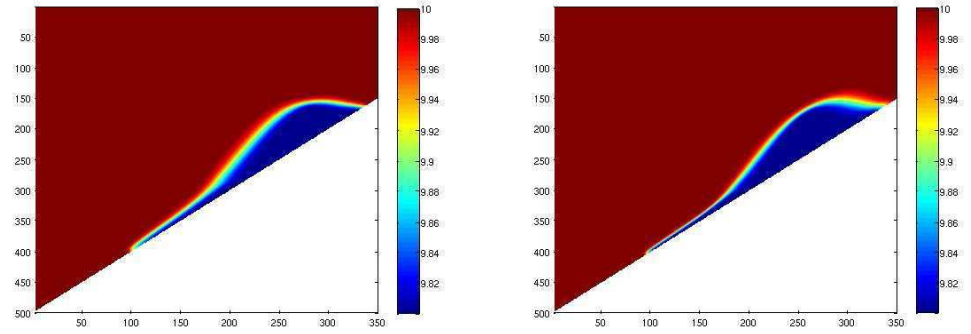
Fig. 2. Temperature structure (in ^{\circ}\text{C} ) in the reference simulations after 2 days; left: z -coordinate (G01) and right: \sigma coordinate (G02). Coordinates give grid in the x -direction and the z -direction for the z -coordinate grid. For the \sigma -coordinate results are interpolated to the z -coordinate grid (in the z -direction)
