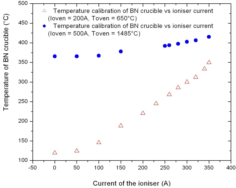
Figure 4.27: Temperature calibration of the boron nitrite crucible versus ioniser current
