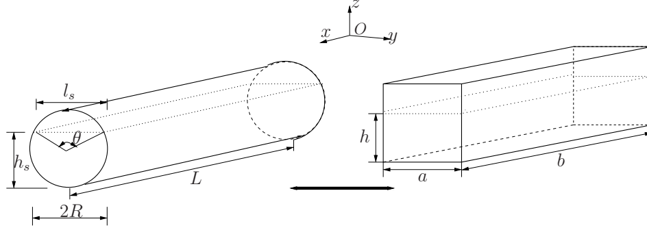
Figure 2.11: Equivalent tanks
