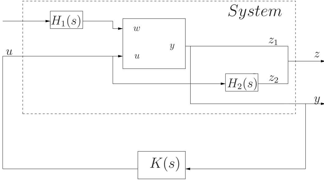
Figure 4.28: Standard H_\infty problem with filters
