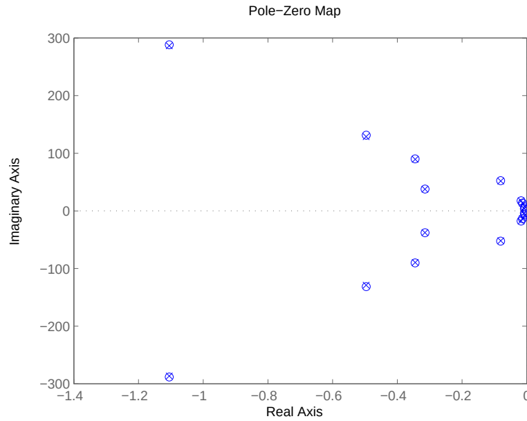
Figure 4.25: Pole/ zero map for the open-loop system augmented with one mode; tank fill level equal 0.9
