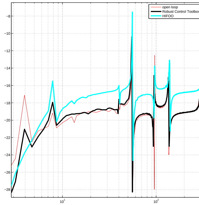
Figure 4.30: Experimental Bode plot of the open-loop system (thin line) and of the closed-loop system using a HIFOO controller and a Robust controller computed with Matlab (2 modes and a fixed tank filling of 0.7)
