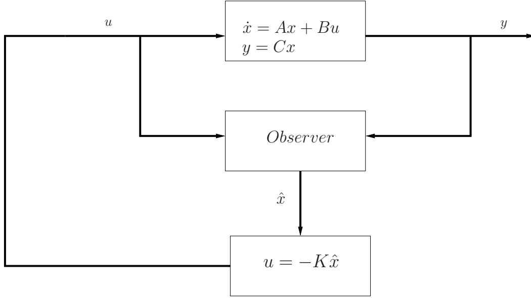
Figure 3.2: Feedback control law and observer
