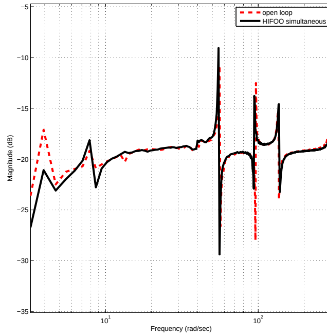
Figure 4.40: Experimental Bode plot of the open-loop system (dotted line) and of the closed-loop system (bold line) using simultaneous HIFOO controller - e = 0.7
