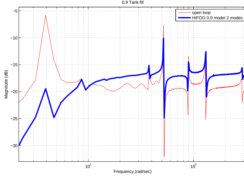
Figure 4.31: Experimental Bode plots of the open-loop system (thin line) and the closed-loop system (bold line) with a HIFOO controller computed for 2 modes and a fixed tank filling of 0.9
