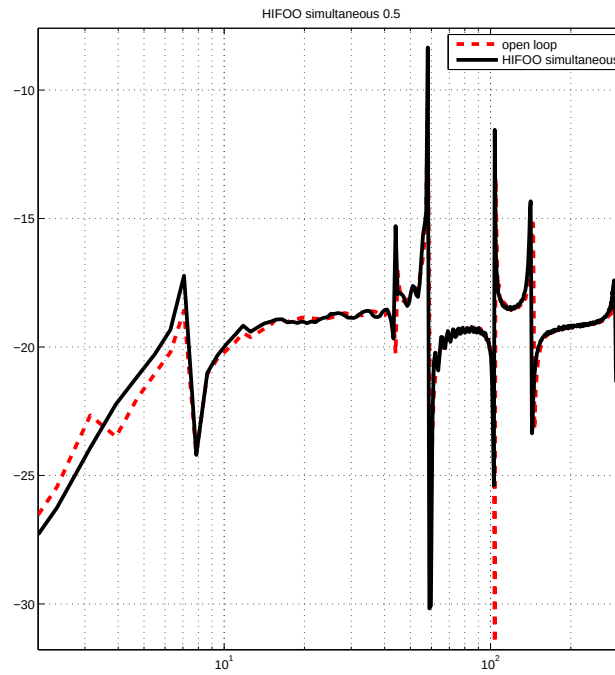
Figure 4.41: Experimental Bode plot of the open-loop system (dotted line) and of the closed-loop system (bold line) using simultaneous HIFOO controller - e = 0.5
