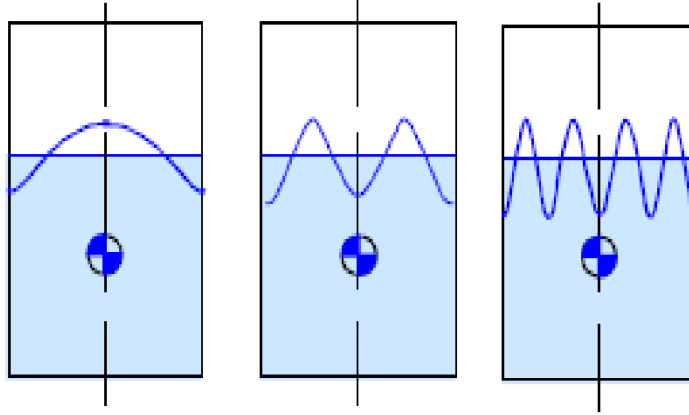
Figure 2.13: The mode shape of the first three symmetric waves (from left to right)
