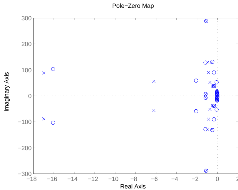
Figure 4.26: Pole/ zero map for the closed-loop system augmented with one mode and with the controller computed with d_{12} = 0.1 ; tank fill level equal 0.9
