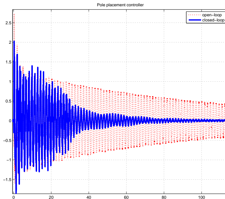
Figure 4.17: Experimental output of the of open-loop (dotted line) and closed-loop (plain line) systems using a pole placement controller with a tank fill level of 0.9
