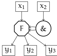
FIGURE 3.3: Arithmetic circuit where a node has been syntactically substituted by a circuit F with 3 inputs and 3 outputs.
