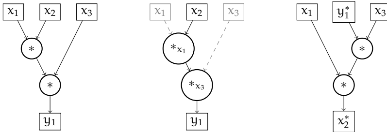
FIGURE 3.4: A circuit over a commutative ring, its linearization for \ell = \{x_2\} (scalar edges are grayed out), and its \ell -dual.
