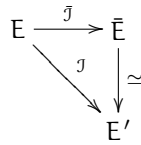
FIGURE 8.2: Using Vélu formulas to compute an explicit isogeny.
