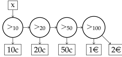
FIGURE A.1: The coffee machine circuit. On input n \in \mathbb{Z} , the operator >_x: \mathbb{Z} \rightarrow \mathbb{Z} \oplus \mathbb{Z} gives n on its right output if n > x , on its left output otherwise. The circuit is an euro coin separator.
