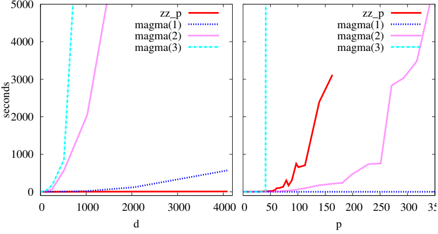
FIGURE 6.3: Build times with respect to d (left) and p (right).
