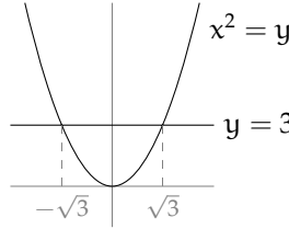
FIGURE 5.1: Plot in the reals of the ideal I = (y - 3, x^2 - y) .
