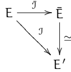
FIGURE 8.2: Using Vélú formulas to compute an explicit isogeny.
