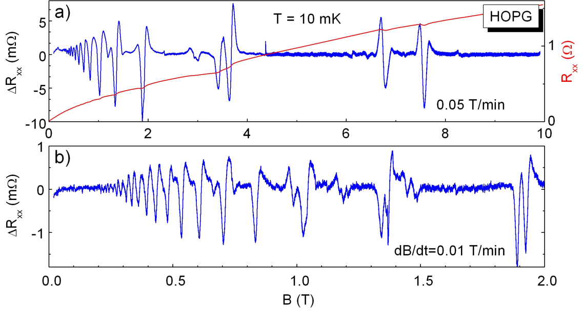
Fig. 5.9: a) Right axis: Resistance R_{xx} vs. B measured at T = 10 mK for HOPG. R_{xx} increases linearly with the magnetic field, with the superimposed quantum oscillations being more distinct than in the higher temperature data (Fig. 5.1). a) and b) Left axis: Background removed data \Delta R_{xx} showing quantum oscillations measured over different magnetic field regions with different sweep rates.
