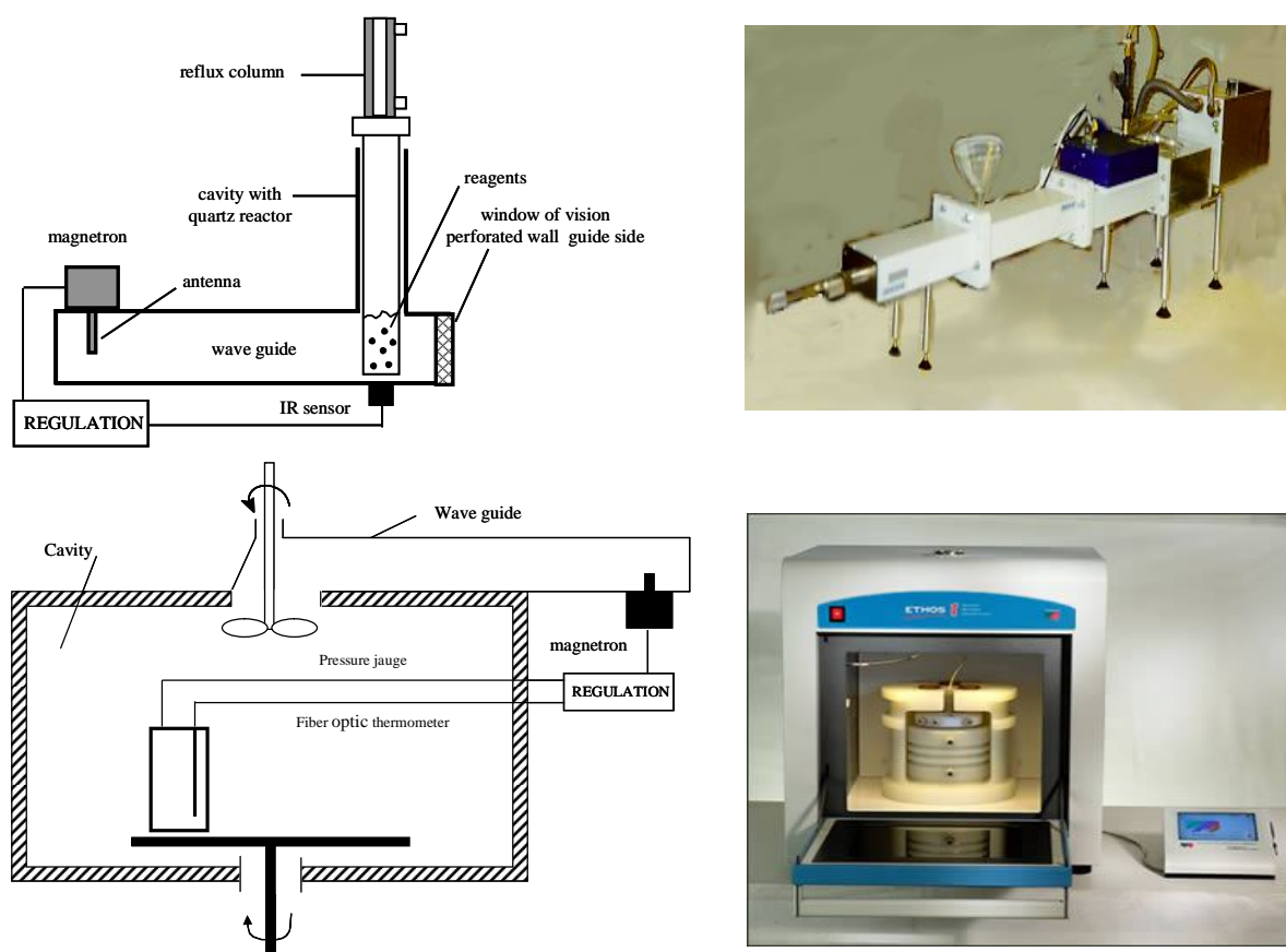
Figure 1: Monomode and multimode microwave ovens
