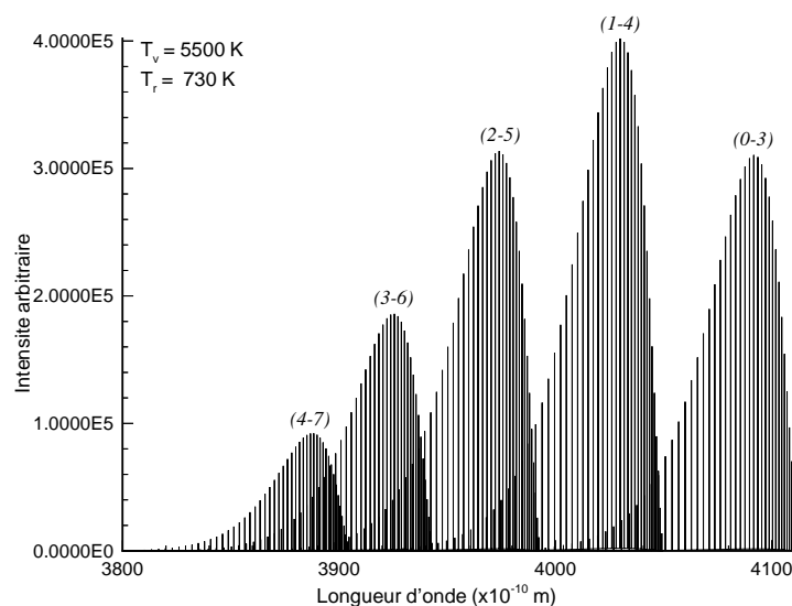
Figure 2.21. Transition électronique 2^+ ( N_2(C^3\Pi_u) \longrightarrow N_2(B^3\Pi_g) ), branche R ( \Delta J = +1 )
