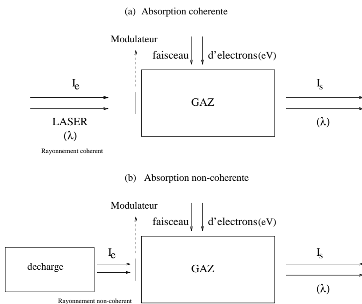
Figure 2.5. a) Absorption cohérente ; b) Absorption non-cohérente
