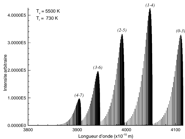
Figure 2.19. Transition électronique 2^+ ( N_2(C^3\Pi_u) \longrightarrow N_2(B^3\Pi_g) ), branche P ( \Delta J = -1 )
