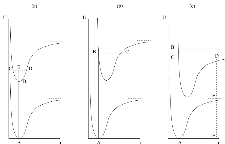
Figure 2.15. Principe de Franck-Condon
