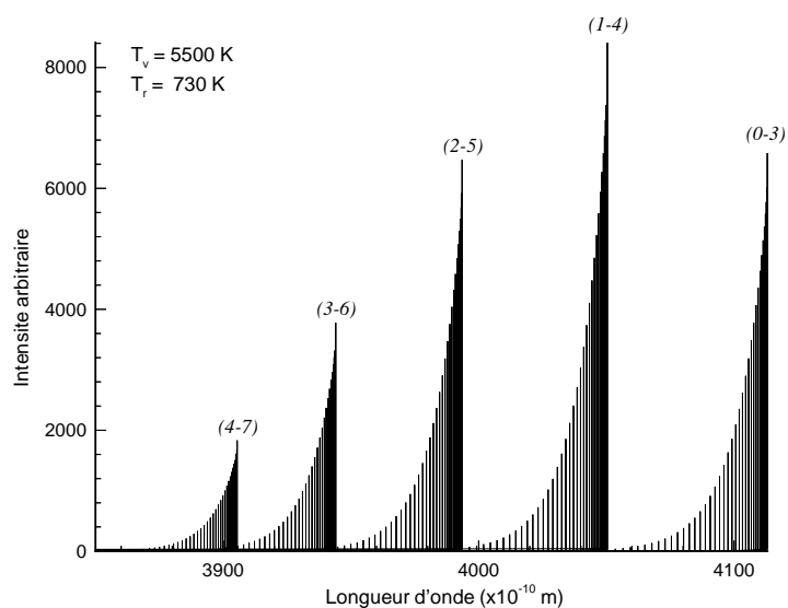
Figure 2.20. Transition électronique 2^+ ( N_2(C^3\Pi_u) \longrightarrow N_2(B^3\Pi_g) ), branche Q ( \Delta J = 0 )
