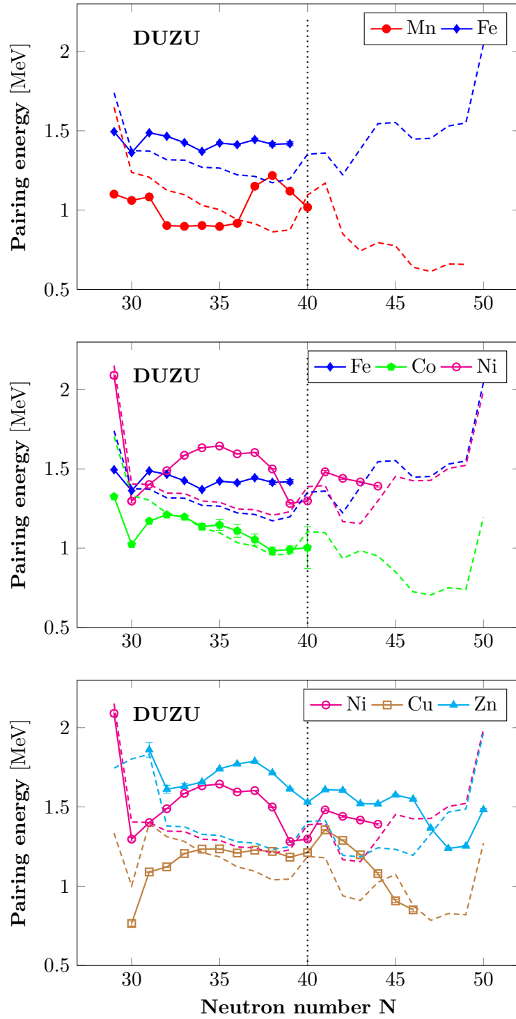
Figure 6.19.: Pairing energy versus N . For each isotopes chain the data are shown (solid lines) with comparison to the Dufo-Zuker predicted values (dashed lines).
