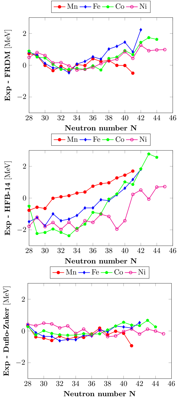
Figure 6.6.: Difference between binding energies calculated in the FRDM, HFB-14 and Duflou-Zuker models and measured binding energies.
