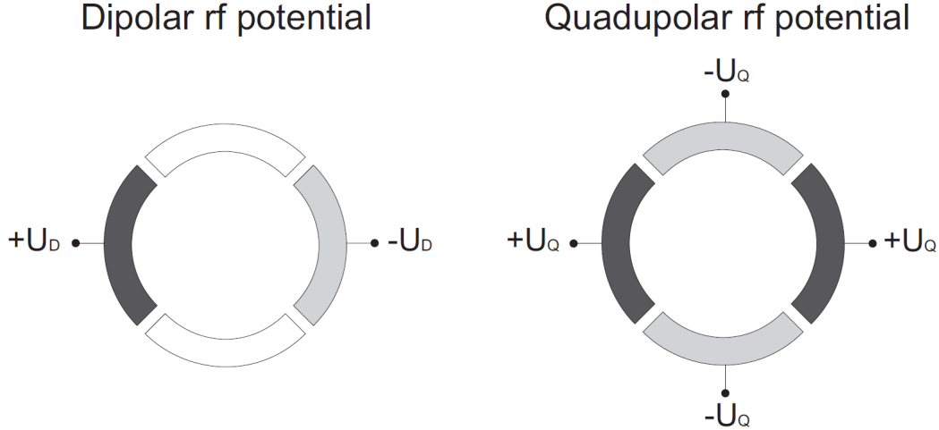
Figure 3.3.: Radial segmented ring electrode (top view) of a Penning trap to apply an electromagnetic radiofrequency field. (left) Dipolar radiofrequency field between two opposite ring segments in phase with the ion motion. (right) A quadrupolar field can be generated by applying a radiofrequency field between each opposite pairs of the four-fold segmented ring electrode.
