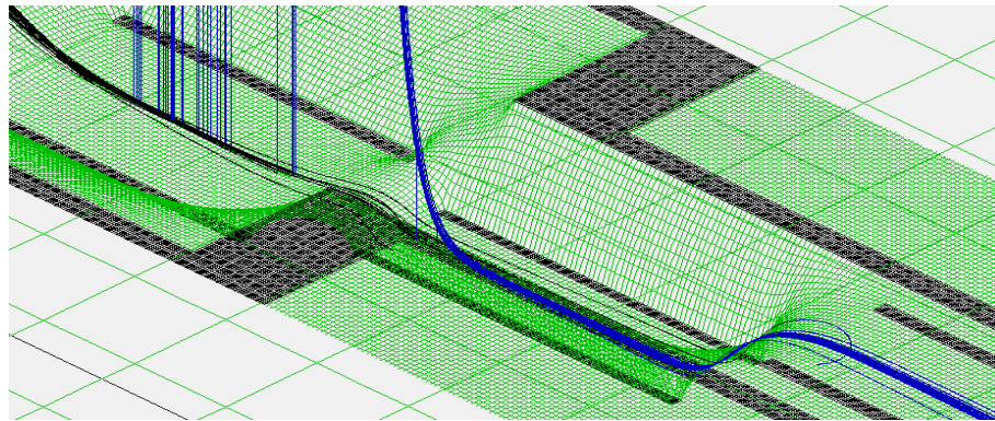
Figure A.7.: (top) Electric potential surface of same simulation in Figure A.6 . One can see how the ions are lifted from -1.5 kV to 30 kV. The zoom (bottom) shows that all ions are not lifted at the same place in the electrode because of their different time-of-flight (all ions are lifted at \approx 172\mu s after their ejection from the trap).
