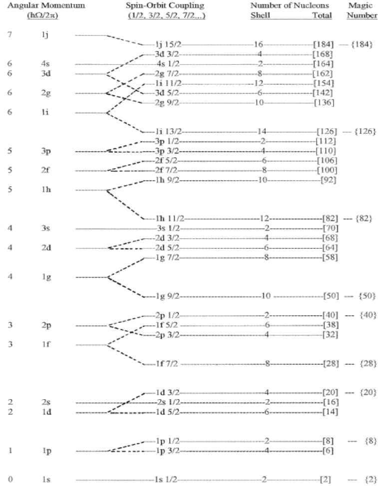
Figure 2.2.: Shell model.
