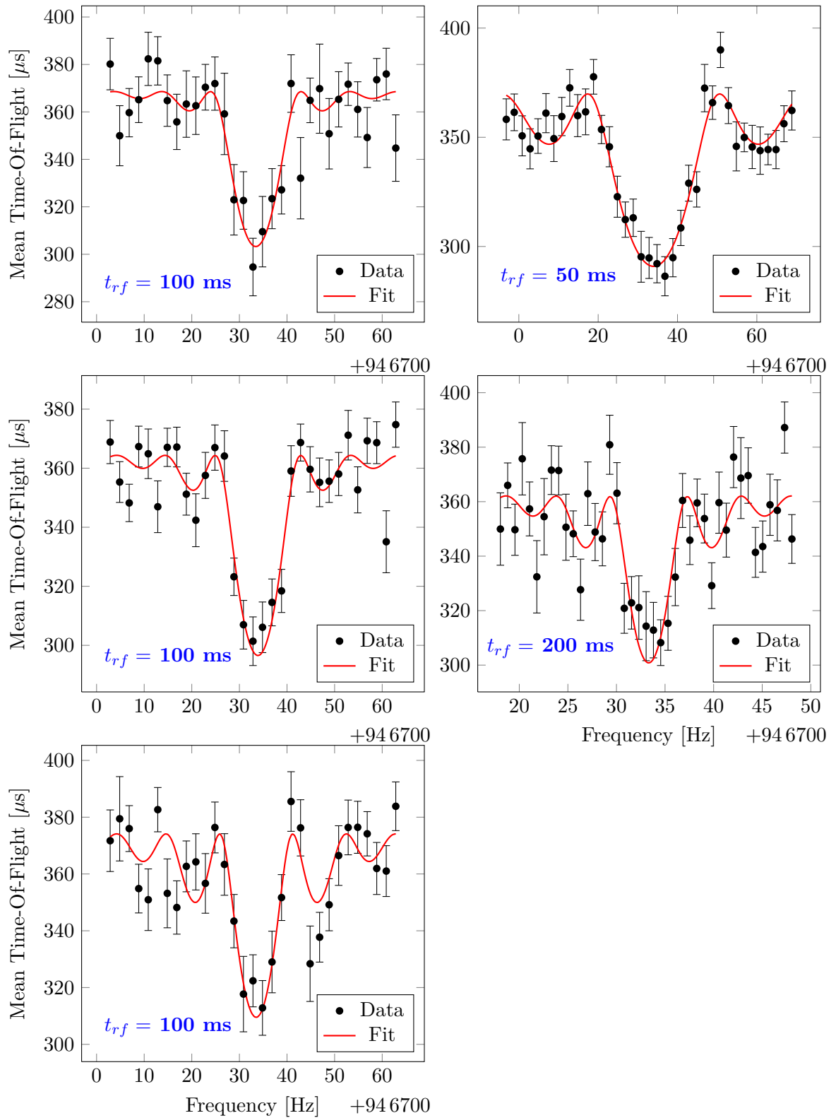
Figure B.2.: TOF resonances of ^{96}\text{Kr}^+ from the precision Penning trap. Excitation time T_{rf} = 100 ms (left), T_{rf} = 50 ms (top right) and T_{rf} = 200 ms (bottom right).
