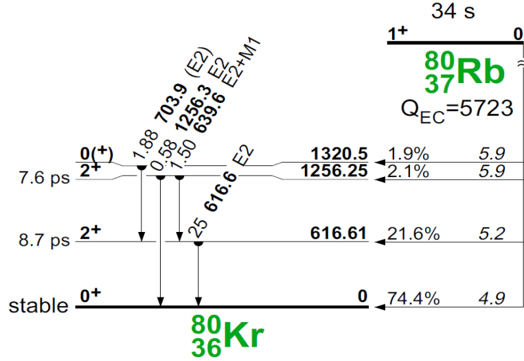
Figure A.11.: Decay scheme of ^{80}\text{Rb} (from [Fir+99])
