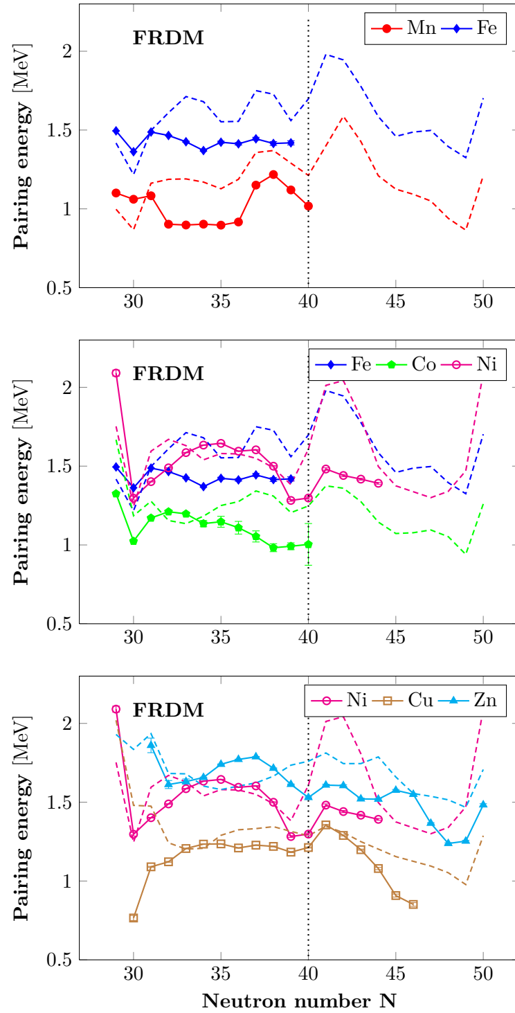
Figure 6.18.: Pairing energy versus N . For each isotopes chain the data are shown (solid lines) with comparison to the FRDM predicted values (dashed lines).
