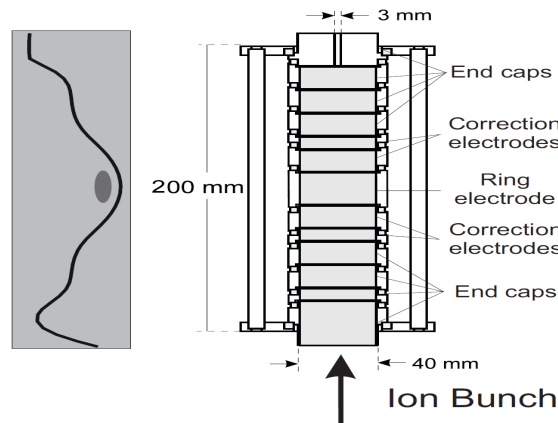
Figure 4.3.: Schematic view of the preparation Penning trap (right), and the axial potential (left). The ion bunch is shown trapped in the harmonic part of this potential.
