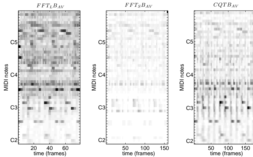
Figure 3.18: Pitch class spectrum of the first seconds of the song Love Me Do . From left to right: FFT_L B_{AV} , FFT_S B_{AV} and CQT B_{AV} .
