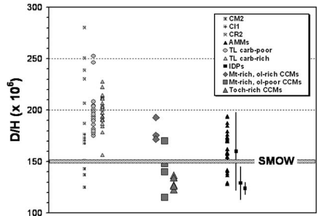
Fig. 5. Comparison of CCMs phyllosilicates' structural water D/H ratios with phyllosilicates' structural water D/H ratios of carbonaceous chondrites, and micrometeorites. For CCMs, each point is either a single measure, or the average of several data points (Table 4). Data for CM2 and C11 chondrites are from Eiler and Kitchen (2004). Data for the two Tagish Lake lithologies are from Engrand et al. (2003). Data for AMMs and IDPs are from Engrand et al. (1999) and Aléon et al. (2001) respectively. For CR2 chondrites, we have not plotted the Renazzo data reported by Deloule and Robert (1995) because they are not tabulated. These data are compatible with those of Guan and Zolensky (1997). Error bars (except for the three IDPs) have not been plotted for sake of clarity. They are of the order of 4% relative for CCMs, AMMs and Tagish Lake (Engrand et al., 1999, 2003; this work), of 3% for CM2 and C11 data (Eiler and Kitchen, 2004) and between 1 to 3% for CR2 chondrites. Standard Mean Ocean Water (SMOW) D/H ratio is indicated for reference.
