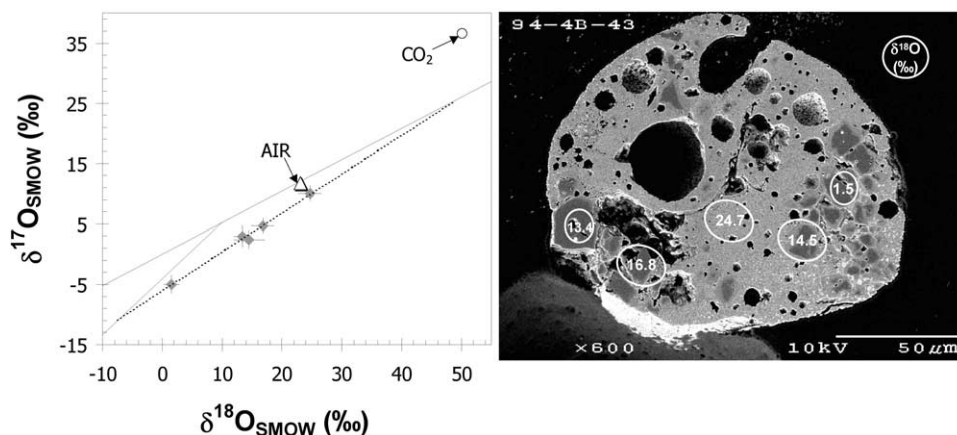
Fig. 13. Oxygen three isotope diagram of the porphyritic olivine partially melted spherule 94-4B-43. This spherule exhibits a range of variation in \delta^{18}O values of more than 20‰. Two olivine grains with about the same composition ( F_{O_{98.7}} and F_{O_{98.8}} ) have \delta^{18}O values that differ by more than 10‰. A best fit through the data gives a linear equation: y = 0.645x - 6.1273 , with R^2 = 0.992 . The values for atmospheric air and atmospheric CO_2 at 60 km altitude are given for reference (Thiemens et al., 1995). The backscattered electron micrograph of this spherule is given on the right where the analysis areas (ellipses) are labeled with their corresponding \delta^{18}O values.
