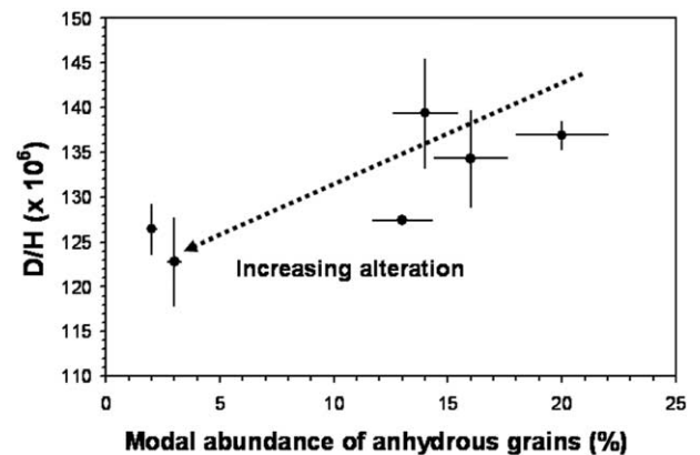
Fig. 6. D/H ratios plotted vs. the modal abundance of anhydrous grains for tochilinite-rich CCMs. This modal abundance is negatively correlated with the mineralogical alteration index defined for CM2 chondrites by Browning et al. (1996). Error bars on the modal abundance have been estimated to be 10% relative. The dashed line is a hand-drawn best fit curve.
