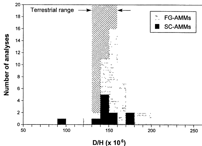
FIG. 7. Distribution of the D/H ratios in the fine-grained unmetelted Antarctic micrometeorites (FG-AMMs) compared to that of the scoriaceous partially dehydrated/melted AMMs (SC-AMMs).
