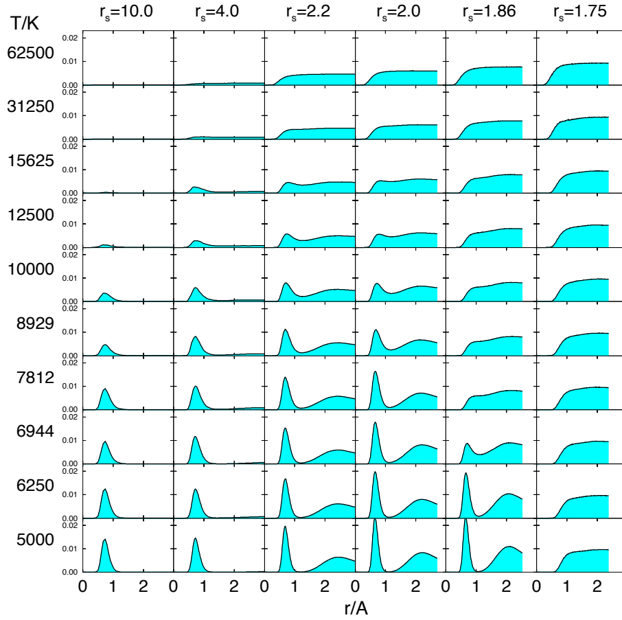
Figure 3.4: Proton-proton pair correlation function multiplied by the density n as a function of interparticle distance r (in Angstrom). The columns correspond, from left to right, to decreasing values of the density parameter r_s = a_0/a_e (increasing density \rho ; a_0 is Bohr's radius, a_e is the mean electronic distance). The rows correspond to temperatures increasing from 5000 K (bottom) to 62500 K (top). [Courtesy of B. Militzer; see also Militzer & Ceperley 2001].
