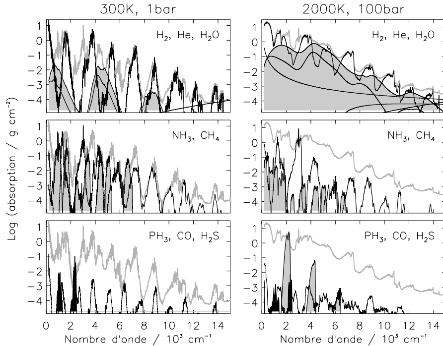
Figure 4.1: Absorption of a solar-composition mixture, at 300 K and 1 bar (left), and at 2000 K and 100 bar. Various contributions are shown. Top diagrams : \text{H}_2 - \text{H}_2 CIA (shaded) and \text{H}_2\text{O} (grey lines); Middle : \text{NH}_3 (shaded) and \text{CH}_4 (grey lines); Bottom : \text{PH}_3 (shaded, left diagram), \text{CO} (shaded, right diagram) and \text{H}_2\text{S} (grey).
