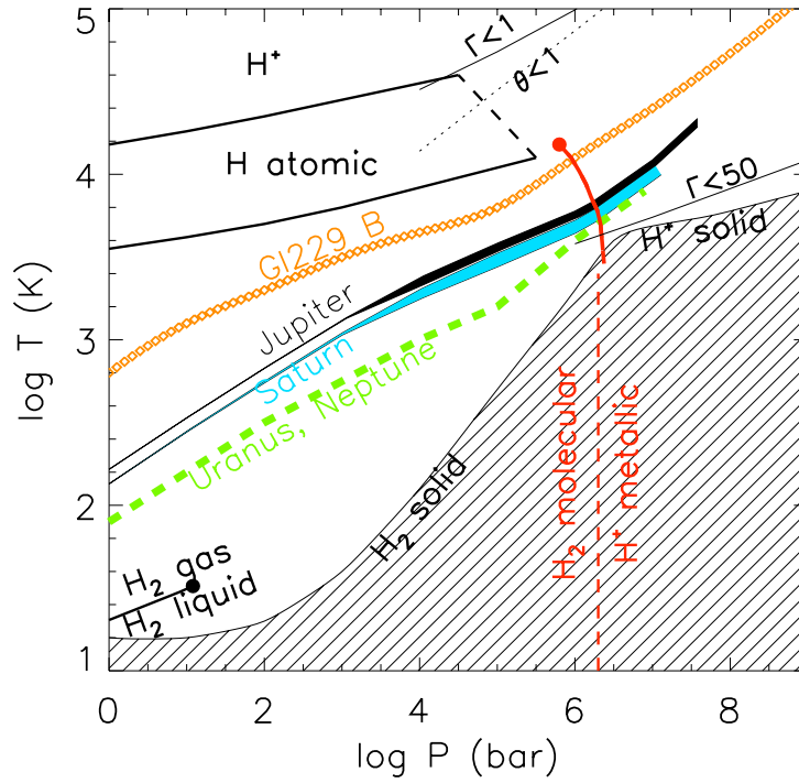
Figure 3.1: Phase diagram for hydrogen with the main phase transitions occurring in the fluid or gas phase. The temperature-pressure profiles for Jupiter, Saturn, Uranus, Neptune, and G1229B (assumed to be a 30 M_J brown dwarf) are shown. The plain, almost vertical line near 1 Mbar represents the Plasma Phase Transition (PPT) supposed to separate molecular from metallic hydrogen as computed by Saumon et al. (1995). The region in which hydrogen is predicted to be solid is represented as a dashed area. Lines showing the values of the parameters \theta and \Gamma (see text) are also shown.
