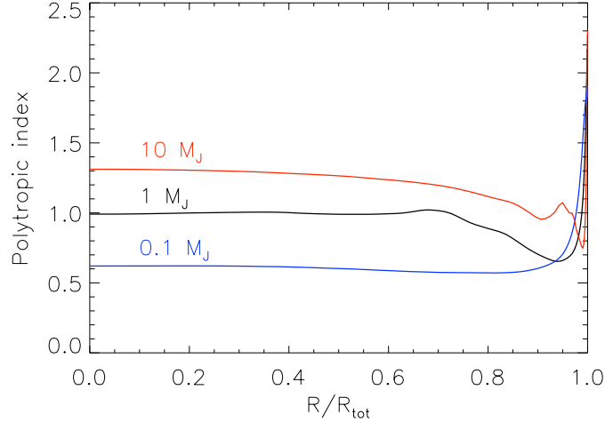
Figure 2.3: Polytropic index n (such that P \propto \rho^{1+1/n} ) as a function of internal radius, for 0.1, 1 and 10 M_{\text{J}} isolated planets of solar composition after 10 Ga of evolution.
