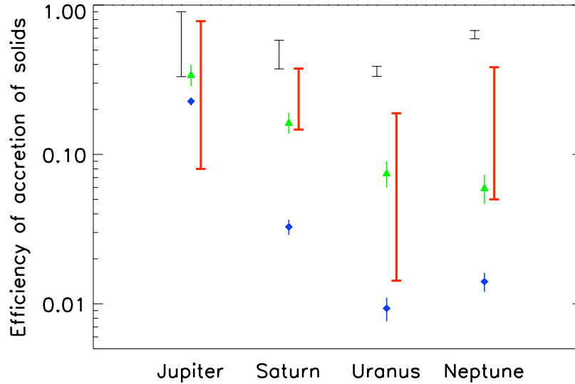
Figure 5.6: Accretion efficiencies required to form the giant planets in the core accretion scenario. The accretion efficiency for a given planet is defined as the quantity of heavy elements that had to impact the planet divided by the total amount of heavy elements within the annulus that extends halfway to the next planet. The upper left error bar for each planets corresponds to the ratio between the total mass of heavy elements and the quantity of solids required by Pollack et al. (1996). The lower thick error bars account for core formation by runaway growth, and include only heavy elements in the envelopes. Diamonds are accretion probabilities in the Jupiter, Saturn, Uranus and Neptune regions, respectively, as calculated in the standard case. Triangles correspond to the reduced-mass case (see text). [From Guillot & Gladman 2000].
