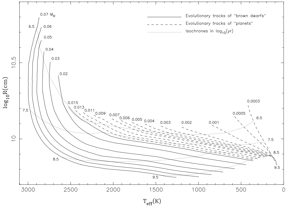
Figure 6.5: \log_{10} radius (in cm) vs. effective temperature ( T_{\text{eff}} , in K), with T_{\text{eff}} decreasing to the right. The isochrones are the almost horizontal lines and are labeled in \log_{10} yr. In all cases, the radius decreases with time. Initially, for the more massive brown dwarfs, the effective temperature is roughly constant, or slightly increasing, before decreasing inexorably at later times. [From Burrows et al. (1997)].
