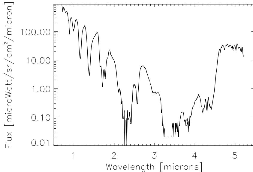
Figure 1.2: Flux emitted by a Jupiter hot spot as seen by the Galileo orbiter with NIMS. [From Carlson et al. 1996; Courtesy of P. Drossart].
