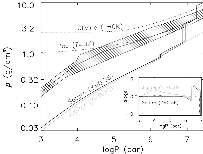
Figure 5.1: Density profiles in models of Jupiter (gray line) and Saturn (continuous lines: adiabatic i -EOS and PPT-EOS models; dashed: non-adiabatic i -EOS model). Upper curves (dashed and dot-dashed) are T = 0 K density profiles for water ice and olivine (from Thompson 1990). The dashed region represents the assumed uncertainty on the EOS for heavy elements ( \rho_Z(P, T) ). Within this region, the continuous line corresponds to our “preferred” profile for \rho_Z . Inset : Differences of the decimal logarithm of the Saturn density profiles with the same profile using the i -EOS and an adiabatic structure (plain and dotted lines). The gray line corresponds to the same difference but for a PPT-EOS non-adiabatic Jupiter model. (From Guillot 1999a).
