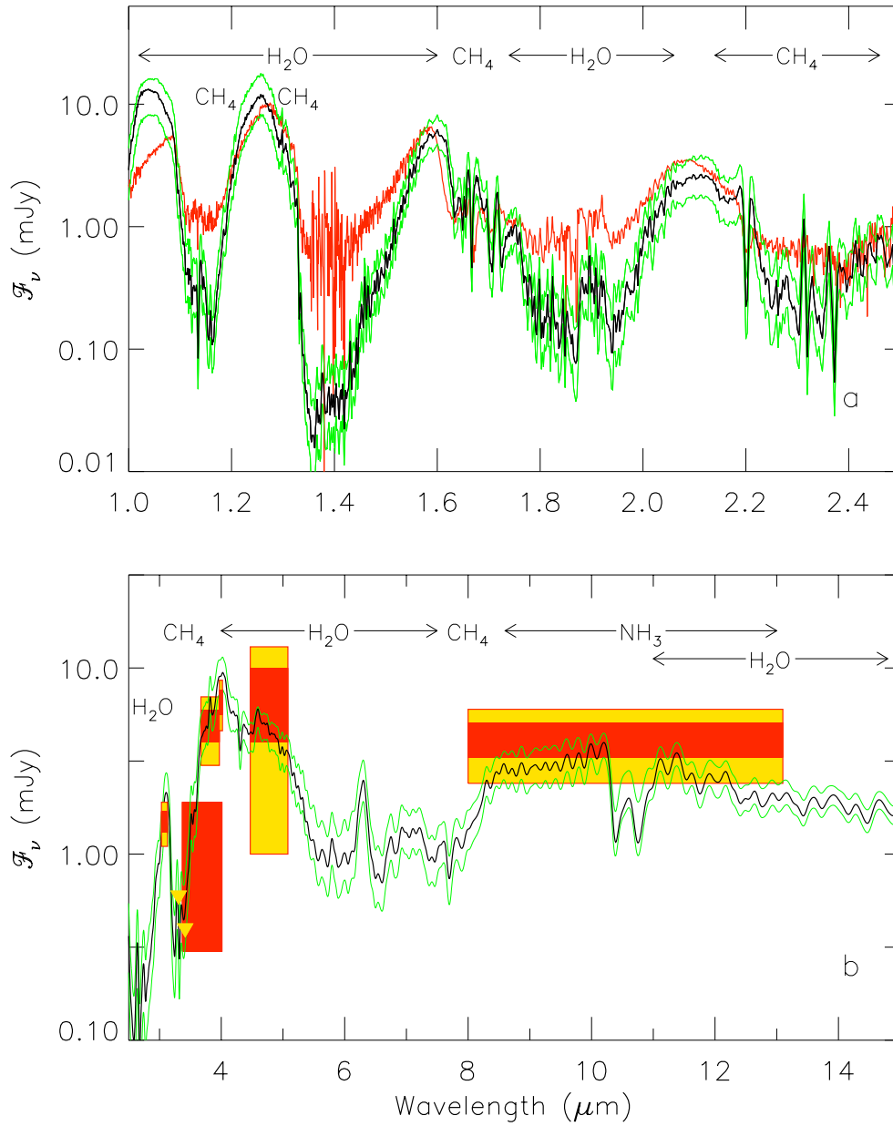
Figure 7.1: Synthetic spectra for (bottom to top) T_{\text{eff}} = 890 \text{ K}, 960 \text{ K}, 1030 \text{ K} and g = 10^5 \text{ cm s}^{-2} together with observed data from Geballe et al. (1996) (top panel) and photometric broadband measurements also from Geballe et al. (bottom panel). In both panels, spectral intervals are labeled with the molecules primarily responsible for the opacity in that interval. [From Marley et al. 1996].
