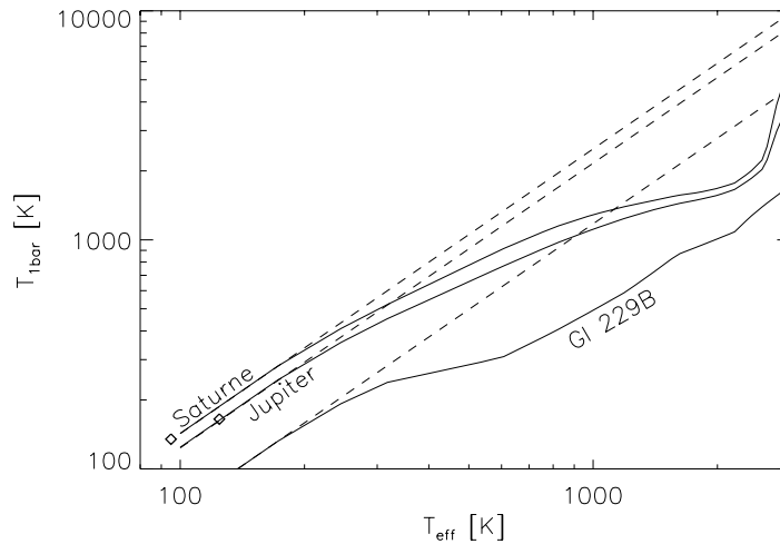
Figure 2.1: Comparison of the boundary condition obtained from Eq.(2.7) (dashed) to a grey atmosphere from Saumon et al. (1996) (plain), in the case of Saturn ( g \approx 1100 \text{ cm s}^{-2} ), Jupiter ( g \approx 2600 \text{ cm s}^{-2} ) and Gl229B ( g \approx 10^5 \text{ cm s}^{-2} ).
