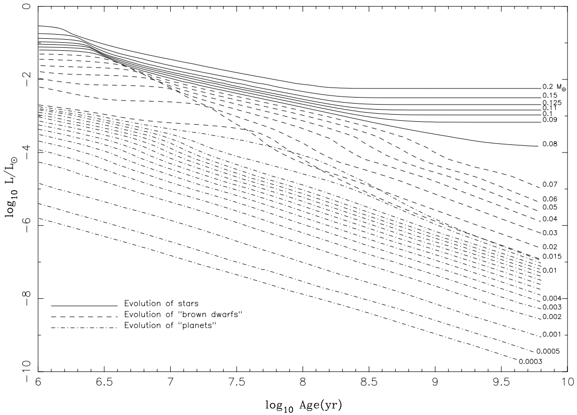
Figure 6.4: Evolution of the luminosity (in L_{\odot} ) of solar-metallicity M dwarfs and substellar objects vs. time (in yr) after formation. The stars, "brown dwarfs" and "planets" are shown as solid, dashed, and dot-dashed curves, respectively. In this figure, we arbitrarily designate as "brown dwarfs" those objects that burn deuterium, while we designate those that do not as "planets." The masses (in M_{\odot} ) label most of the curves, with the lowest three corresponding to the mass of Saturn, half the mass of Jupiter, and the mass of Jupiter. [From Burrows et al. (1997)].
