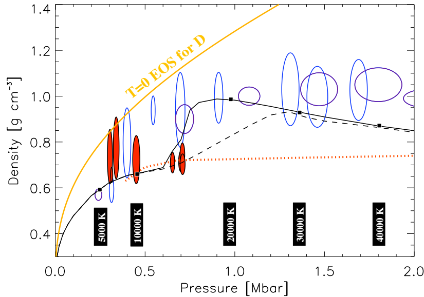
Figure 3.2: Comparison of experimental data and theoretical Hugoniot for deuterium (densities are twice larger than expected for hydrogen at any given pressure). Empty ellipses correspond to data points from laser compression (Collins et al. 1998). Filled ellipses were obtained by magnetic compression (Knudson et al. 2001). Theoretical calculations are represented by lines. They are respectively: the “PPT” (solid) and “interpolated” (dashed) Saumon-Chabrier equations of state (Saumon, Chabrier & Van Horn 1995), and a Path Integral Monte Carlo EOS (Militzer & Ceperley 2000). The solid line to the left shows the T=0 equation of state for D_2 as determined by an exp-6 potential fit to diamond-anvil cell measurements (Hemley et al. 1990). The temperatures along the Hugoniot have been calculated using the PPT-EOS. [From Guillot et al. 2003].
