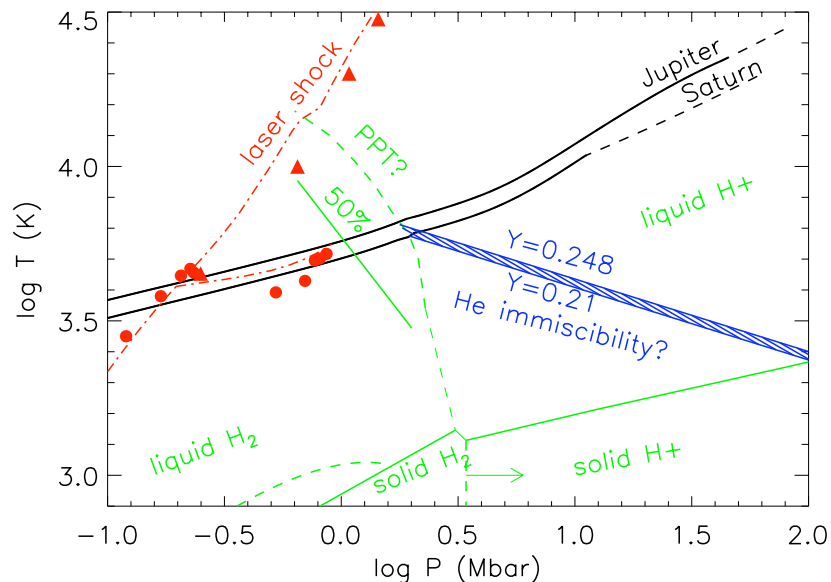
Figure 3.3: Hydrogen phase diagram, with interior profiles of present-day Jupiter and Saturn overlaid, and with some experimental data shown. The boundary between liquid H 2 and solid H 2 is somewhat uncertain in the Mbar pressure range (2 estimates are shown), but is not relevant to Jupiter. The laser shock measurements of Collins et al. (2001) and the gas-gun measurements of Holmes et al. (1995) are shown as triangles and filled circles in the upper left-hand corner, respectively. Single- and double-shock hydrogen Hugoniot calculated by Saumon et al. (2000) are shown as dot-dashed lines in the same region of the plot. The solid line labeled “50%” shows where 50% of molecular dissociation is obtained in the model of Ross (1998).
