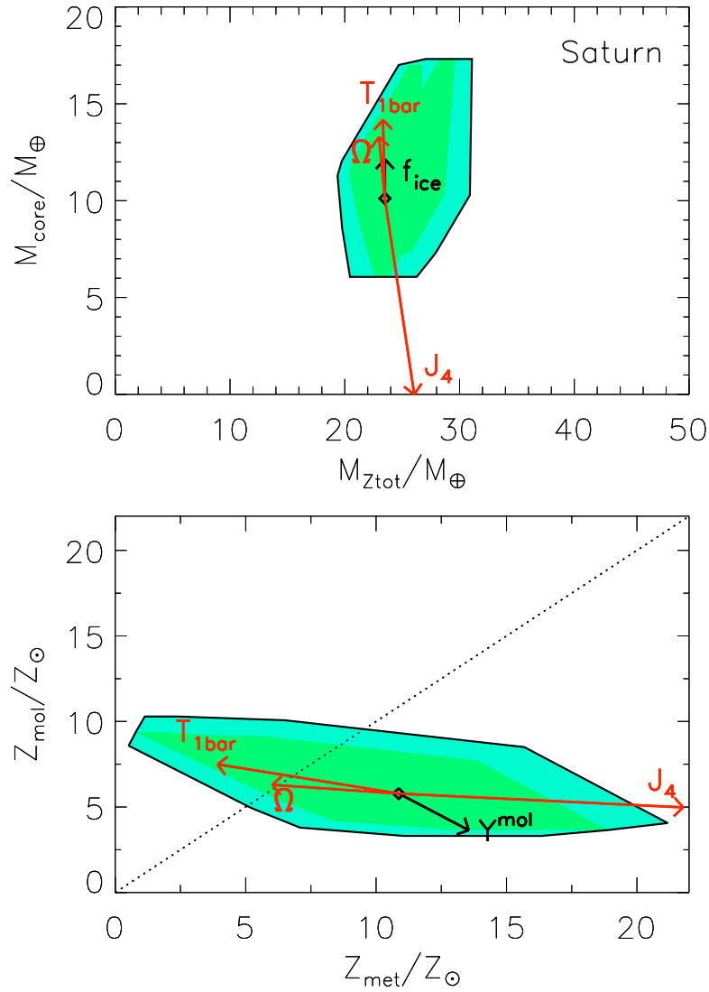
Figure 5.3: Same as fig. 5.2 in the case of Saturn. The solutions for the PPT and interpolated hydrogen EOSs are very similar and are thus not highlighted. The arrow labeled T_{1\text{bar}} corresponds to an increase of Saturn's 1 bar temperature from 135 to 145 K. The arrow labeled Y^{\text{mol}} corresponds to an increase of the helium mass mixing ratio from 0.16 to 0.21. [Adapted from Guillot 1999a].
