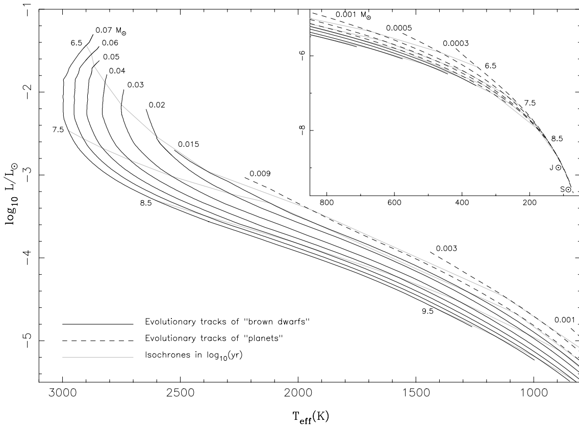
Figure 6.6: H-R diagram: luminosity (in L_{\odot} ) versus T_{\text{eff}} (in K) for various masses labeled on the figure in M_{\odot} . Due to the large range in luminosity and the near degeneracy of the tracks of substellar objects at late stages of evolution, it is not possible to represent with adequate detail the whole H-R diagram as one figure. Accordingly, the low-temperature and low-luminosity tail of the H-R diagram is shown in the inset. The observed positions of Jupiter and Saturn are labeled as points “J” and “S,” respectively. [From Burrows et al. (1997)].
