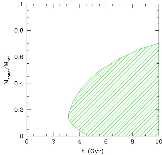
Figure 6.3: Evolution of the conductive core M_{\text{cond}}/M_{\text{tot}} (shaded area) as a function of time for a 0.06 M_{\odot} brown dwarf. [From Chabrier et al. (2000b)].
