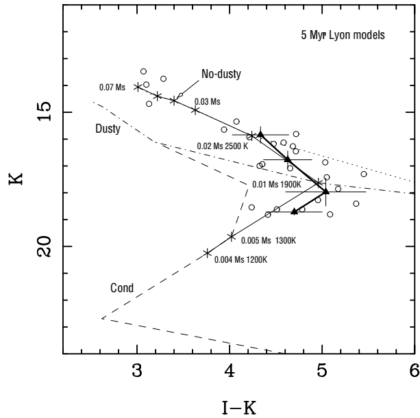
Figure 7.3: K vs I-K color-magnitude diagram. Empty circles are substellar members in \sigma Orionis. The thick solid line and filled triangles represent the mean locus of the \sigma Orionis objects. The 5 Myr isochrones from Chabrier et al. (2000b) are displayed (Nextgen no-dusty models—dotted line, Dusty models—dot-dashed line, and Cond models—dashed line). The thin solid line with asterisks is a best-guess isochrone that combines the models. [From Martín et al. 2001].
