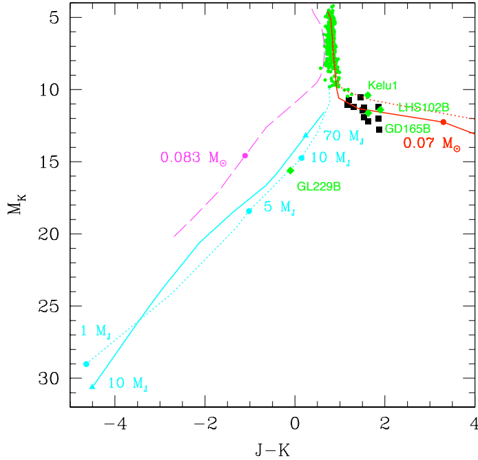
Figure 7.2: M_K vs (J-K) diagram for different ages and metallicities: [\text{Fe}/\text{H}]=0 for 10^8 yr (dotted lines) and 5 \times 10^9 yr (solid lines); [\text{Fe}/\text{H}]=-2 , t=10 Gyr (dashed line). The red curves on the right correspond to the DUSTY models for [\text{Fe}/\text{H}]=0 . The blue curves on the left correspond to the COND models for [\text{Fe}/\text{H}]=0 . Filled circles and triangles on the isochrones indicate masses either in M_\odot or M_J ( 1 M_J \approx 10^{-3} M_\odot ). [From Chabrier & Baraffe 2000].
