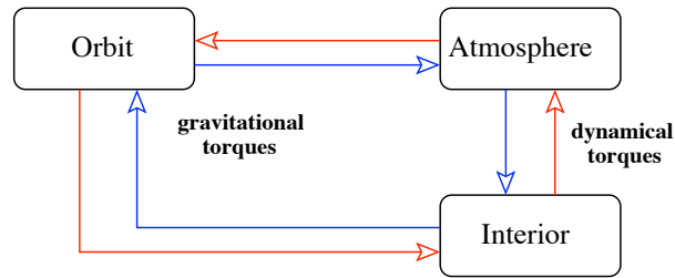
Figure 8.5: Angular momentum flow between orbit, interior, and atmosphere for a Pegasi planet in steady state. Arrows indicate flow of prograde angular momentum (i.e., that with the same sign as the orbital angular momentum) for two cases: Anticlockwise : Gravitational torque on atmosphere is retrograde (i.e., adds westward angular momentum to atmosphere). For torque balance, the gravitational torque on the interior must be prograde (i.e., eastward). These gravitational torques must be balanced by fluid-dynamical torques that transport retrograde angular momentum from atmosphere to interior. Clockwise : Gravitational torque on atmosphere is prograde, implying a retrograde torque on the interior and downward transport of prograde angular momentum from atmosphere to interior. Atmosphere will superrotate if gravitational torques push atmosphere away from synchronous (as on Venus). It will subrotate if gravitational torques synchronize the atmosphere (e.g., gravity-wave resonance).
