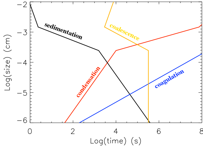
Figure 7.6: Time scales for grain growth and sedimentation at the basis of an “iron-cloud” in a brown dwarf of T_{\text{eff}} = 2000 \text{ K} , g = 3 \times 10^5 \text{ cm s}^{-2} . [Brown dwarf model: courtesy of F. Allard; timescales from Rossow 1978].
