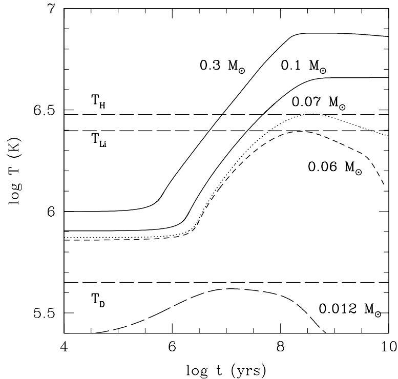
Figure 6.7: Central temperature as a function of age for different masses. T_H , T_{Li} and T_D indicate the hydrogen, lithium and deuterium burning temperatures, respectively. [From Chabrier & Baraffe 2000].
