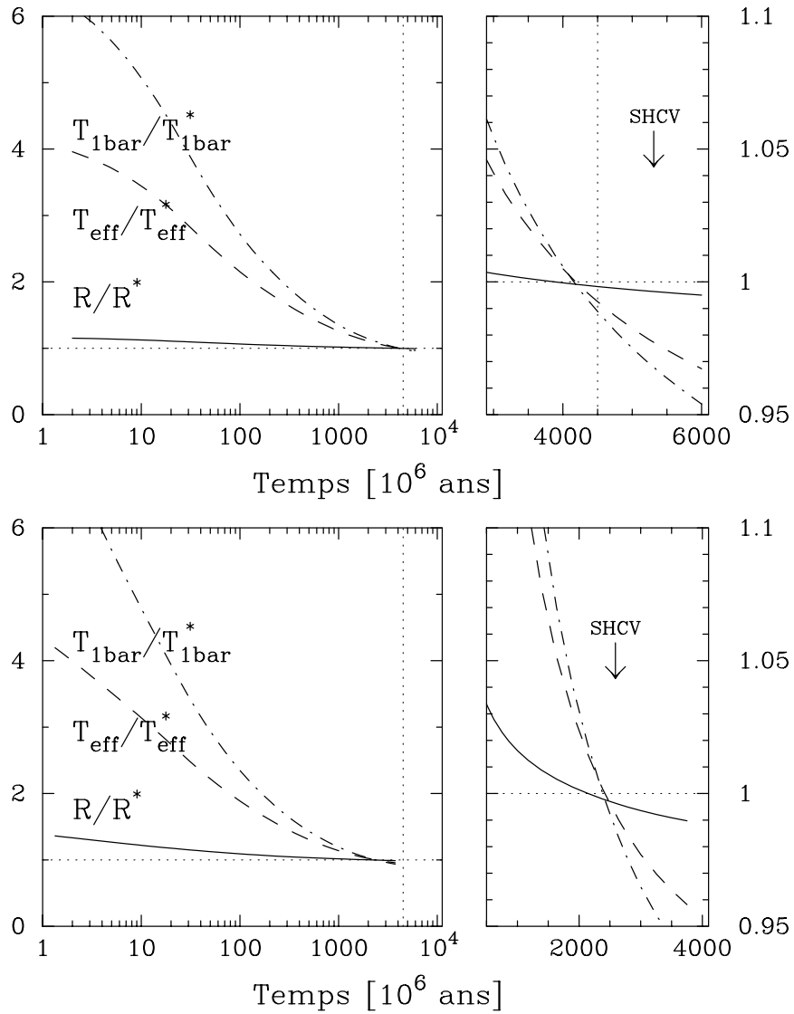
Figure 6.2: Contraction and cooling a non-adiabatic models of Jupiter (top) and Saturn (bottom) (opacities not including alkali metals). The 1 bar temperature, effective temperature and mean radius are represented as a function of time. All these quantities are normalized to their present value, T_{1\text{bar}}^* , T_{\text{eff}}^* , and R^* . The right figure is an enlargement of the left one. Note that time is then represented linearly. The vertical dotted line indicates the age of the solar system. The arrow labeled SHCV corresponds to the age obtained for a fully convective model by Saumon et al. (1992). [From Guillot et al. (1995)].
