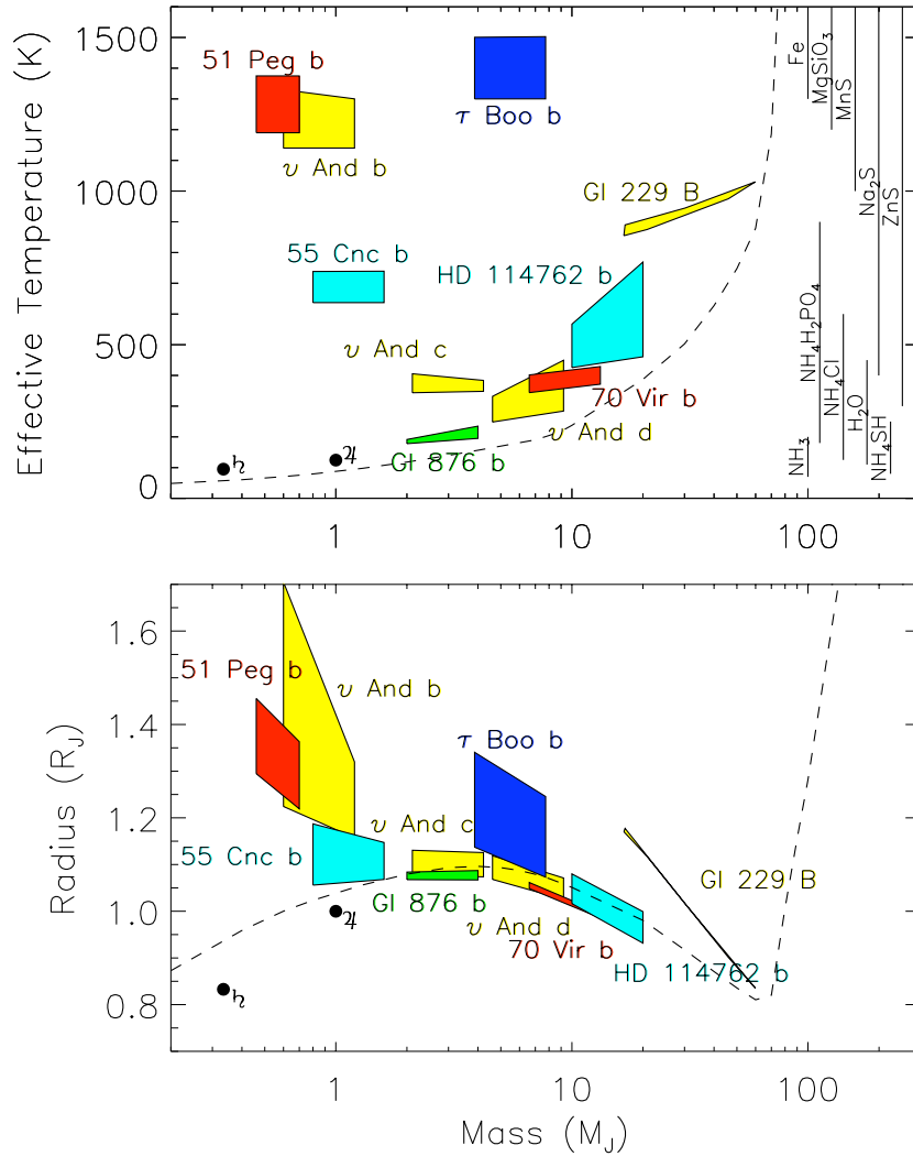
Figure 6.8: Predicted effective temperatures and radii (in units of Jupiter radii, R_J \sim 70,000 km) of some extrasolar planets and brown dwarfs, including reasonable uncertainties for their mass, albedo and age (see text). The dashed line is for isolated H-He ( Y = 0.25 ) objects after 10 Ga of evolution. The upper panel also shows potentially important chemical species expected to condense near the photosphere in the indicated range of effective temperatures. [From Guillot (1999b)]
