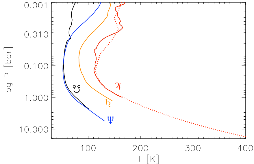
Figure 1.1: Atmospheric temperatures as a function of pressure for Jupiter, Saturn, Uranus and Neptune, as obtained from Voyager radio-occultation experiments (see Lindal 1992). The dotted line corresponds to the temperature profile retrieved by the Galileo probe, down to 22 bar and a temperature of 428 K (Seiff et al. 1998).
