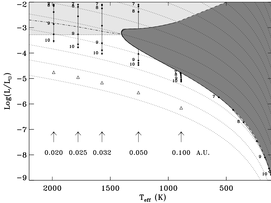
Figure 8.2: Hertzsprung–Russell diagram for 1 M_J planets orbiting at 0.02, 0.025, 0.032, 0.05 and 0.1 AU from a solar-type star, assuming a Bond albedo of 0.35. Arrows indicate the corresponding equilibrium effective temperature ( T_0 ). A Jupiter model is also shown, the diamond in the bottom right-hand corner corresponding to the present-day effective temperature and luminosity of the planet. Evolutionary tracks for planets of solar composition are indicated by lines connecting dots which are equally spaced in \log(\text{time}) . The numbers 7, 8, 9 and 10 are the common logarithms of the planet’s age. Zero-temperature models for 1 M_J planets made of olivine ( \text{Mg}_2\text{SiO}_4 ) are indicated by triangles. The Hayashi forbidden region, which is enclosed by the evolutionary track of the fully convective model, is shown in dark gray (see text). Models in the light gray region have radii above the Roche limit (and therefore are tidally disrupted by the star). The region where classical Jeans escape becomes significant is bounded by the dash-dotted line. Lines of constant radius are indicated by dotted curves. These correspond, from bottom to top, to radii (in units of \bar{R}_J ) in multiples of 2, starting at 1/4 . [From Guillot et al. (1996)]
