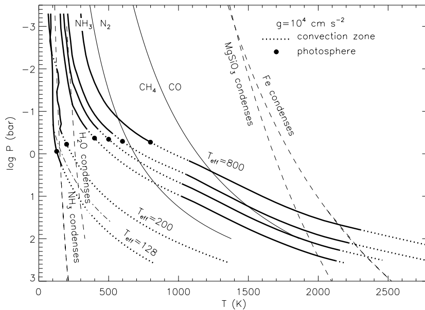
Figure 7.5: Atmospheric pressure–temperature profiles for non-irradiated substellar atmospheres with surface gravity fixed at 10^4 \text{ cm s}^{-2} and T_{\text{eff}} = 800, 600, 500, 400, 200, and 128 \text{ K} . Note that the inner radiative zones disappear in the presence of alkali metals (not accounted for in the calculation). [From Burrows et al. (1997)]
