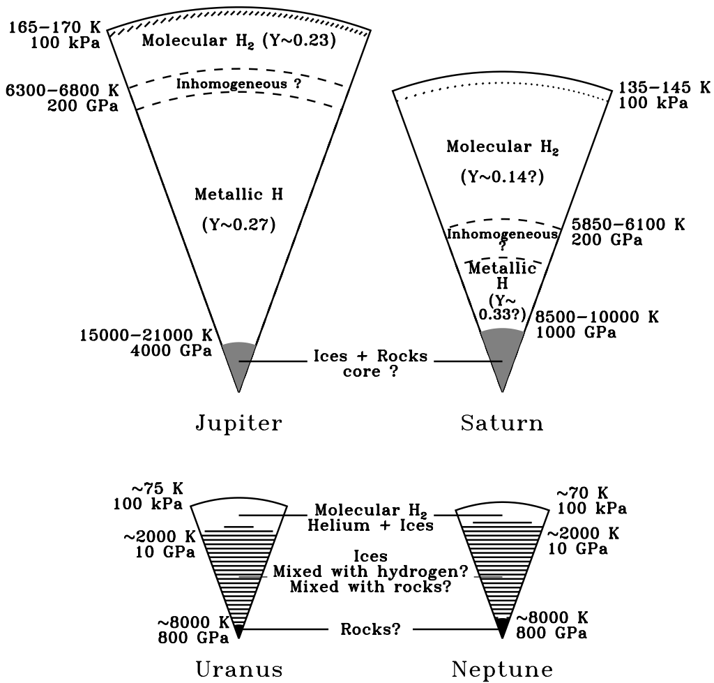
Figure 5.4: Schematic representation of the interiors of Jupiter, Saturn, Uranus and Neptune. The hashed region indicate a possible radiative zone (in Jupiter, it corresponds to P \sim 0.15 to 0.6 GPa, T \sim 1450 to 1900 K, and R \sim 0.990 to 0.984 R_J ; in Saturn, it is located around P \sim 0.5 GPa, T \sim 1700 K, R \sim 0.965 R_S ). The radiative zone are expected to disappear in the presence of alkali metals. The range of temperatures for Jupiter and Saturn is for models neglecting the presence of the inhomogeneous region. Helium mass mixing ratios Y are indicated. In the case of Saturn, it is assumed that Y/(X+Y) = 0.16 in the molecular region. The size of the central rock and ice cores of Jupiter and Saturn is very uncertain. Two representative models of Uranus and Neptune are shown, but their actual interior structure may be significantly different (see text). [From Guillot 1999b].
