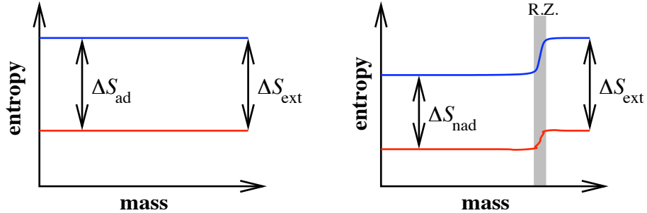
Figure 6.1: Example of evolution of the specific entropy profile in the purely adiabatic case (left) and in the presence of a radiative zone (gray area in the right hand side figure). In each case, the entropy is represented in function of the mass variable at two different times. Here the entropy jump is chosen to decrease with time. In spite of the fact that the initial surface conditions are the same in the two cases for the initial and final models, the mean entropy difference is smaller in the non-adiabatic case than in the adiabatic one ( \Delta S_{\text{nad}} < \Delta S_{\text{ad}} ). In this example, the cooling of the non-adiabatic model is faster (see text).
