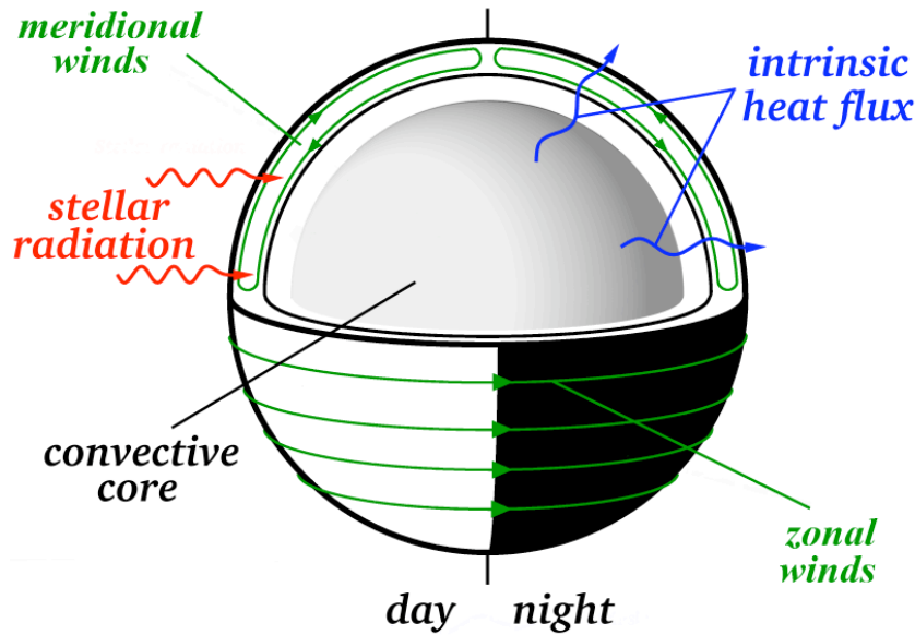
Figure 8.7: Conjectured dynamical structure of Pegasi planets: At pressures larger than 100–800 bar, the intrinsic heat flux must be transported by convection. The convective core is at or near synchronous rotation with the star and has small latitudinal and longitudinal temperature variations. At lower pressures a radiative envelope is present. The top part of the atmosphere is penetrated by the stellar light on the day side. The spatial variation in insolation should drive winds that transport heat from the day side to the night side. [From Guillot (2001); Showman & Guillot (2002)].
