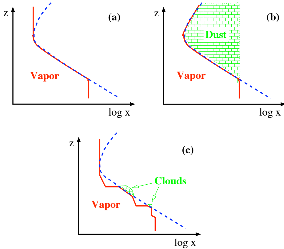
Figure 7.4: Possible abundance profiles x of a condensing species in a substellar or planetary atmosphere (plain lines). The dashed lines corresponds to the saturation profiles. Three cases are: (a) clear atmosphere (immediate “rainout” of condensates); (b) dusty atmosphere (no “rainout”); (c) a possibly more realistic situation (see text).
