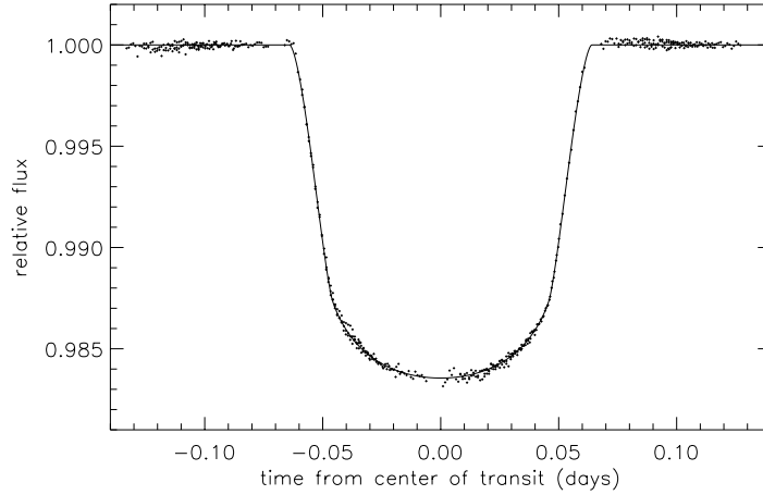
Figure 8.1: Phased light curve of four planetary transits across the star HD209458 observed with the HST. The orbital period of the planet is 3.52474 days. [Figure from Brown et al. (2001a)]
