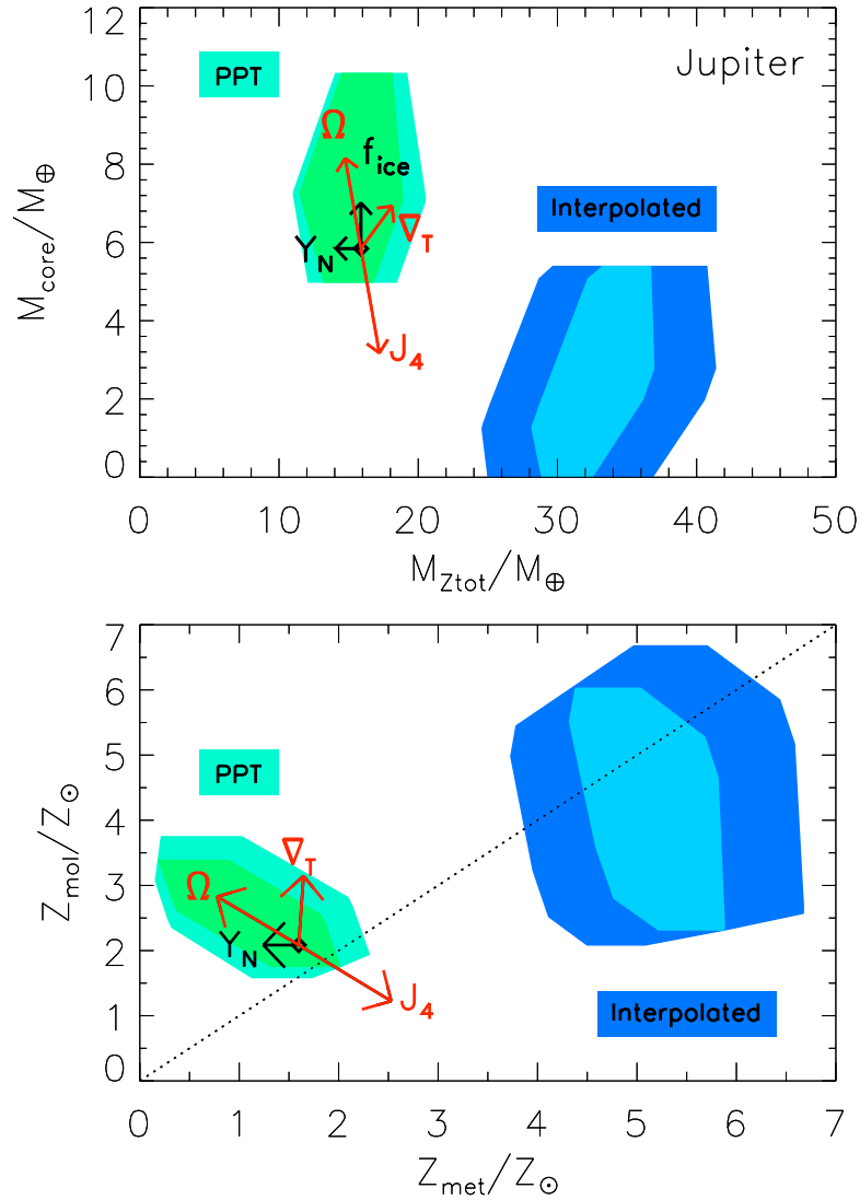
Figure 5.2: Constraints on Jupiter’s interior structure. The upper panel shows values of the core mass ( M_{\text{core}} ) and total mass of heavy elements ( M_{Z_{\text{tot}}} ) of models matching all available observational constraints. The lower panel shows the mass mixing ratio of heavy elements of the molecular ( Z_{\text{mol}} ) and metallic ( Z_{\text{met}} ) regions, in solar units ( Z_{\odot} = 0.0192 ). The two different regions correspond to different EOSs for hydrogen (see text). Arrows indicate the direction and magnitude of the assumed uncertainties, if J_4 or Y_{\text{proto}} are increased by 1\sigma , rotation is assumed to be solid (“ \Omega ”), the core is assumed to be composed of ices only (“ f_{\text{ice}} ”) and if Jupiter’s interior becomes fully adiabatic (“ \nabla_T ”). The dashed line in the lower panel indicates a homogeneous abundance of heavy elements ( Z_{\text{mol}} = Z_{\text{met}} ). [Adapted from Guillot 1999a].
