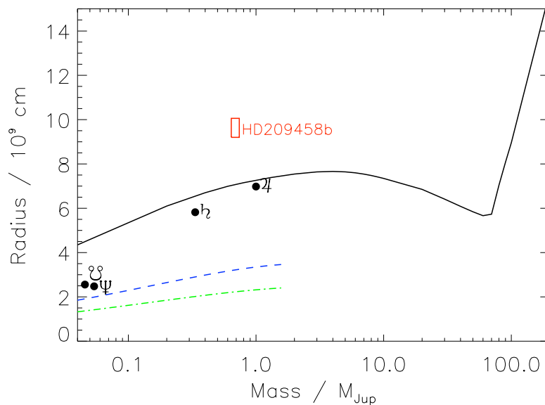
Figure 2.2: Radius versus mass for hydrogen-helium planets ( Y=0.25 ) after 10 Ga of evolution (plain line). An approximate mass-radius relation for zero-temperature water and olivine planets is shown as dashed and dash-dotted lines, respectively (Courtesy of W.B. Hubbard). The observed values for Uranus, Neptune, Saturn and Jupiter, as well as that for the Pegasi planet HD209458b are indicated.
