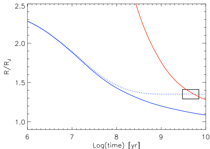
Figure 8.4: Evolution of the radius of a solar composition 0.69 M_J planet with T_{\bullet} = 1400 K. The plain lines correspond to standard evolution models with the “hot” (larger radii) and “cold” (smaller radii) atmospheric boundary condition. The dotted curve corresponds to an evolution calculation with dissipation, and in the “cold” case. The box indicates inferred radii and ages of HD209458b. [Adapted from Guillot & Showman (2002)]
