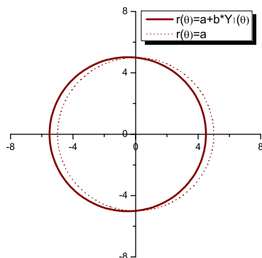
(b) \bar{r}(\theta) \propto Y_1(\theta)
