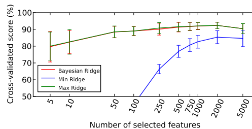
Figure 3.12: Cross-validated regression score (4-fold) obtained for different numbers of voxels, for Bayesian Ridge (red), and the minimum (blue) and maximum (green) values obtained by the classical Ridge among the different values of the regularization parameter (see Fig. 3.8).
