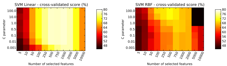
Figure 3.3: SVC - Average cross-validated classification score (4-fold) obtained for different numbers of voxels and different values of C for a linear kernel (left) and an RBF kernel (right).
