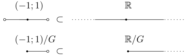
Figure 3.2: Two local suborbit spaces.
