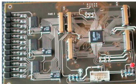
Figure 1: The basic board with a 2096VE device (front and back side)
