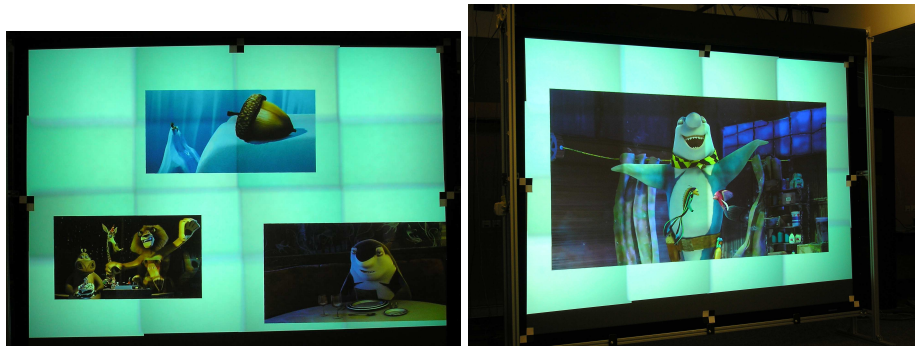
Figure 5.5: Rendering HDTV videos on a 16 projector display wall using Mplayer and FlowVR Render.
