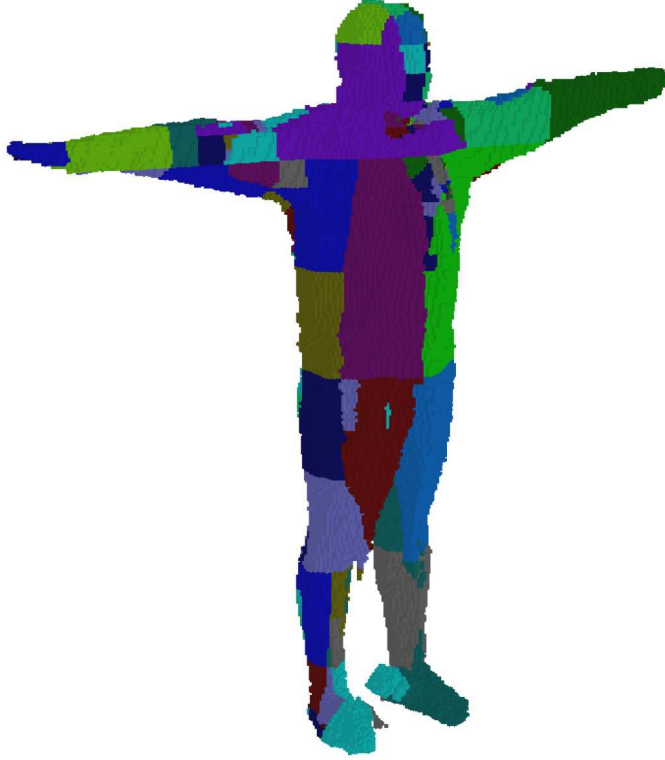
Figure 7.3: Parallel octree carving with 16 cores (max depth of 8). Voxels are color-coded according to the core that produced them. It shows the good spatial locality of work stealing.
