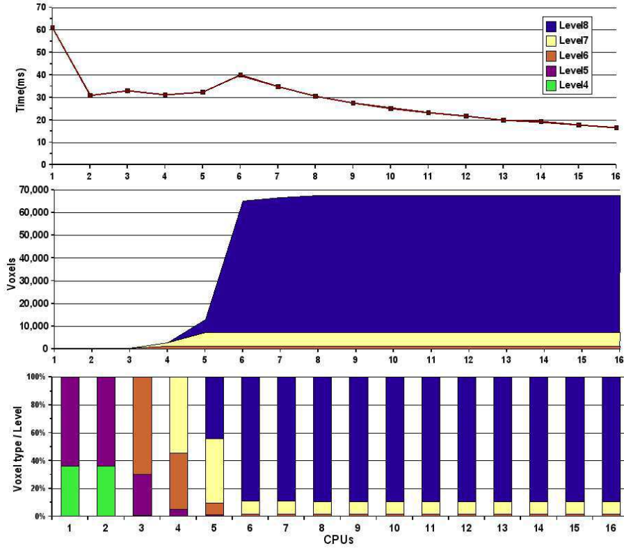
Figure 7.4: Performance result of octree carving with a 30 ms time limit. (Top) Execution time, (Middle) number of voxels computed, (Down) percentage of voxel per depth level (max depth level set to 8).
