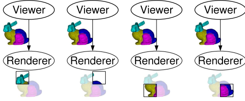
Figure 3: Replication: Viewer application is replicated on each rendering node. If the application is non-determinist then communications will be necessary to keep copies synchronized.
