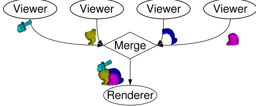
Figure 4: Parallel scene description: To distribute the load in viewers, several viewers can describe parts of the scene which are then merged together.
