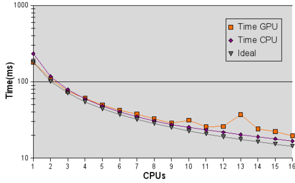
Figure 10: GPGPU x Pure CPU.
