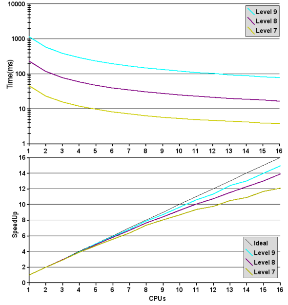
Figure 6: Execution time and speed up for Ben.
