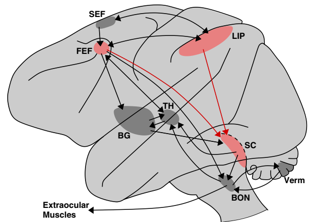
Fig. 1 Premotor and motor circuitry shared by saccade and smooth pursuit movement (Macaque monkey). BG basal ganglia, BON brain-stem oculomotor nuclei, FEF frontal eye fields, LIP lateral bank of the intraparietal sulcus, SC superior colliculus, SEF supplementary eye fields, TH thalamus, Verm cerebellar vermis. In light red regions using retinotopic reference frames to encode visual, memory and motor activity, refer to text for more details. Adapted from (Krauzlis 2004) (color in online)
