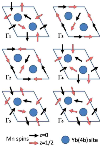
FIG. 7. (Color online) Symmetry allowed Mn spin orders in hexagonal RMnO 3 . In YbMnO 3 , \Gamma_2 or \Gamma_4 IR yield the best fit to experiment.
