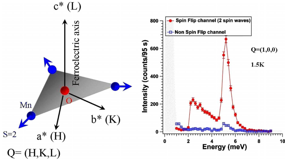
FIG. 1. (Color online) (a) Sketch of the Mn-O plane with the ordered spins ( S=2 ) of the Mn ions as observed in the Néel state in hexagonal multiferroics. The reciprocal vectors ( a^* , b^* , and c^* ) are also depicted. The momentum transfer Q=(H,K,L) is expressed in units of reciprocal wave vectors. (b) Typical measurement of “normal” spin waves at the wave vector Q=(100) . The peaks appear only in the SF channel (red open circles) whereas the signal measured in the NSF channel (blue open squares) corresponds to the leak of intensity from the SF channel. Note that the asymmetric profile of the first spin-wave peak could be due to resolution effects.
