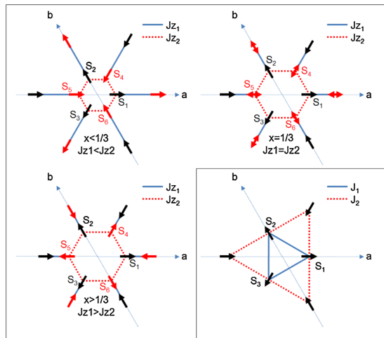
FIG. 1 (color online). Sketch of the hexagonal MnO planes with out-of-plane exchange paths J_{z1} (between \vec{S}_4 and \vec{S}_3 ) and J_{z2} (between \vec{S}_4 and \vec{S}_1 as well as \vec{S}_4 and \vec{S}_2 ). Black (red) arrows depict the positions of the Mn spins within z = 0 ( z = 1/2 ) Mn planes. \vec{S}_1 , \vec{S}_2 , and \vec{S}_3 are located at (x, 0, 0) , (0, x, 0) , and (-x, -x, 0) , respectively, while \vec{S}_4 , \vec{S}_5 , and \vec{S}_6 are at (x, x, 1/2) , (1-x, 0, 1/2) , and (0, 1-x, 1/2) , respectively. Double arrows are used when several spin orientations can be stabilized. Inset: Sketch of the hexagonal MnO plane with in-plane exchange paths J_1 and J_2 .
