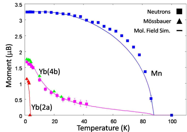
FIG. 8. (Color online) Observed Mn, \text{Yb}(4b) , and \text{Yb}(2a) moments from NPD and Mössbauer measurements (dots) versus temperature. The solid lines correspond to the molecular-field calculation.
