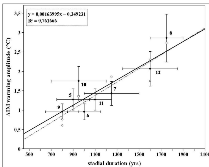
Figure P5: Correlation between the amplitude of surface temperature increases for each AIM event and the duration of the accompanying stadial in Greenland. Black dots and line correspond to TALDICE data and open diamonds and dash line to EDML data (Epica Community members, 2006). Numbers correspond to the AIM events
