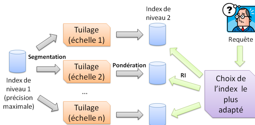
FIGURE 5.5 – Indexation multi-échelles
