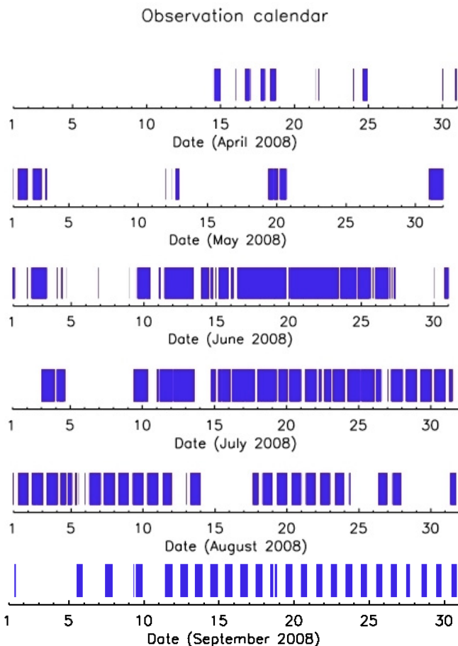
Fig. 12. ASTEP South observation calendar for the 2008 campaign. April and May were mainly dedicated to solving technical problems. Continuous observations started mid-June with very few interruptions until the end of the winter.
