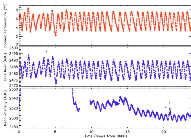
Fig. 10. Camera temperature, bias level and image intensity on July 11. The camera temperature varies between +4 and +8\text{ }^{\circ}\text{C} with a period of one hour and affects the bias level and the image intensity to about 10 ADU.
