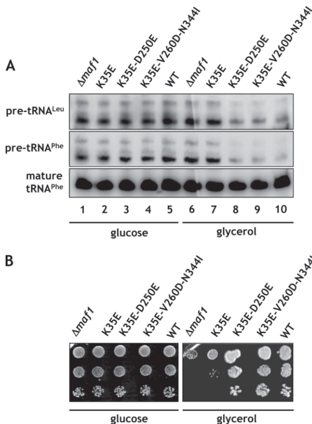
FIGURE 4. Regulation of pol III transcription and growth is impaired by the K35E mutation in region encoding A domain and restored by second-site suppressor mutations in BC domain of MAF1. maf1 \Delta , maf1 -K35E, maf1 -K35E/D250E, and maf1 -K35E/V260D/N344I mutants and isogenic wild type strain YPH500 (WT) were used. A , cells were grown to exponential phase in glucose medium (YPD) at 30°C, then transferred to glycerol medium (YPGly) and incubated at 37°C for 1.5 h. Total RNA isolated from cells was tested by Northern blotting with pre-tRNA Leu and tRNA Phe probes. B , 10-fold serial dilutions of cells grown to exponential phase in glucose medium were plated on glucose medium (YPD) and incubated at 30°C or on glycerol medium (YPGly) and incubated at 37°C for 2–3 days.
