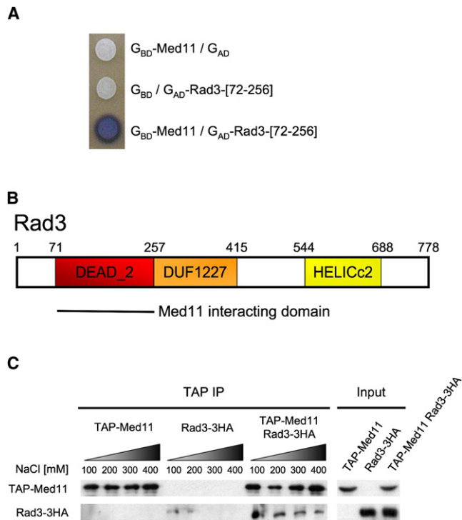
Figure 1. Med11 Mediator Subunit Interacts with Rad3 Helicase of TFIIH
