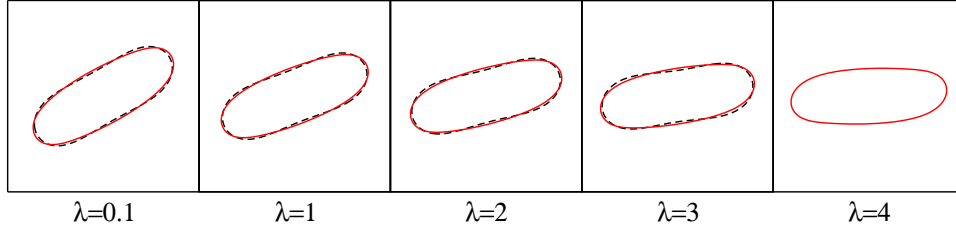
Figure 6.10: Stationary contours of tank-treading vesicles ( \alpha = 0.7 ) at C_a = 10.0 (solid line) compared with the corresponding ones at C_a = 1.0 (dashed line) for different values of the viscosity ratio \lambda (for \lambda = 4.0 and C_a = 1.0 there is no tank-treading solution).
