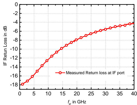
Figure 4.31: Return loss measured at one of the baseband outputs
