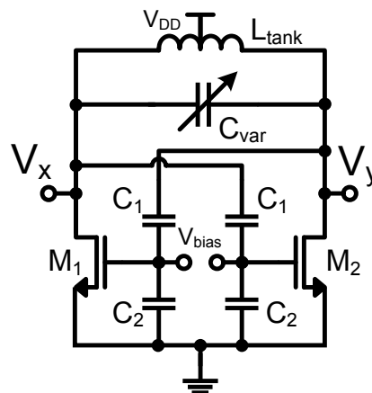
Figure 4.11: Schematic illustrating the principle of the common-source Colpitts VCO
