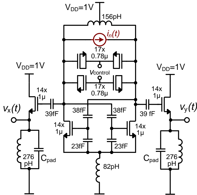
Figure 8.19: Schematic of the 65 nm CMOS 60 GHz VCO
