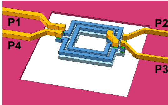
Figure 3.30: Three-dimensional layout of a single-coil stacked transformer, occupying metal layers M6 and M7 for the coils and M5 and alucap for over- and underpasses. The vertical dimensions are three times magnified.
