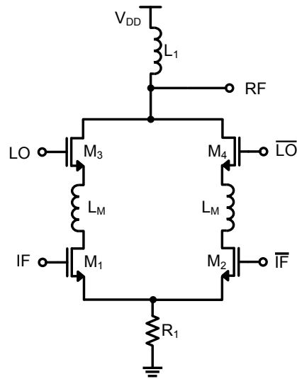
Figure 4.38: Schematic of the dual-gate mixer core (without biasing)
