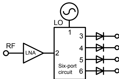
Figure 2.16: Block diagram of six-port receiver front-end
