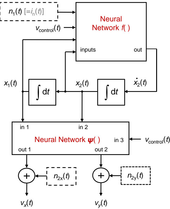
Figure 8.7: Block diagram of the oscillator model for the case of differential outputs ( v_x(t), v_y(t) ) and one control input ( v_{\text{control}}(t) ). Blocks with dashed margin represent white Gaussian noise generators.
