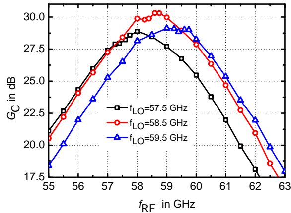
Figure 5.6: Measured power conversion gain versus RF frequency at different LO frequencies
