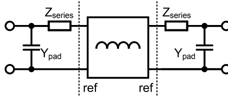
Figure 3.45: Lumped element de-embedding assumes a parallel admittance and a series impedance as error two-port
