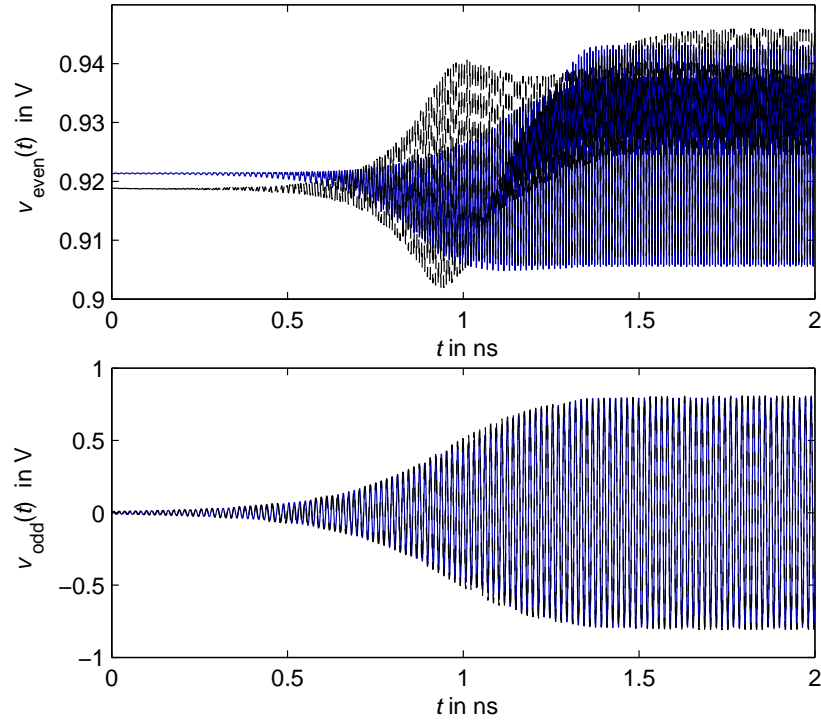
Figure 8.16: Output of the VHDL-AMS model (dotted black line) versus ADS simulation results (solid blue line) in even mode ( v_{\text{even}}(t) = (v_x(t) + v_y)/2(t) ) and odd mode ( v_{\text{odd}}(t) = (v_y(t) - v_x(t))/2 ).
