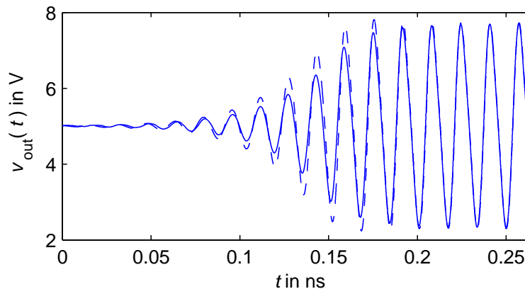
Figure 8.14: Startup of the single-ended oscillator: VHDL-AMS model (solid line) versus ADS response (dashed line)
