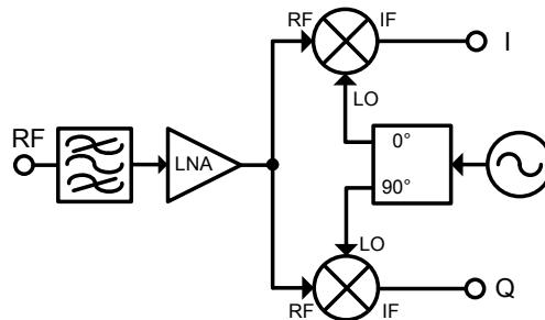
Figure 2.12: Principle of a direct conversion receiver creating the quadrature phases at the mixer's LO input by a 90^\circ phase shifter
