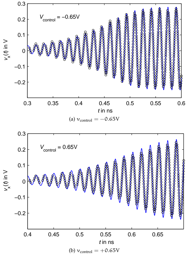
Figure 8.22: Startup waveform at output x of the VCO. VHDL-AMS model (markers) versus SPECTRE-simulation (solid line).
