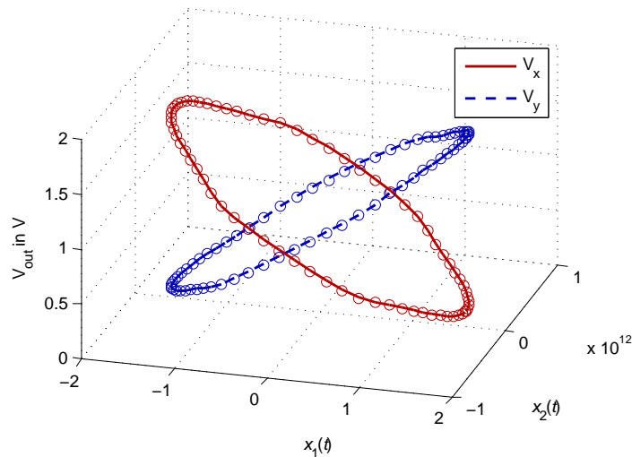
Figure 8.13: Mapping from the states x_1 and x_2 of the system to its output voltages (function \psi(\cdot) ). dashed and solid line: original output, circles: output of neural network.
