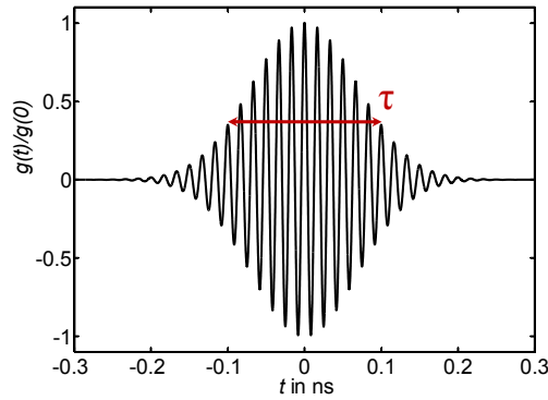
Figure 2.1: Gaussian Impulse for the 60 GHz band
