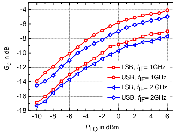
Figure 4.43: Conversion Gain versus LO power for two IF frequencies with f_{LO} = 62 GHz and P_{IF} = -20 dBm.
