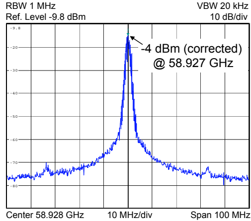
Figure 4.19: Measured oscillator output spectrum at 58.92 GHz ( V_{\text{control}}=0 V)
