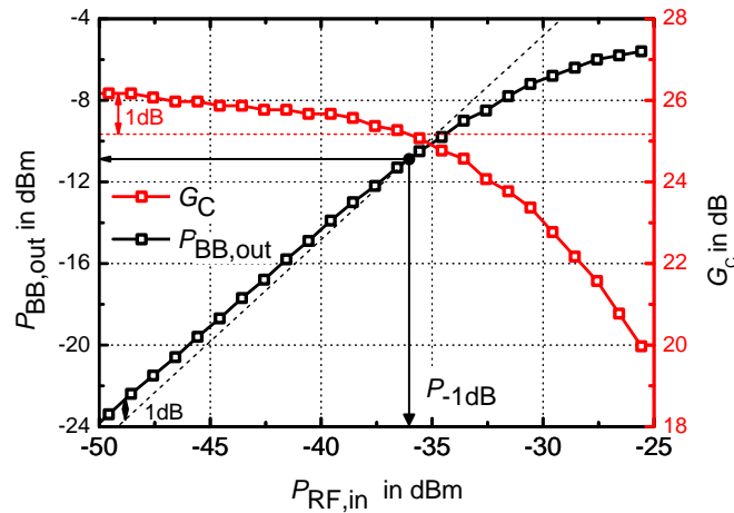
Figure 5.9: Linearity measurement for f_{LO} = 59 GHz and f_{RF} = 60 GHz
