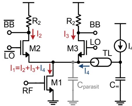
Figure 4.26: Current bleeding as proposed by B. Razavi [67]
