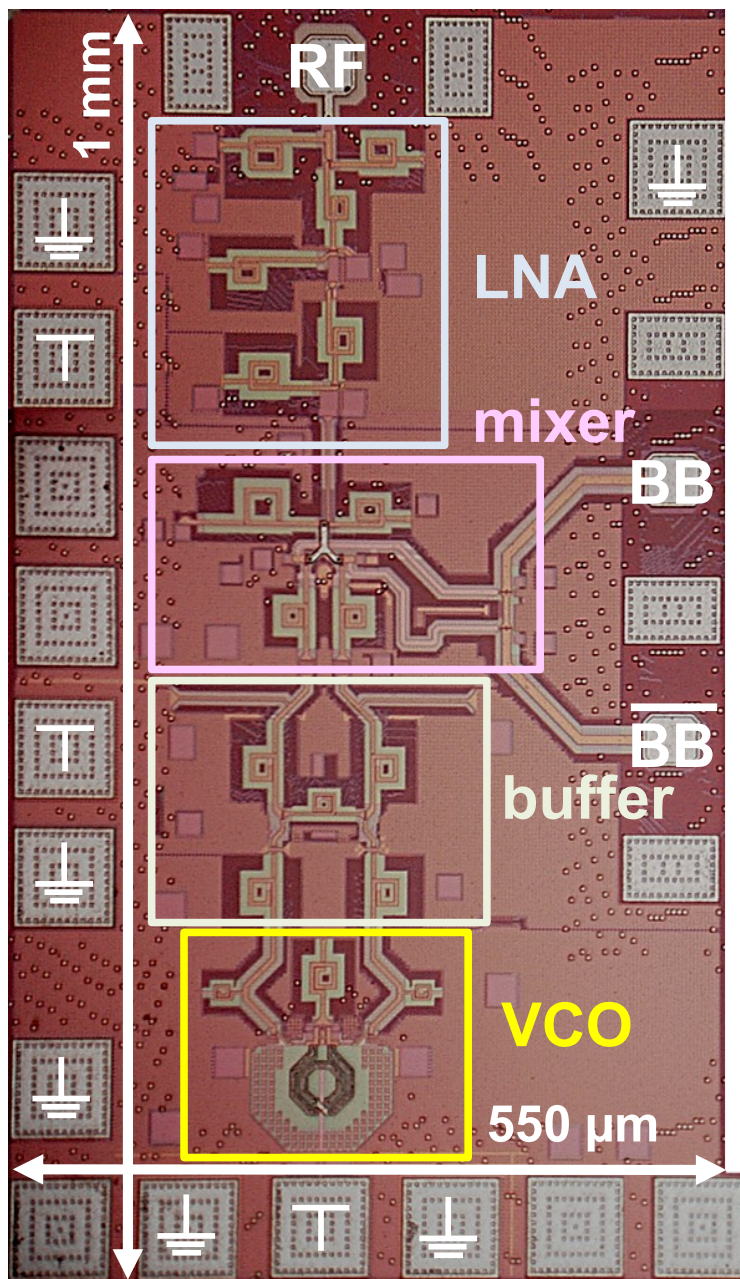
Figure 5.2: Microphotograph of the fabricated CMOS receiver front-end
