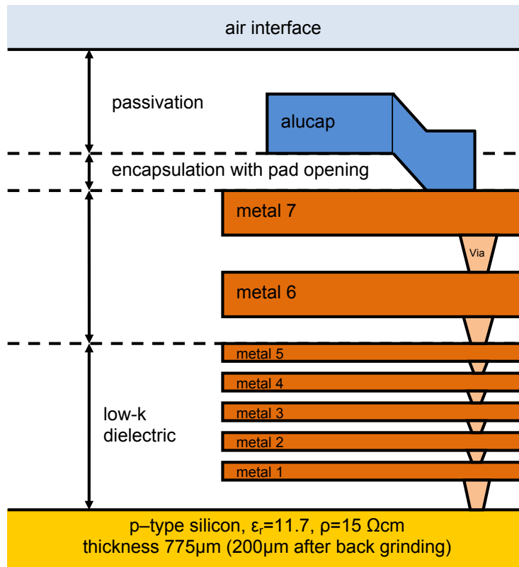
Figure 3.1: Simplified metal-backend of the 65 nm CMOS technology
