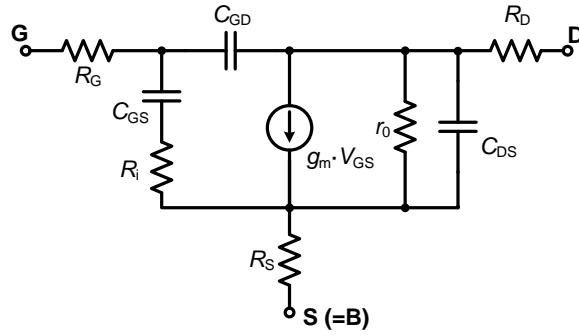
Figure 3.7: Typical small signal equivalent circuit model of a MOSFET valid up to mm-waves.
