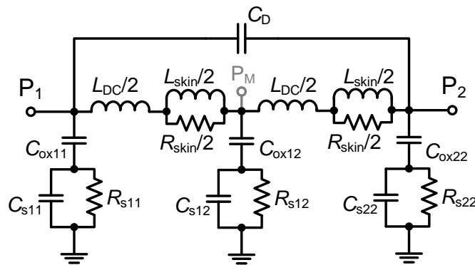
Figure 3.28: 2- \pi equivalent circuit for spiral inductors
