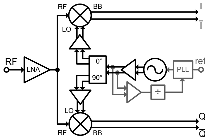
Figure 2.20: Block diagram of adopted direct conversion receiver
