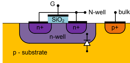
Figure 3.16: Principle structure of an accumulation-mode MOS varactor in an n-well
