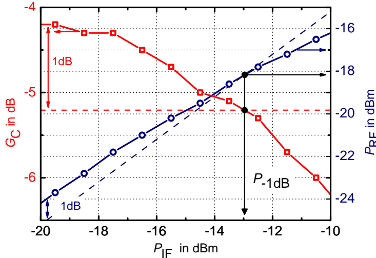
Figure 4.49: 1 dB Compression point measured at P_{LO}=6 dBm, f_{LO}=62 GHz, f_{IF}=1 GHz
