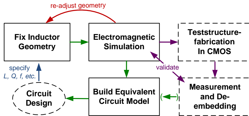
Figure 3.19: Design flow for mm-wave full-custom spiral inductors
