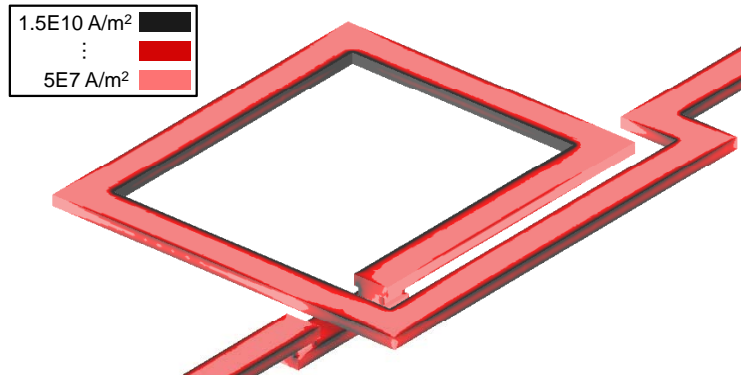
Figure 3.23: Plot of the current densities on the conductor surface. Plot obtained by HFSS-simulation, current density in logarithmic scale increasing to darker colors.
