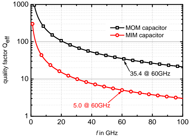
Figure 3.13: Comparison of the effective quality factors of MOM and MIM capacitances of value 100 fF. Plots obtained by DK simulation in accurate mode.
