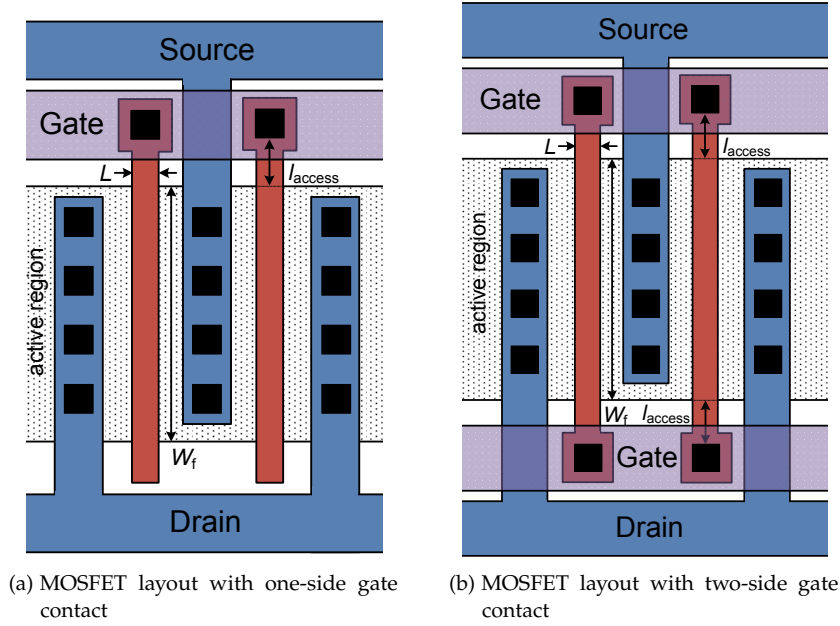
Figure 3.8: Illustration of MOSFET multifinger layouts using single or double gate contacts
