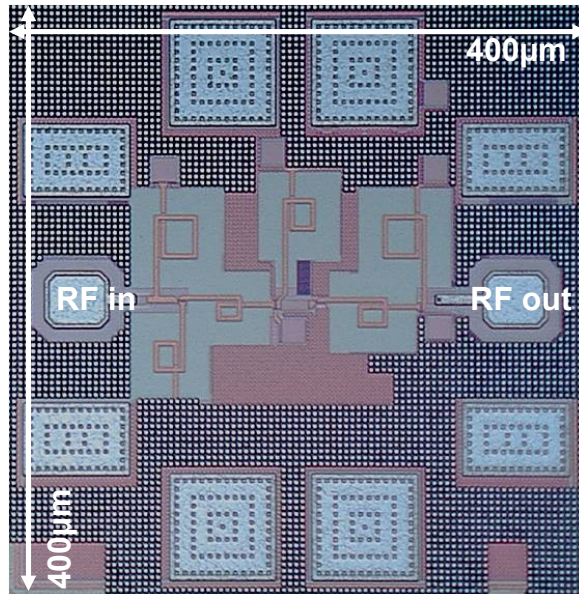
Figure 4.2: Photo of the fabricated LNA, circuit dimensions 400 \mu\text{m} \times 400 \mu\text{m} including pads.
