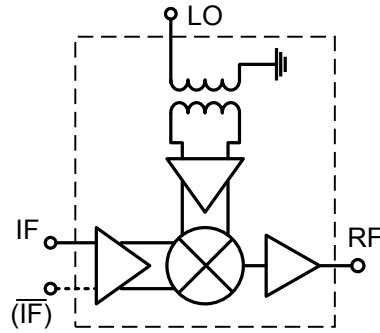
Figure 4.37: Mixer breakout comprising IF, LO and RF buffers and an LO transformer balun.
