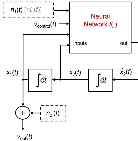
Figure 8.6: Block diagram of the oscillator model for the case of a single-ended output and one control input ( v_{\text{control}}(t) ). Blocks with dashed margin represent white Gaussian noise generators.
