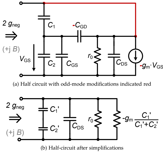
Figure 4.14: Equivalent half-circuit to calculate the negative admittance g_{\text{neg}}
