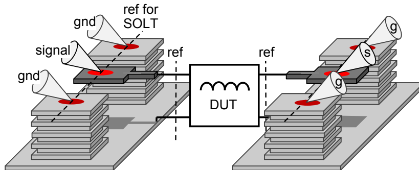
Figure 3.42: Perspective view of the test structure (with probes sitting on ground and signal pads) and illustration of the contact area
