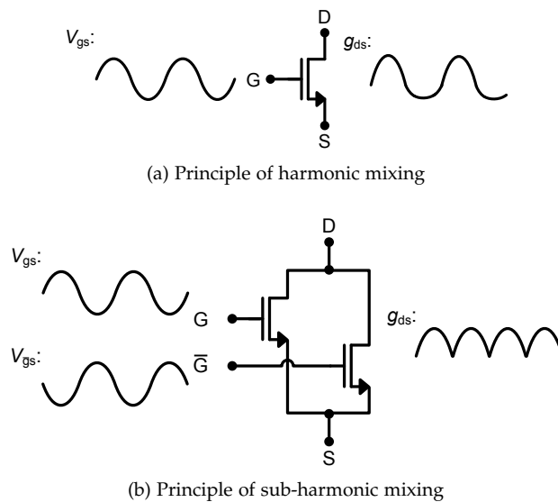
Figure 2.18: Harmonic versus sub-harmonic mixing principle
