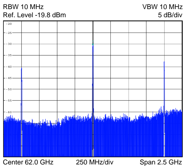
Figure 4.48: Uncorrected output spectrum using P_{LO,corr} = -5 dBm, P_{IF,corr} = -20.5 dBm
