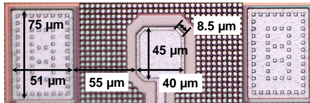
Figure 3.57: Die photo of G-S-G pad with annotated dimensions
