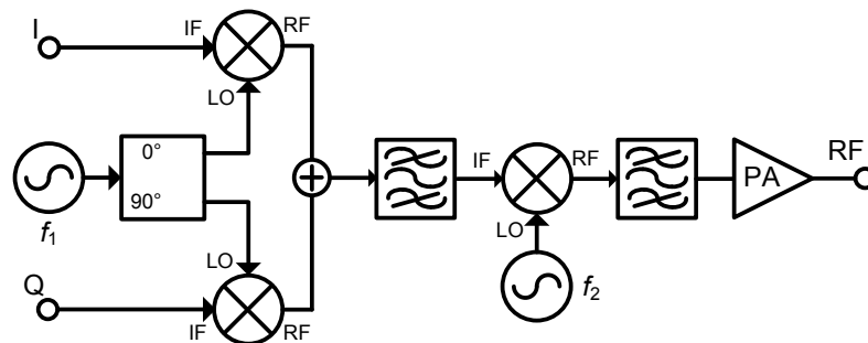
Figure 2.6: Two-step transmitter front-end using two different LO frequencies
