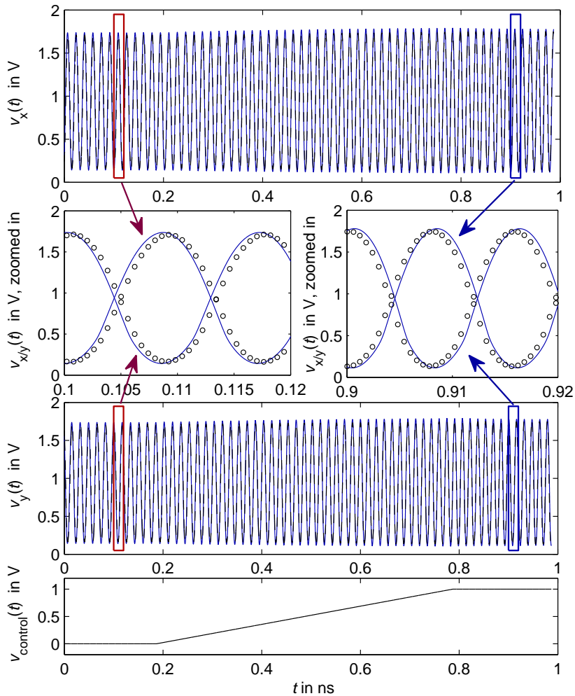
Figure 8.17: Output of the VHDL-AMS model (dotted black line or markers) versus ADS simulation results (solid blue line) for control voltage sweep
