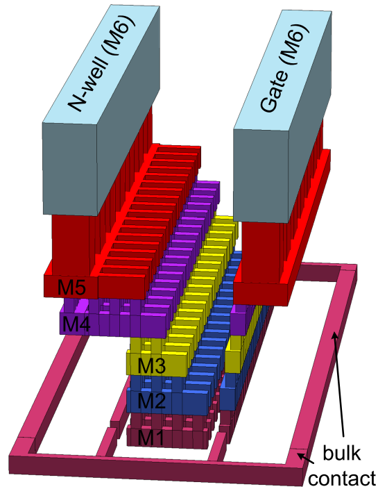
Figure 3.17: Metal back-end of the multifinger varactor layout based on a SVT GP device. Minimum-length fingers with W_f=0.78\ \mu\text{m} width are used.
