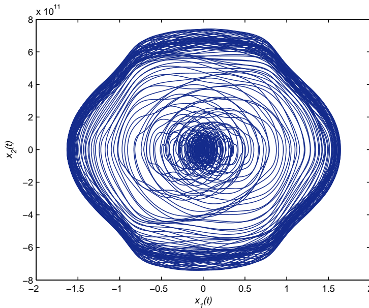
Figure 8.10: Dense trajectory due to the use of the artificial current source for injection of a current that influences the trajectory. The shown training-data originates from several start-ups.
