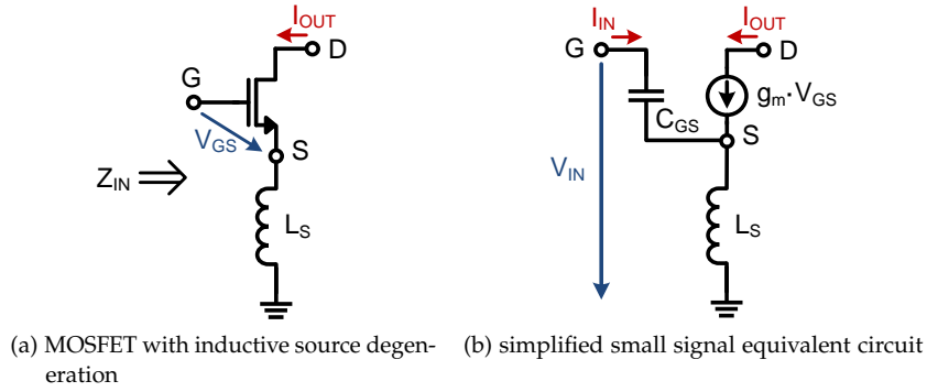
Figure 3.53: Inductive source generation
