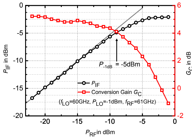
Figure 4.35: P_{IF} and G_C versus P_{RF} to illustrate nonlinearity and 1 dB compression point
