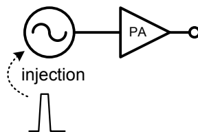
Figure 2.3: 60 GHz impulse transmitter based on a mm-wave oscillator with fast, impulse-triggered start-up
