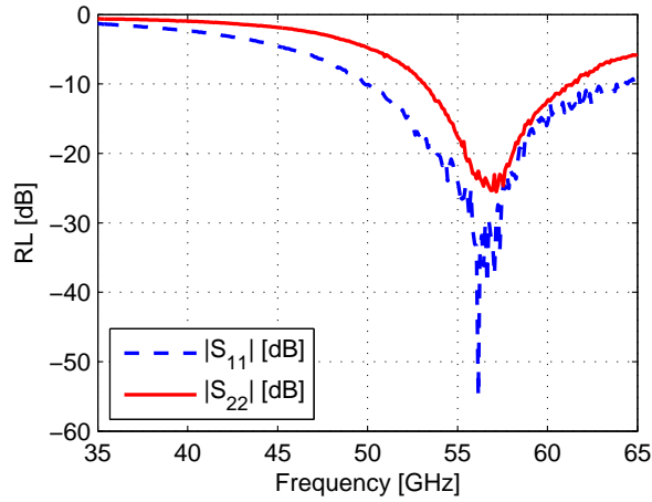
Figure 4.4: Return Loss (RL) measured at the input and output of the LNA biased at V_{DD}=1.5 V.
