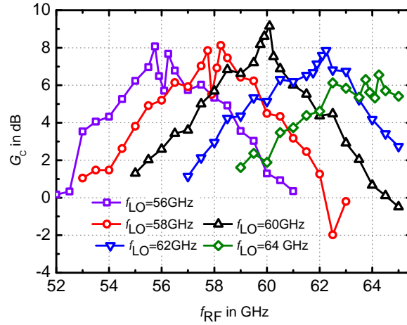
Figure 4.34: Conversion gain G_C versus f_{RF} for different LO frequencies. The IF is varying from 100 MHz to 5 GHz.
