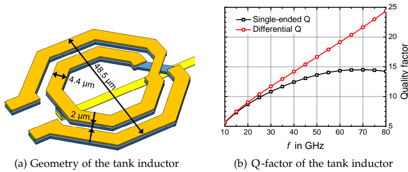
Figure 4.15: Characteristics of the VCO's 155 pH tank inductor
