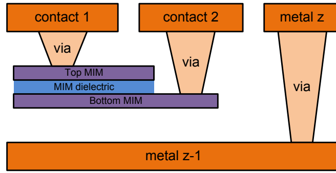
Figure 3.11: Illustration of a MIM capacitor inserted between two thick metal layers
