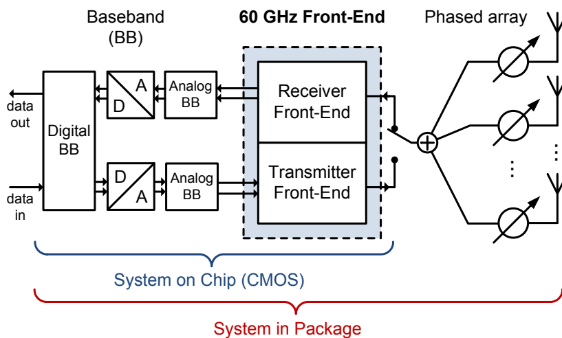
Figure 1.7: The proposed 60 GHz radio interface, whose 60 GHz transceiver front-end (highlighted in grey) is the subject of this thesis
