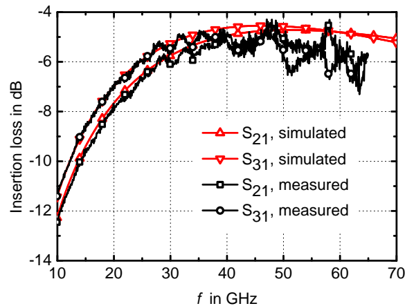
Figure 3.36: Simulated versus measured insertion loss from port P1 to ports P2 and P3, P1-P3 terminated in 50\ \Omega
