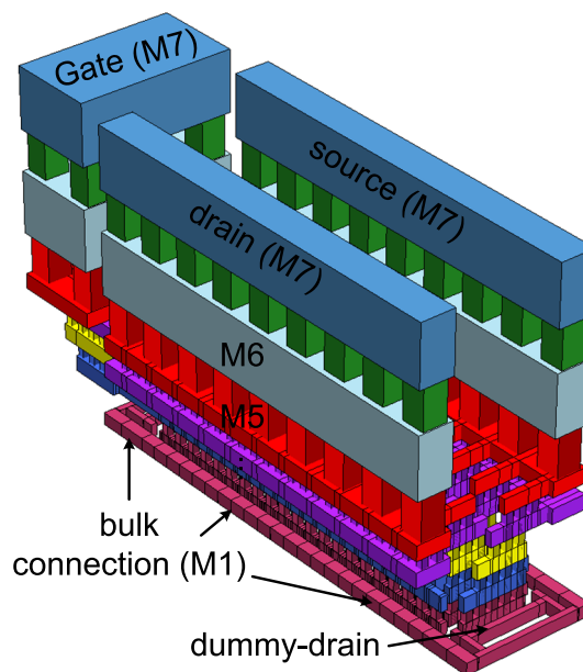
Figure 3.9: Three-dimensional view of the metal-backend of a multifinger transistor with 1\ \mu\text{m} finger width and 10 effective gates.
