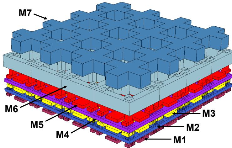
Figure 3.56: Shielding and supply distribution network consisting of all copper metal layers (metal layer 7 for V_{DD} , metal layer 3 and 5 for bias voltages and interconnected metal layers 1,2,4 and 6 for ground).
