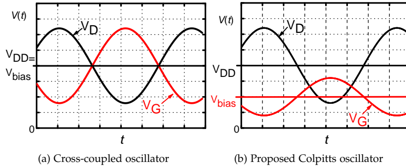
Figure 4.12: Illustration of oscillators' gate and drain voltage
