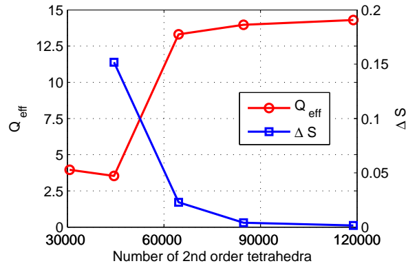
Figure 3.24: Convergence of the adaptive mesh refinement process in HFSS
