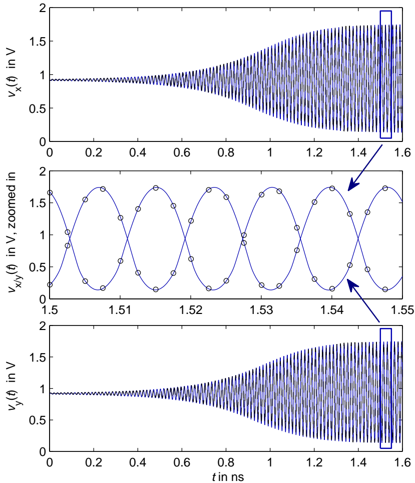
Figure 8.15: Output of the VHDL-AMS model (dotted black line or markers) versus ADS simulation results (solid blue line) for v_{\text{control}} = 0.5 \text{ V}
