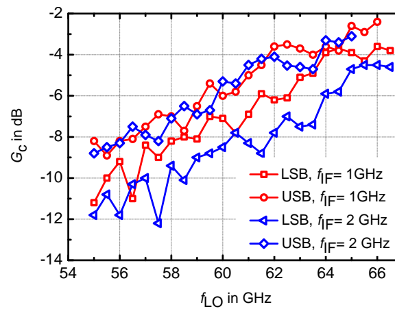
Figure 4.44: Conversion gain versus LO frequency for two different IFs
