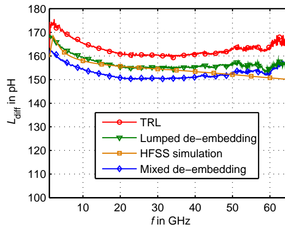
Figure 3.50: Comparison of differential inductance obtained using different de-embedding techniques and HFSS simulation
