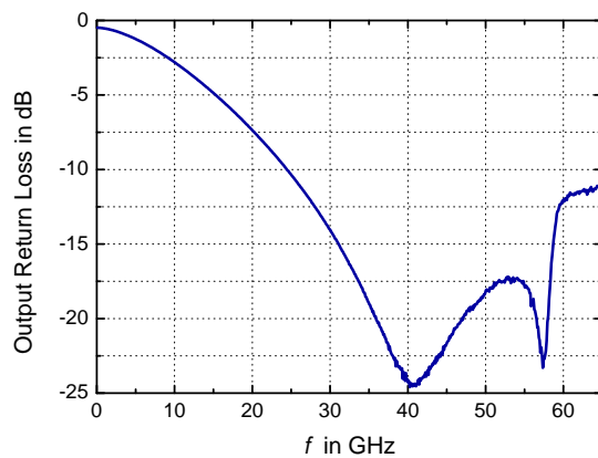
Figure 4.22: Output Return loss measured at one of the VCO outputs
