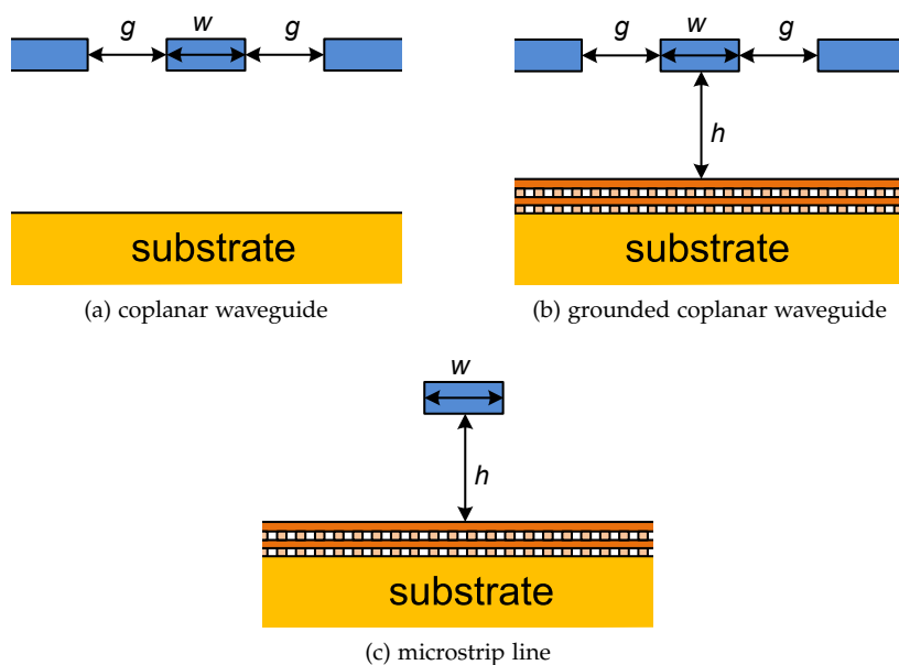
Figure 3.38: Commonly employed line types
