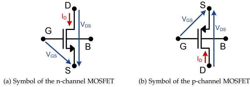
Figure 3.2: Definition of the symbols used for n and p channel MOSFETs. A missing bulk contact when using these symbols in a circuit indicates a shorting of this contact to the ground.
