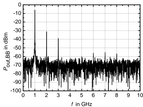
Figure 5.8: (Uncorrected) single-ended output spectrum for f_{LO}=58 GHz, f_{RF}=59 GHz and P_{RF}=-25 dBm
