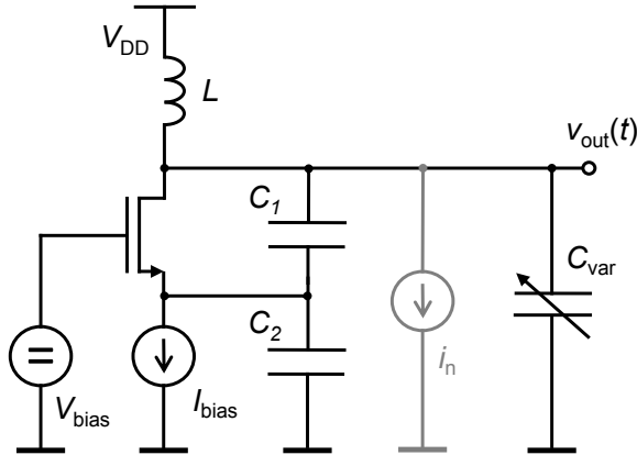
Figure 8.2: Simplified schematic of a typical single-ended VCO
