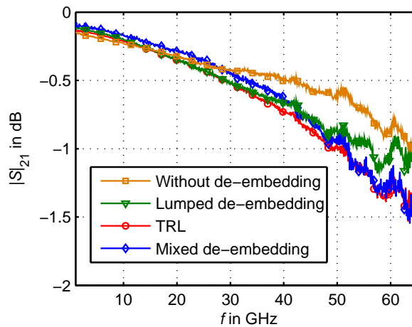
Figure 3.49: Transmission coefficient of the test inductor, with and without de-embedding of the test structure parasitics
