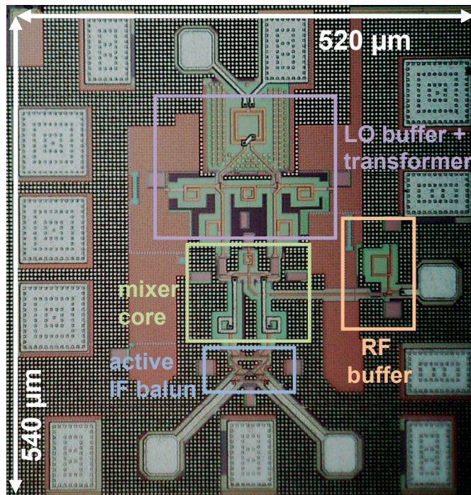
Figure 4.42: Die photograph of mixer circuit, size pad-limited
