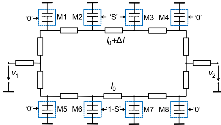
Figure C.4: Schematic of switched line phase shifter composed of RF MEMS capacitive switches and TLs
