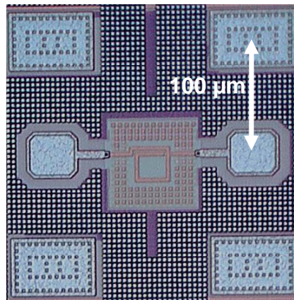
Figure 3.47: Die photo of the measured test structure containing two error two-ports and the IUT
