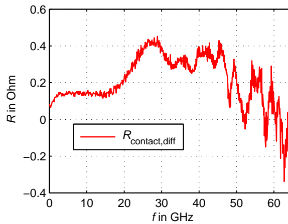
Figure 3.43: Difference between contact resistance on aluminum and on gold obtained from the measurement of microstrip line test-structures
