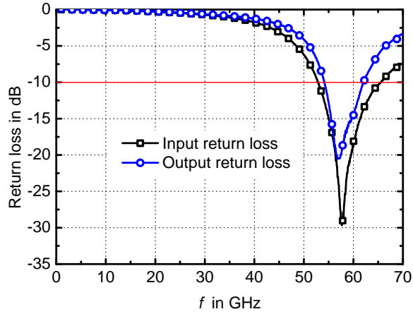
Figure 4.8: Measured return loss of the redesigned LNA biased at V_{DD} = 1\text{ V}
