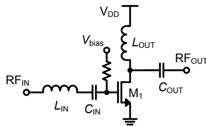
Figure 4.41: Common-source buffer amplifier added to the RF output port of the mixer
