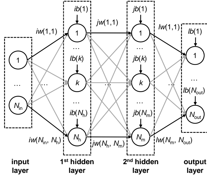
Figure 8.5: Schematic of a multi-layer perceptron with two hidden layers.
