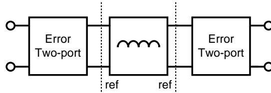
Figure 3.44: Error two-ports during TRL calibration are considered to be black boxes, no assumptions are made concerning the inside
