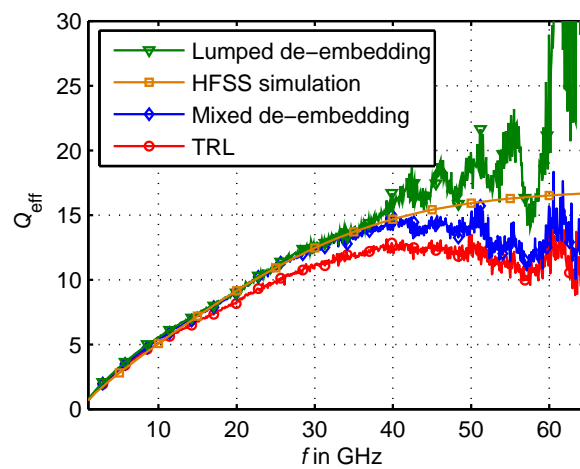
Figure 3.51: Comparison of effective quality factor from different de-embedding techniques and HFSS simulations
