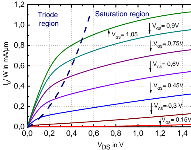
Figure 3.6: Output characteristic of a 65 nm LVT GP n-channel MOSFET, based on the simulation using DK models.
