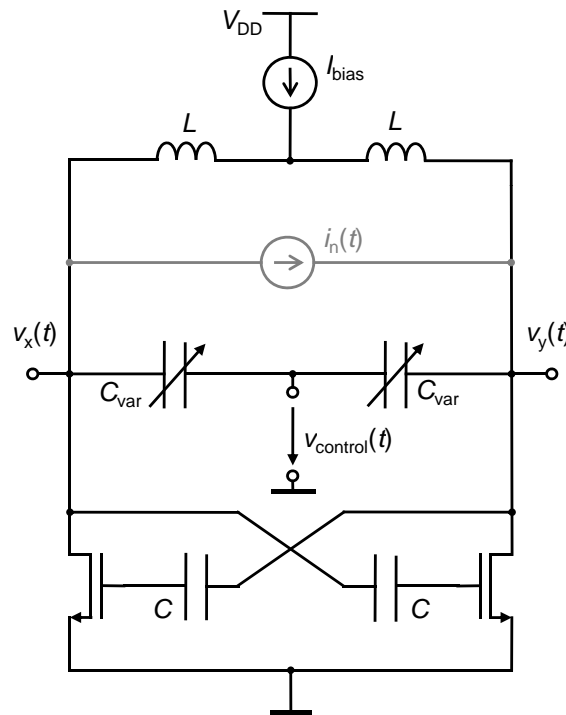
Figure 8.3: Simplified schematic of a typical integrated state-of-the-art VCO with differential outputs
