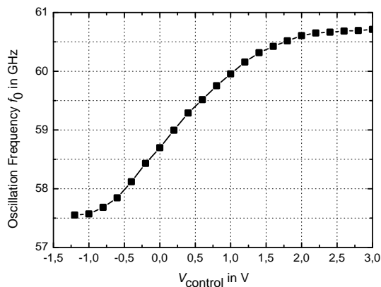
Figure 4.20: Measured tuning curve of the VCO
