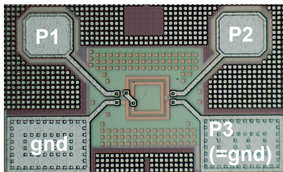
Figure 3.31: Die photo of the single-coil transformer test structure
