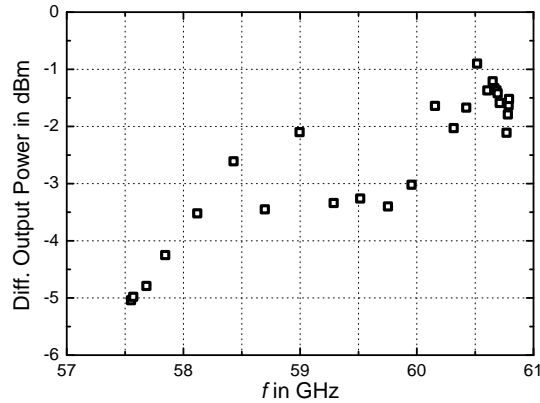
Figure 4.21: Measured differential output power
