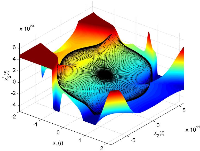
Figure 8.11: Function f() approximated by the neural network (colored plane) versus trajectory used to train it (solid line with dots to indicate actual values), v_{\text{control}} = 0\text{ V} .
