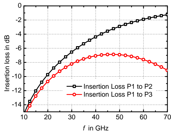
Figure 3.33: Simulated insertion loss from port P1 to ports P2 and P3, P4 at ground potential, P1-P3 terminated in 50 \Omega
