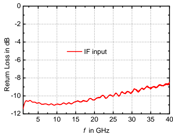
Figure 4.46: Measured input matching at the IF port
