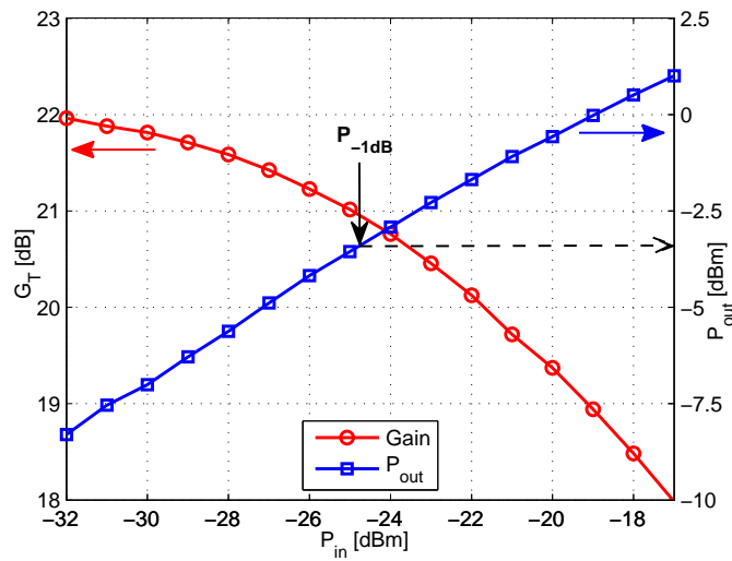
Figure 4.5: Plot of measured transducer power gain G_T and output power P_{out} versus input power P_{in} to obtain the 1 dB compression point.
