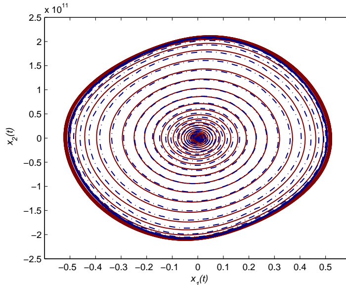
Figure 8.20: Trajectory obtained from SPECTRE-simulation (red, solid line) versus VHDL-AMS model (blue, dotted line)
