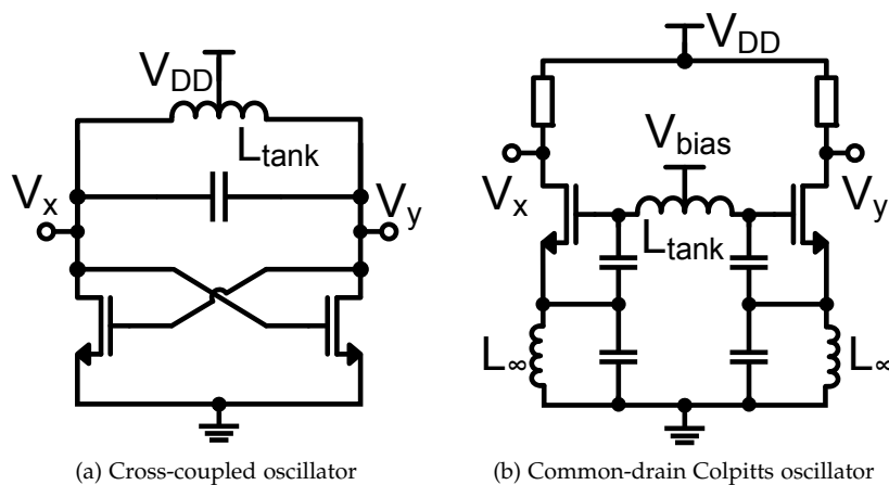
Figure 4.10: Commonly used architectures for 60 GHz VCOs
