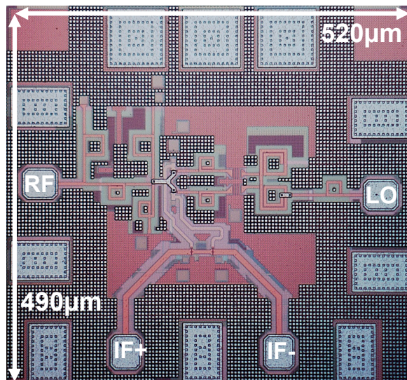
Figure 4.29: Die photo of the fabricated down-mixer
