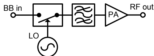
Figure 2.5: Simple direct-conversion impulse transmitter using a mm-wave switch
