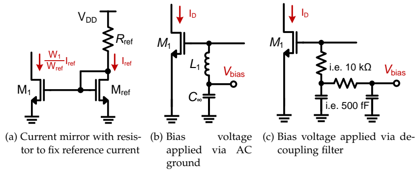
Figure 3.52: Biasing by externally applied voltage
