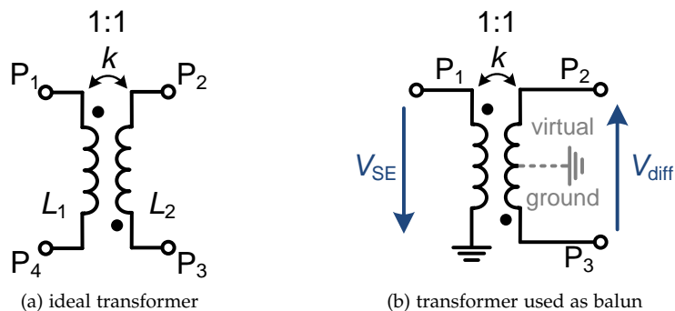
Figure 3.29: lumped 1:1 transformer with coupling factor k employed as single-ended-to-differential converter
