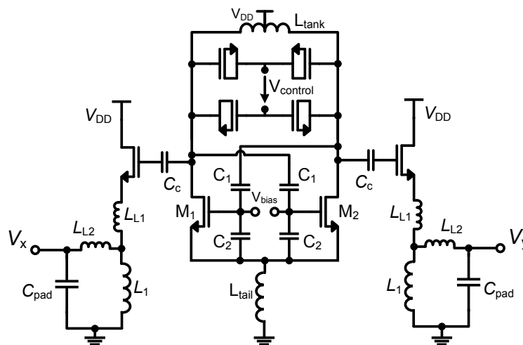
Figure 4.17: Proposed differential common-source Colpitts VCO (without bias circuitry), achieving high efficiency at 60 GHz
