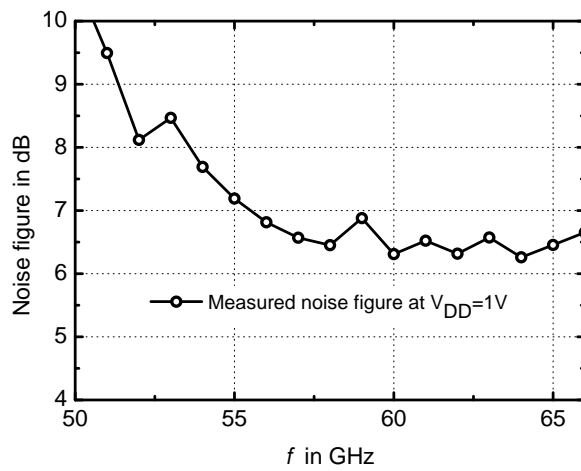
Figure 4.9: Measured noise figure of the redesigned LNA biased at V_{DD} = 1\text{ V}
