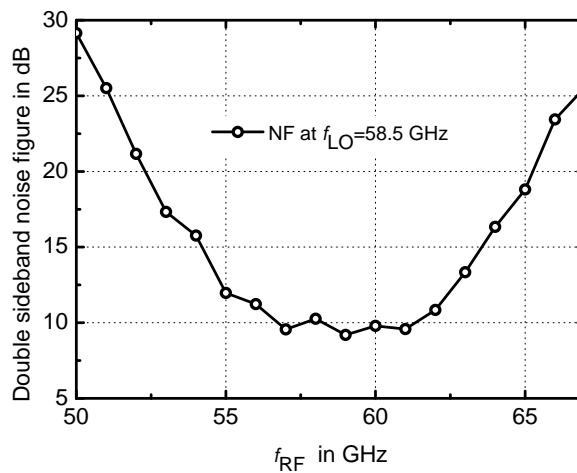
Figure 5.10: Measured double sideband noise figure at f_{LO}=58.5 GHz (influence of spectrum analyzer not removed)
