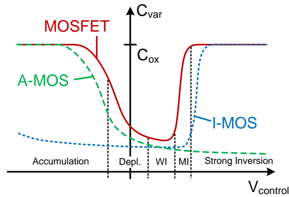
Figure 3.15: Principal capacitance variations of varactors based on MOS technology versus tuning voltage as given in [167] (indicated regions of operation are only valid for the MOSFET, which is of p-channel type if the tuning voltages is applied from the common terminal to source as for the other varactors.)
