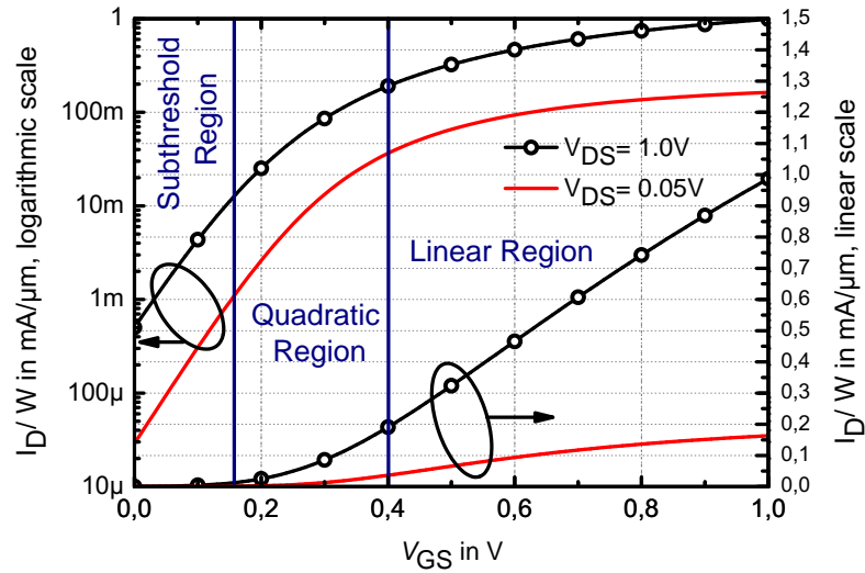
Figure 3.5: Normalized DC transfer characteristic of a 65 nm LVT GP n-channel MOSFET, based on the simulation using DK models
