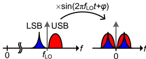
Figure 2.11: Principle of direct down-conversion using a single LO of phase \varphi and frequency f_{LO}
