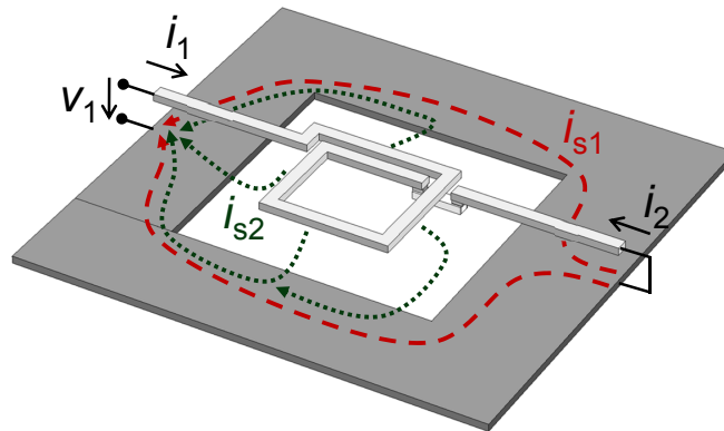
Figure 3.25: Illustration of ground return currents in a configuration used for the calculation of Y -parameters
