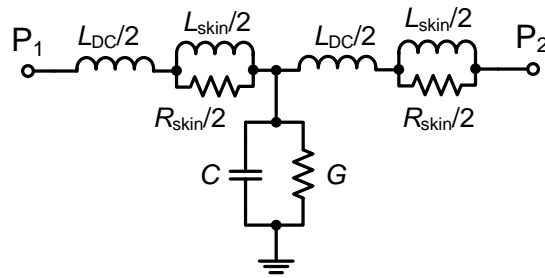
Figure 3.41: Equivalent circuit of a piece of transmission line
