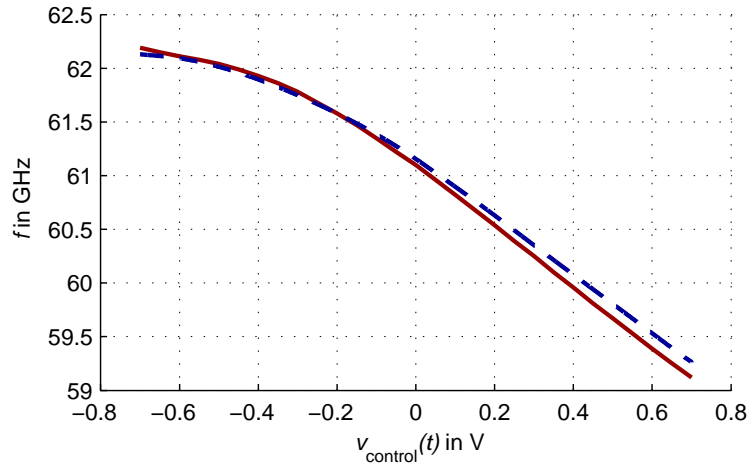
Figure 8.21: Tuning-curve of the oscillator, SPECTRE (solid line) versus VHDL-AMS (dashed line)
