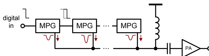
Figure 2.2: 60 GHz pulse transmitter based on Monopulse Generators (MPGs)
