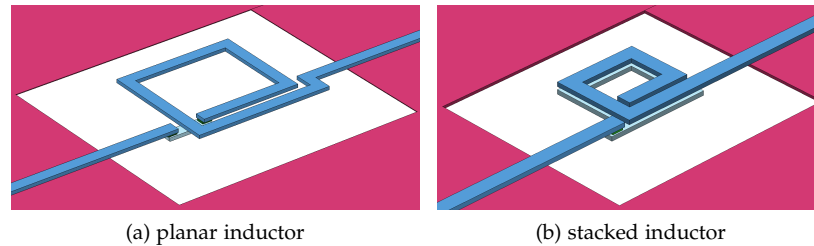
Figure 3.20: Planar inductor geometry versus stacked inductor geometry
