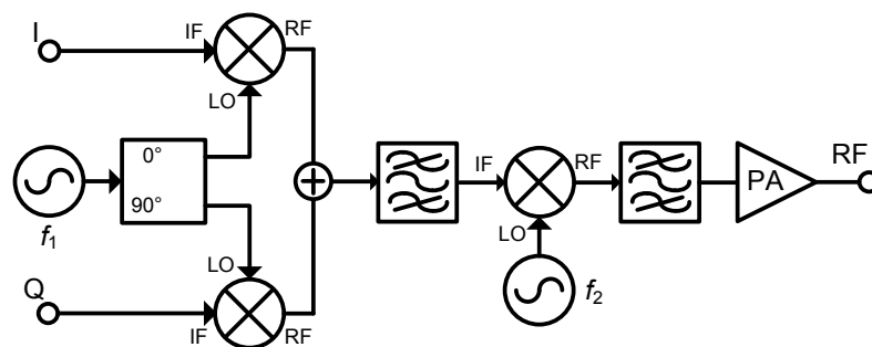
Figure 2.6: Two-step transmitter front-end using two different LO frequencies
