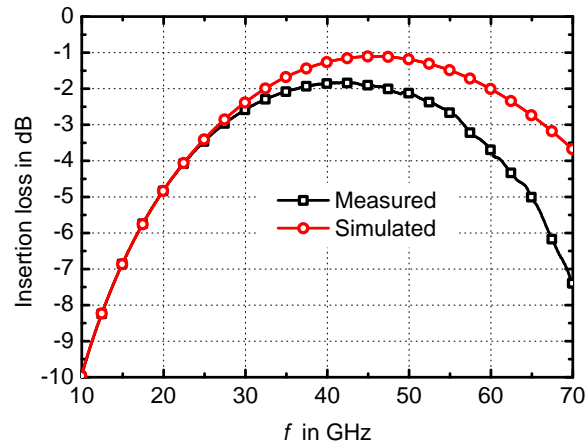
Figure 3.32: Measured versus simulated insertion loss of the one-coil transformer test-structure. The pad capacitance of 32 fF and a series inductance of 24 pF were de-embedded from the measured values at both ports, while the reference plane for the simulation is the limit of the ground ring
