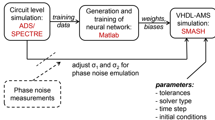
Figure 8.8: Modeling flow: from circuit level simulation to behavioral model
