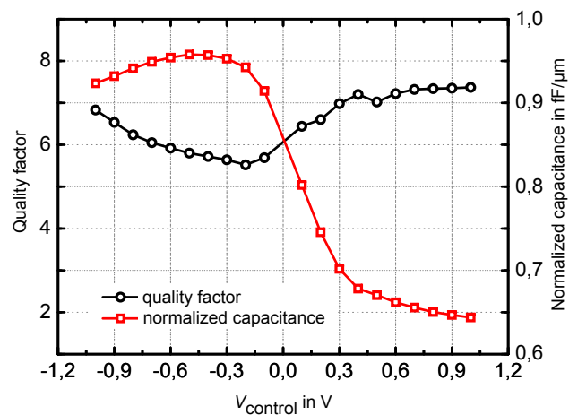
Figure 3.18: Measured normalized capacitance and effective quality factor versus V_{\text{control}} of the realized test-varactor at 60 GHz (width 51 \times 0.78\ \mu\text{m} )
