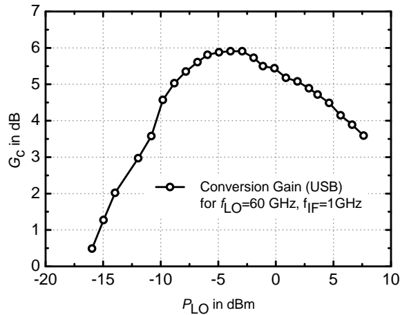
Figure 4.32: Measured conversion gain versus LO power at f_{LO} = 60 GHz and f_{IF} = 1 GHz from the upper sideband
