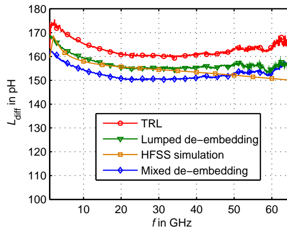
Figure 3.50: Comparison of differential inductance obtained using different de-embedding techniques and HFSS simulation
