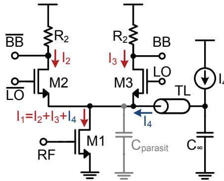
Figure 4.26: Current bleeding as proposed by B. Razavi [67]
