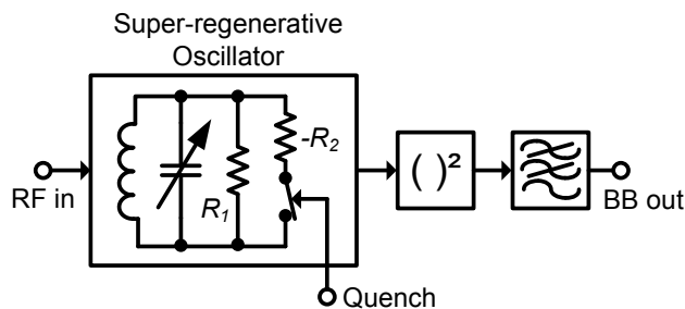
Figure 2.9: Principle of the super-regenerative receiver
