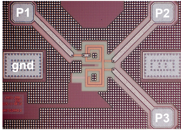
Figure 3.35: Die photo of the two-coil transformer test structure
