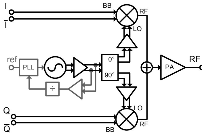
Figure 2.19: Block diagram of adopted direct conversion transmitter
