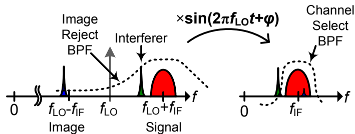
Figure 2.14: Illustrated spectrum in heterodyne down-conversion
