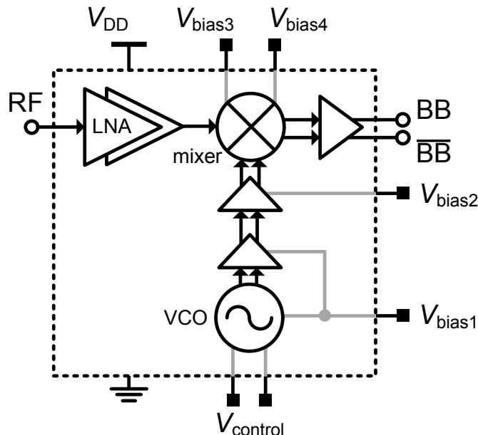
Figure 5.1: Block diagram of the realized receiver front-end with off-chip interfaces
