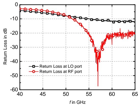
Figure 4.30: Measured return loss at LO and RF port
