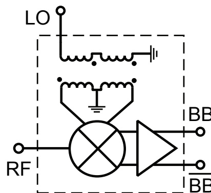
Figure 4.24: Block diagram of the downconversion mixer with integrated LO balun and baseband buffer
