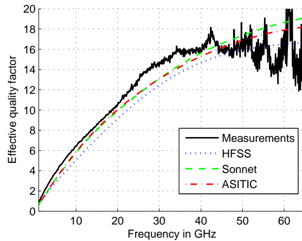
Figure 3.27: Q_{\text{eff}} of the test-inductor
