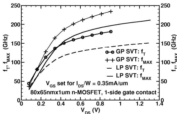
Figure 3.4: f_T and f_{max} of 65 nm NMOS transistors with 80 fingers of 1 \mu\text{m} width versus drain-source voltage, adopted from [150] with permission, Copyright IEEE 2007.
