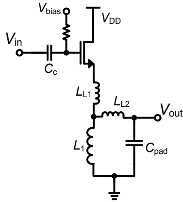
Figure 4.16: VCO source follower output buffer
