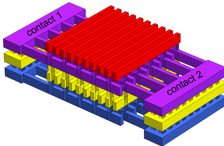
Figure 3.12: Typical structure of a MOM capacitor
