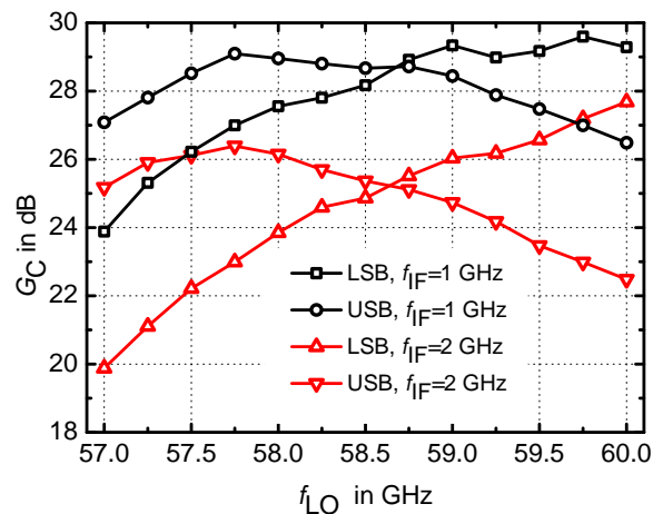
Figure 5.5: Measured power conversion gain versus LO frequency
