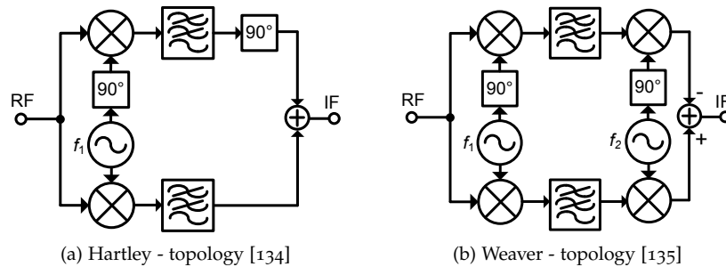
Figure 2.15: Image rejection receiver principles
