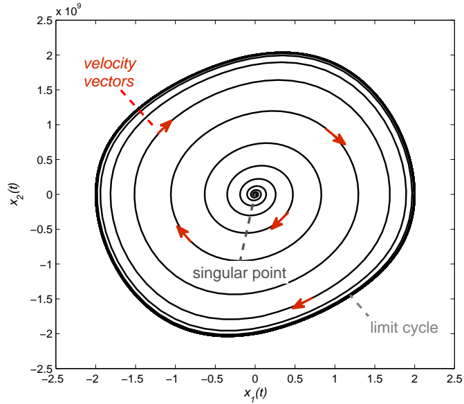
Figure 8.1: Plot of the trajectory of a Van der Pol-oscillator, simulated in VHDL-AMS. Singular point \dot{\mathbf{x}}(t) = \mathbf{0} for \mathbf{x}(t) = \mathbf{0} .
