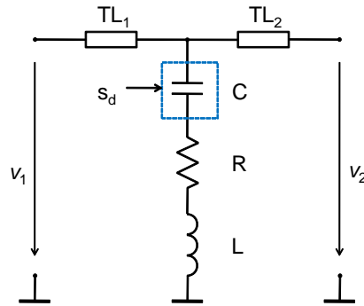
Figure C.2: RF MEMS switch equivalent circuit model
