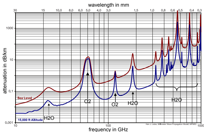
Figure 1.6: Absorption of mm-waves due to atmospheric gases at sea level and 15,000 feet altitude (courtesy of OML Inc., www.omlinc.com )
