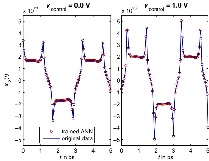
Figure 8.12: Original data (blue solid line) versus output of trained neural network (red circles) for two different control voltages (left: 0 V, right: 1 V)
