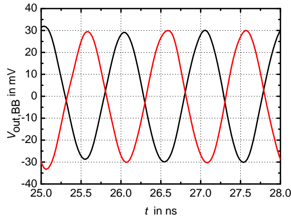
Figure 5.7: (Uncorrected) output voltages at both baseband outputs for f_{LO}=58 GHz, f_{RF}=59 GHz and P_{RF}=-45 dBm
