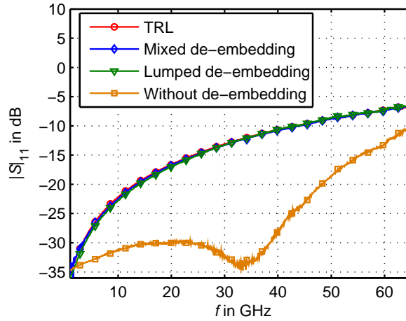
Figure 3.48: Reflection coefficient at port one of the test inductor, with and without de-embedding of the test structure
