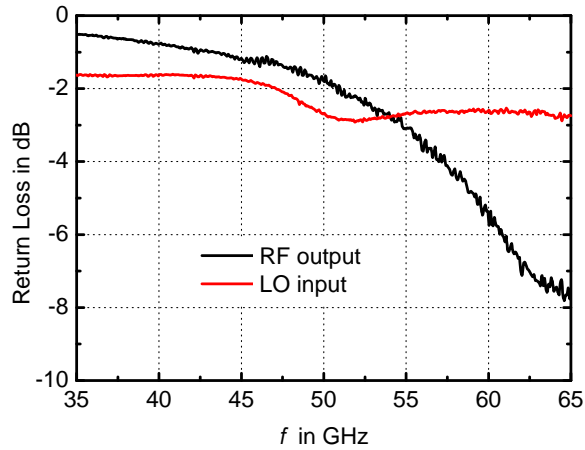
Figure 4.47: Measured LO input and RF output matching
