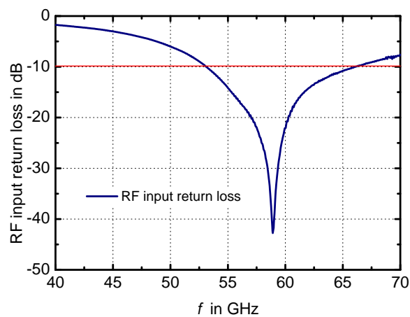
Figure 5.3: Return loss measured at the RF input of the receiver front-end
