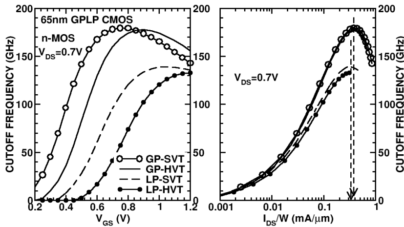
Figure 3.3: f_T of 65 nm NMOS transistors with 80 fingers of 1 \mu\text{m} width versus gate-source voltage and drain current density, adopted from [150] with permission, Copyright IEEE 2007.
