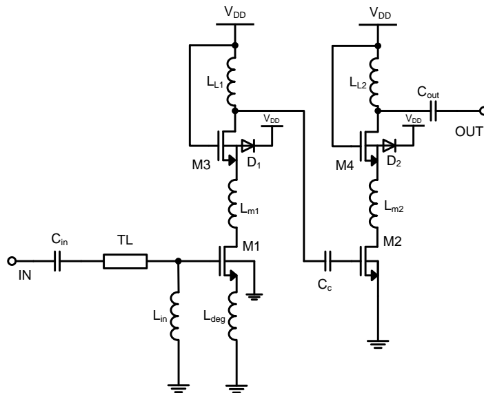
Figure 4.1: Simplified schematic of the designed two-stage cascode LNA (parasitic diodes D_1 and D_2 due to deep n-wells surrounding M3 and M4)
