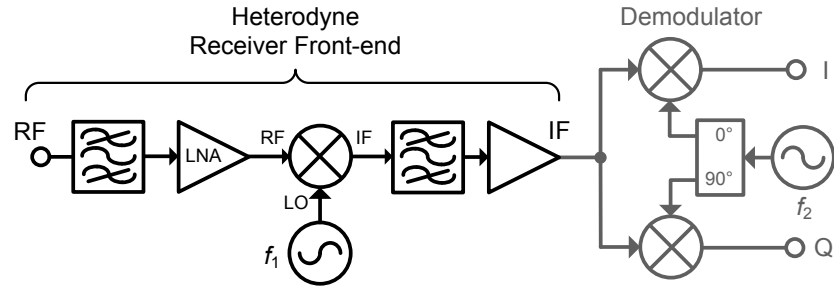
Figure 2.13: Block diagram of heterodyne receiver front-end with subsequent I/Q demodulator
