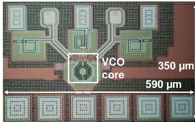
Figure 4.18: Die photo of the fabricated 60 GHz VCO (size pad-limited)
