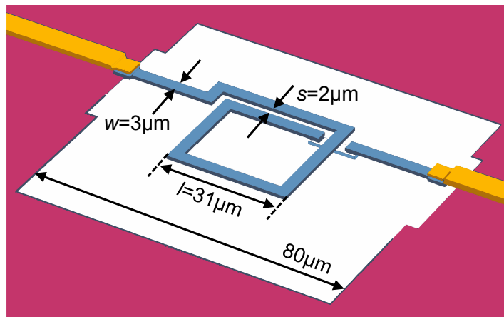
Figure 3.21: 3D view of the inductor used for the following analyses
