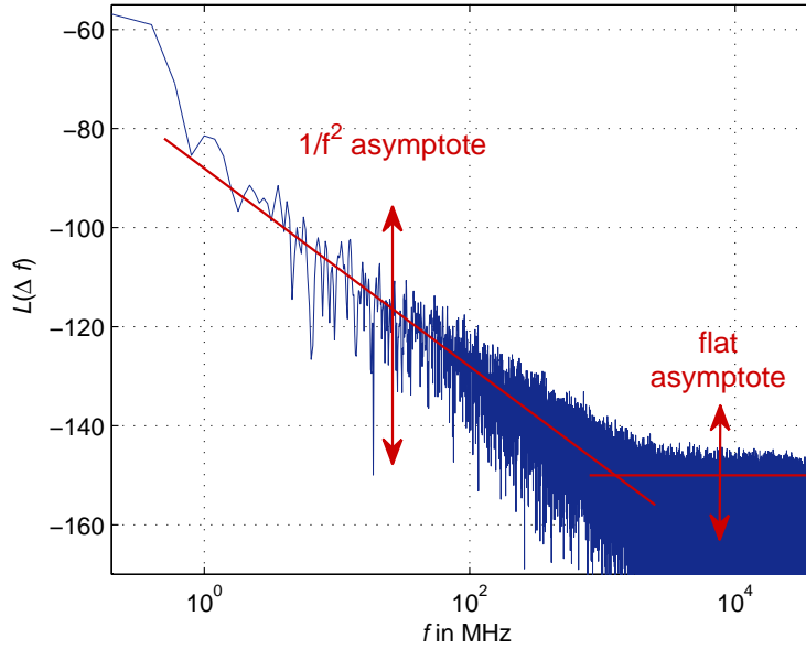
Figure 8.18: Phase noise characteristics shown by the VHDL-AMS model. The height of the asymptotes is set by \sigma_1 and \sigma_{2x}/\sigma_{2y} .
