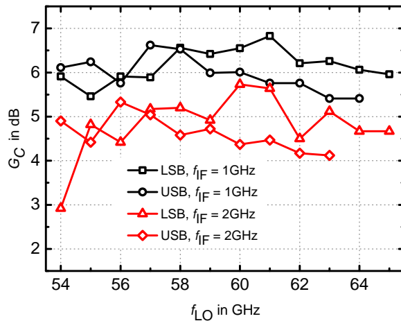
Figure 4.33: Conversion gain G_C versus LO frequency for two different intermediate frequencies, both in upper (USB) and lower sideband (LSB).
