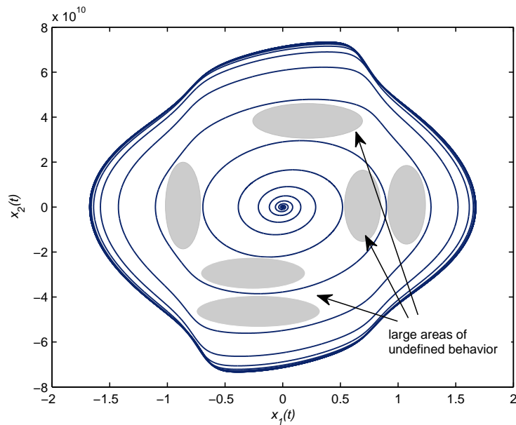
Figure 8.9: Trajectory of an oscillator with fast startup: large uncovered areas in the input space yielding neural networks poorly approximating the desired function.
