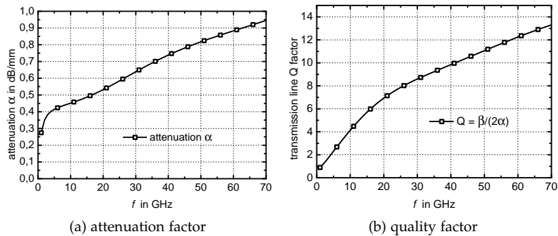
Figure 3.40: Simulated line parameter \alpha and associated Q-factor of a microstrip line with w = 6 \mu\text{m} , situated in the alucap layer of the STMicronics 65 nm CMOS technology
