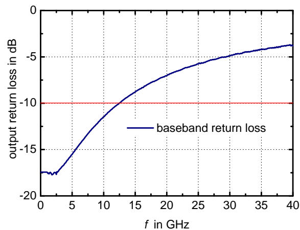
Figure 5.4: Return loss measured at the baseband outputs of the receiver front-end
