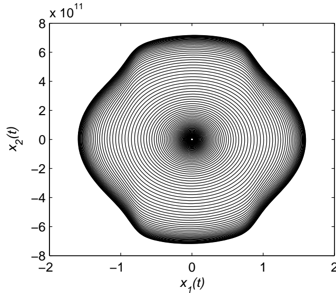
Figure 8.4: Trajectory of a 60 GHz differential Colpitts oscillator in the two-dimensional state space as defined in (8.12)
