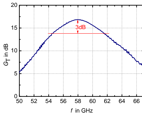
Figure 4.7: Measured transducer power gain of the redesigned LNA at V_{DD}=1 V
