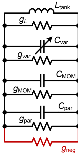
Figure 4.13: Steady-state parallel oscillator model
