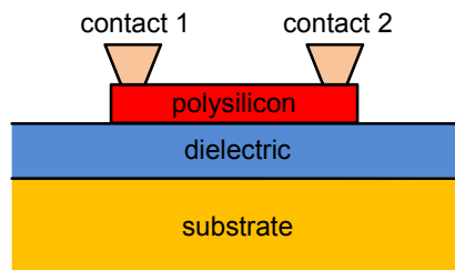
Figure 3.14: Principal structure of a polysilicon resistor
