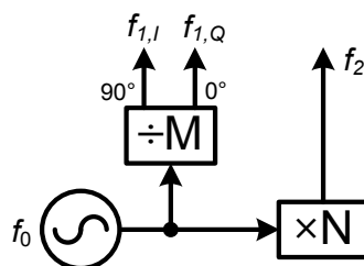
Figure 2.7: Frequency generation from a single synthesizer using dividers and multipliers
