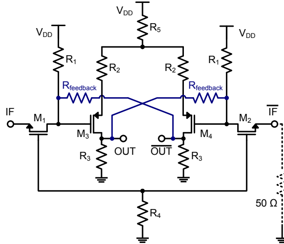
Figure 4.39: Simplified schematic of the IF buffer / active balun
