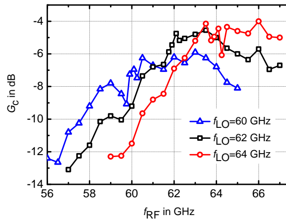
Figure 4.45: Conversion gain versus RF for three LO frequencies
