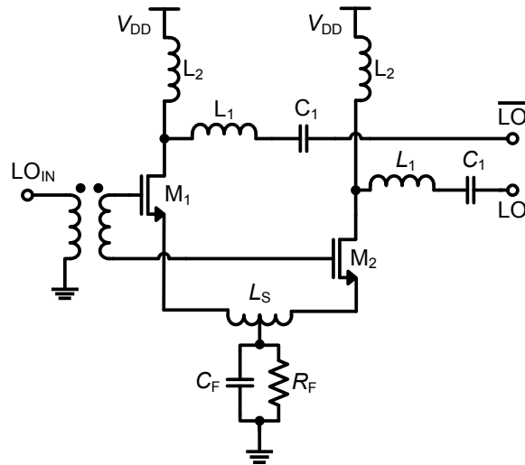
Figure 4.40: Differential LO buffer amplifier with transformer balun at the input
