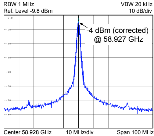
Figure 4.19: Measured oscillator output spectrum at 58.92 GHz ( V_{\text{control}}=0 V)
