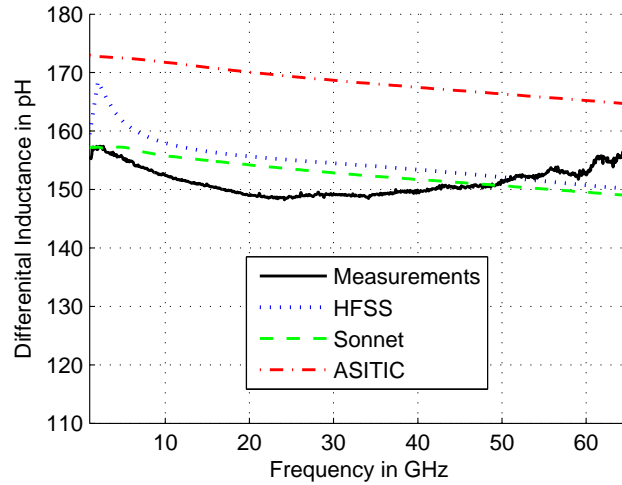
Figure 3.26: L of the test-inductor
