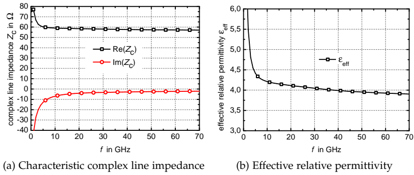
Figure 3.39: Simulated parameters Z_c and \epsilon_{\text{eff}} of a microstrip line with w = 6 \mu\text{m} , situated in the alucap layer of STMicronics' 65 nm CMOS technology
