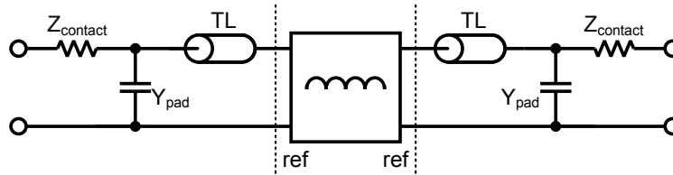
Figure 3.46: Proposed equivalent circuit model for the error two ports surrounding the inductor under test
