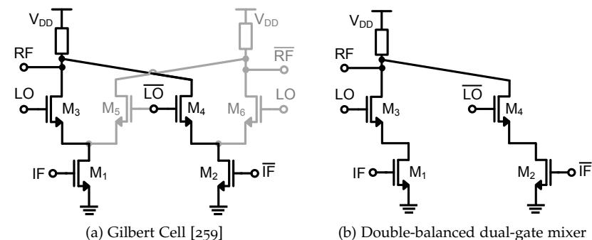
Figure 4.36: Comparison of Gilbert cell (differential output) to dual gate mixer (single-ended output)
