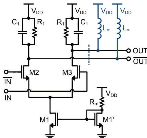
Figure 4.28: Differential pair serving as baseband buffer for the down-converter output
