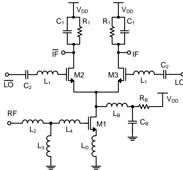
Figure 4.27: Simplified schematic of the mixer core without biasing details
