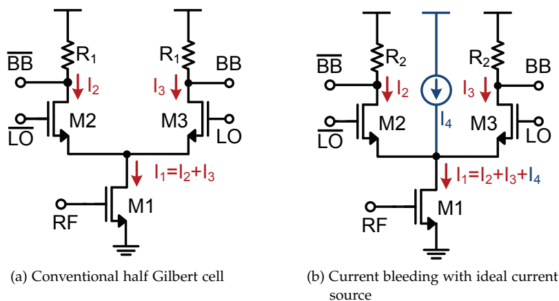
Figure 4.25: Half Gilbert cell with and without current bleeding
