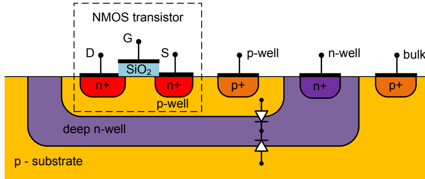
Figure 3.10: n-channel MOS transistor embedded in a deep n-well (parasitic diodes between the wells and the substrate are indicated)
