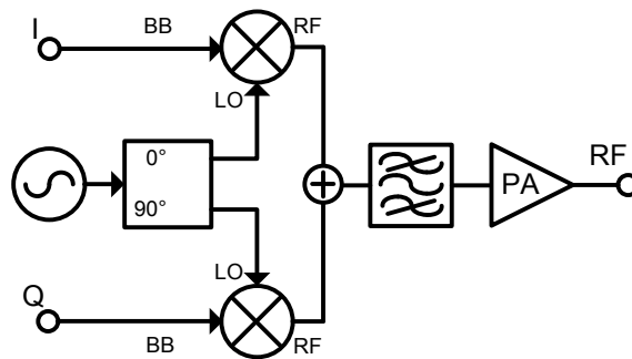
Figure 2.4: Simplified architecture of a direct conversion transmitter
