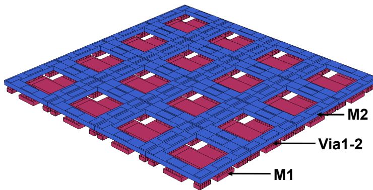
Figure 3.55: Ground plane consisting of shunted metal layers M1 and M2
