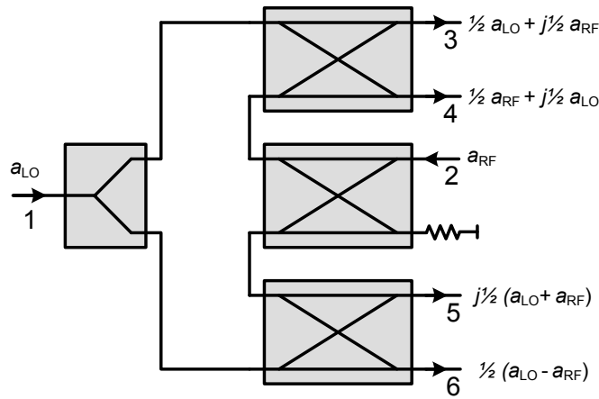
Figure 2.17: Typical implementation of a six-port demodulator
