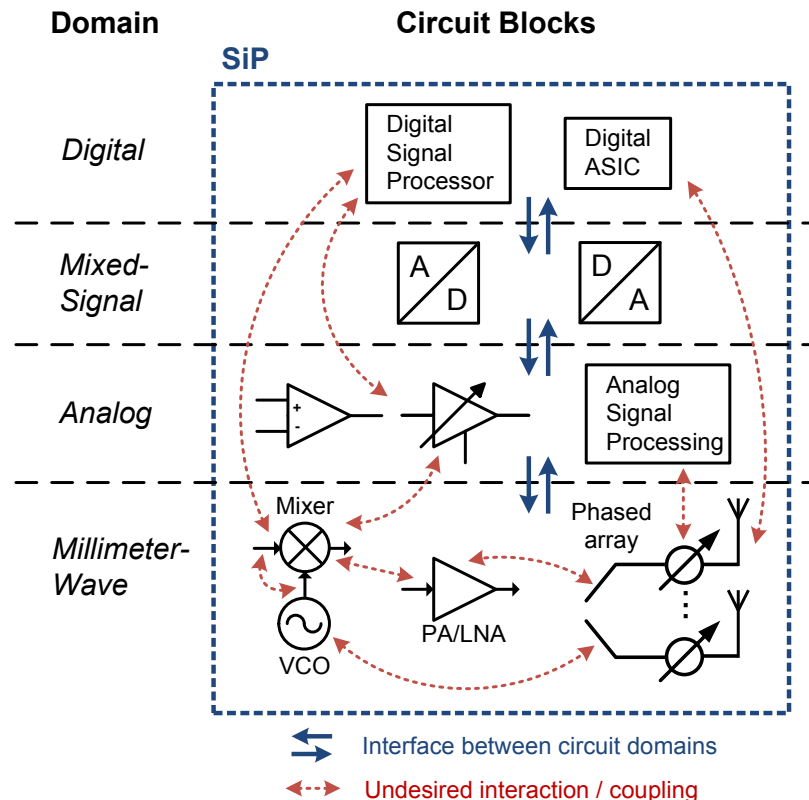
Figure 7.2: Illustration of the different domains of a mm-wave System in Package (SiP) showing typical building blocks and highlighting the issue of parasitic coupling.
