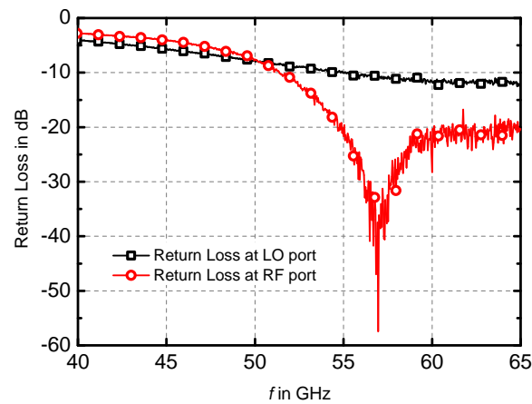
Figure 4.30: Measured return loss at LO and RF port
