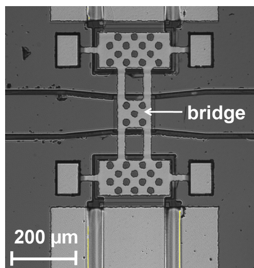
Figure C.1: Die photo of a 60 GHz RF MEMS switch
