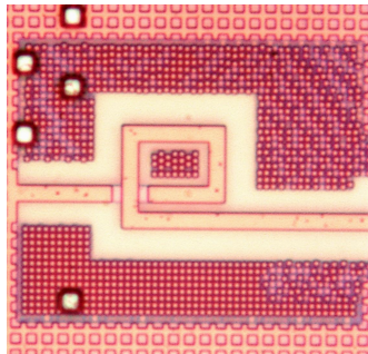
Figure 3.54: Microphotograph of inductor surrounded by dense dummy metal
