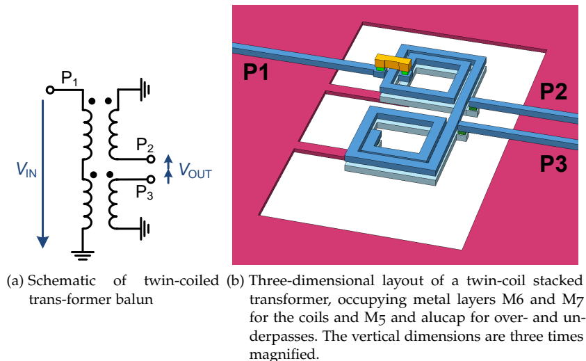
Figure 3.34: Schematic and geometry of twin-coil transformer
