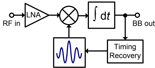
Figure 2.10: Principle of the impulse correlation receiver
