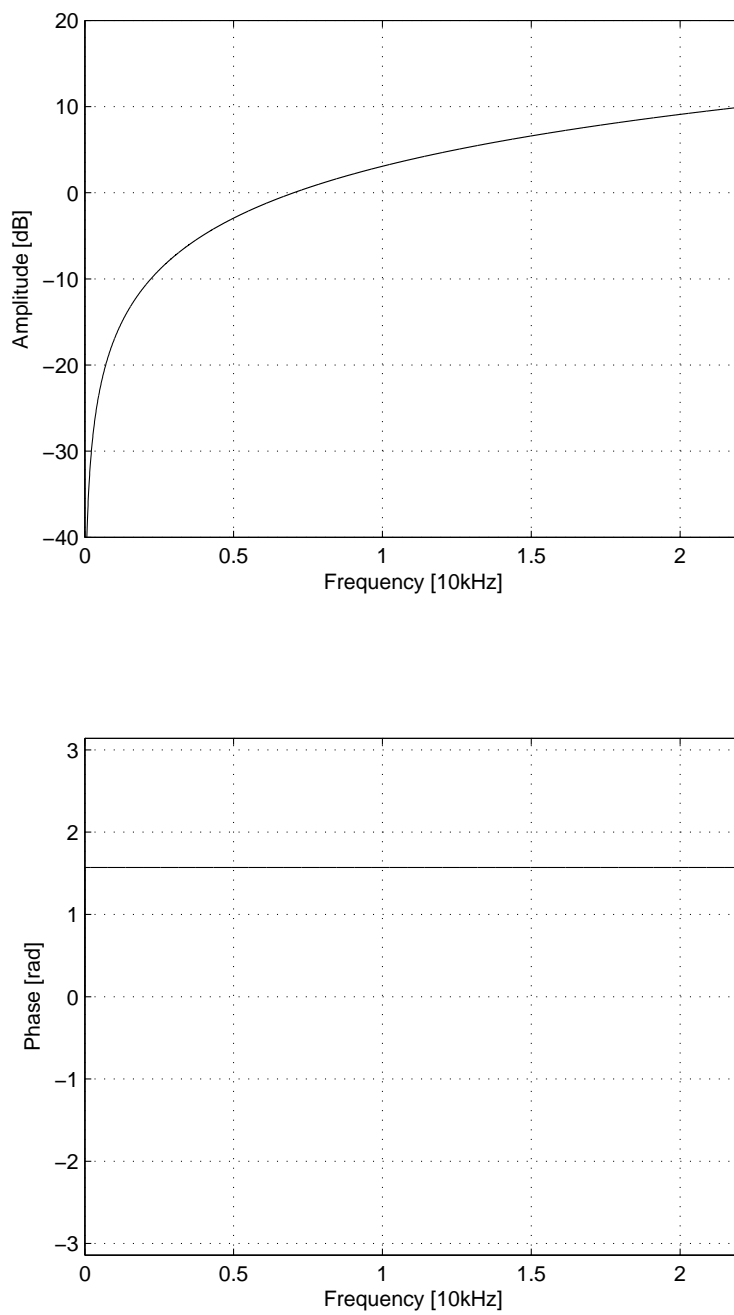
Figure 3.2: The radiation model L(\omega) = j\omega
