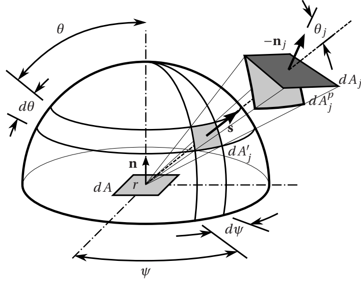
Figure 6.2: Solid angle
