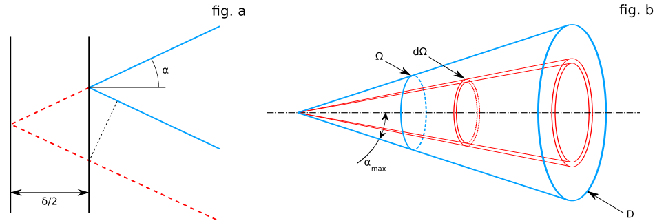
FIGURE 2.15 – Faisceaux lumineux
