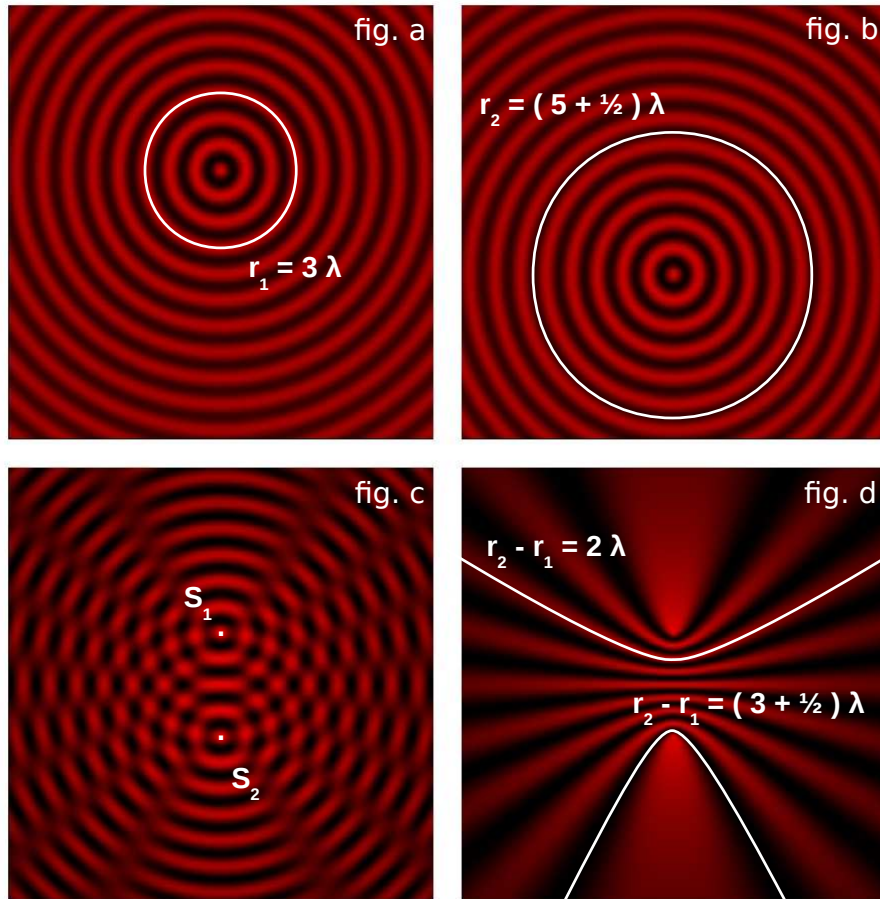
FIGURE 2.3 – Ondes circulaires
