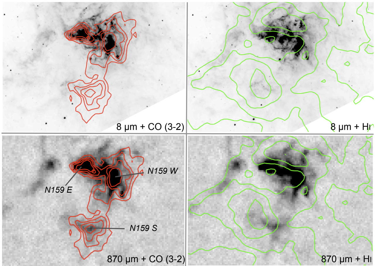
Figure 7.10. IRAC4 (8 \mu\text{m} ) and LABOCA (870 \mu\text{m} ) images with ASTE ^{12}\text{CO}(J = 3 \rightarrow 2) and HI contours overlaid. The HI contours are 5 \times 10^{21} , 6 \times 10^{21} and 7 \times 10^{21} atom \text{cm}^{-2} . The CO contours are 2, 8, 14, 27 K \text{km s}^{-1} . We thank Akiko Kawamura for the CO map.
