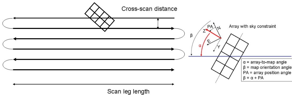
Figure 8.6. Left: Schematic view of a PACS scan map (6 scan lines). Right: Scheme of the reference angles of the array in sky constraint.
