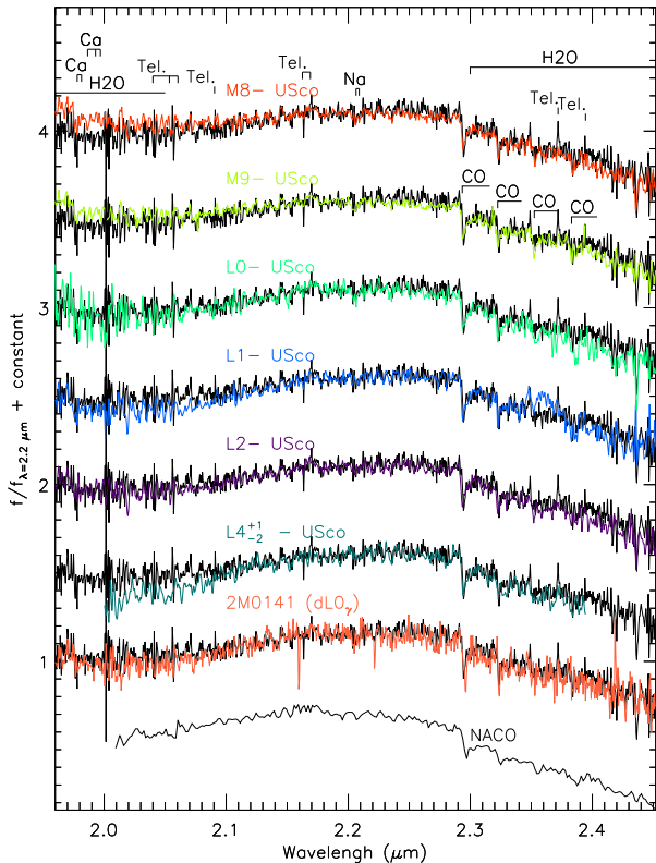
Fig. 3. K-band SINFONI spectrum of AB Pic b (black) compared to young ( \sim 5 Myrs) Upper-Sco brown-dwarf spectra (color) and to the young isolated object 2M0141 (classified dL 0y ). \chi^2 are minimized for young L0 and L2 dwarfs. The shape is not reproduced well by old field dwarfs. The low-resolution ( R_\lambda=550 ) NACO spectrum is overlotted at the bottom for comparison.
