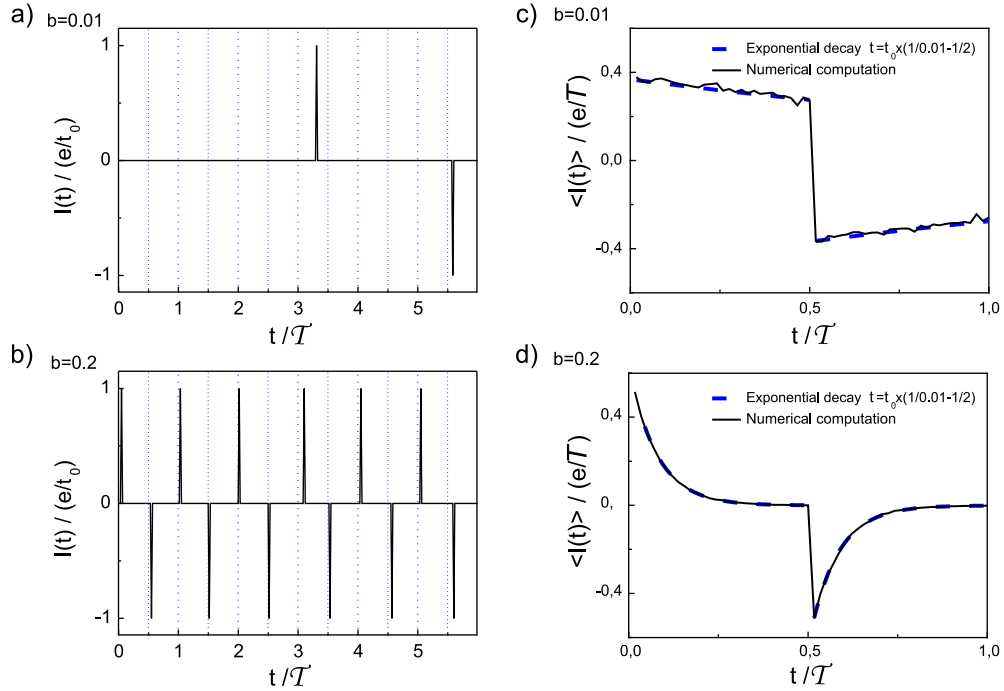
Figure 1.11: AC current emitted by the source, calculated with the heuristic model. a) and b) emitted current as a function of time for escape probability b = 0.01 ( a ), and b = 0.2 ( b ). A peak (dip) appears whenever an electron (hole) is emitted. c) and d) statistical average of the current displayed on one period of the drive, for b = 0.01 ( c ), and b = 0.2 ( d ). The calculations (black lines) display the expected exponential decay with a characteristic time given by \tau = \tau_0(1/b - 1/2) .
