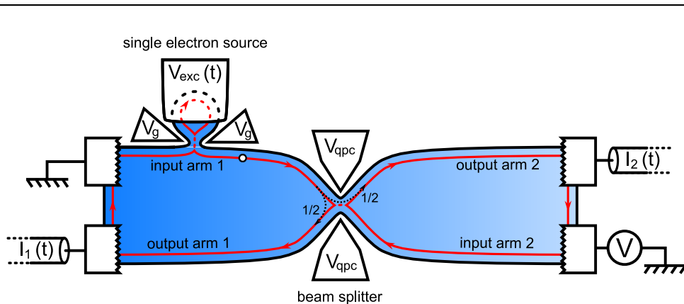
Figure 6: Schematic of the single-charge HBT experiment: a single electron emitter is placed at the first input arm of a QPC, acting as a beam splitter. The correlation of the current fluctuations in the two output arms are measured. The ohmic contact on the second input arm can be biased to measure the energy distribution of the emitted charges.
