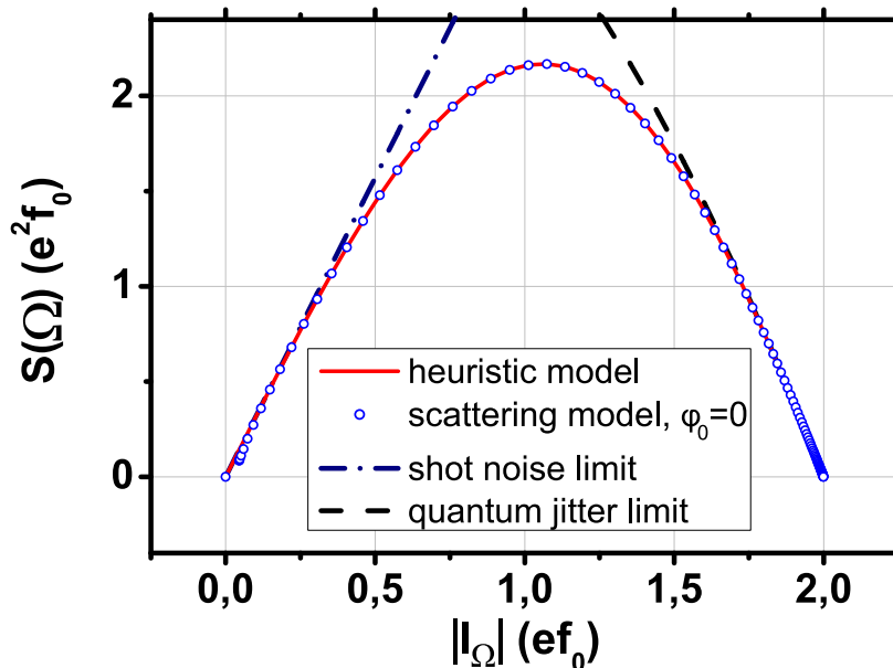
Figure 2.10: Calculated noise in the heuristic model (red line) and in the scattering model (blue circles) as a function of the modulus of the first harmonic of the average AC current. The shot noise and quantum jitter limits (dashed lines) are given by the usual shot noise formula and Eq.2.30.
