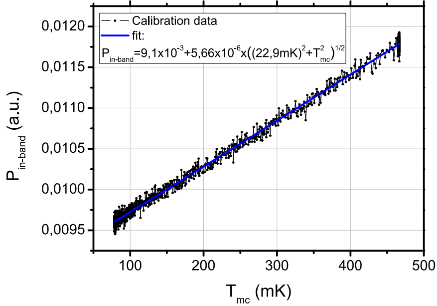
Figure 4.13: Calibration of the low-frequency measurement setup: the thermal noise of the measurement load is recorded as the mixing chamber cools down to the base temperature (averaging time: \sim 3s ). We repeat the calibration several time to estimate the error on the conversion coefficient.
