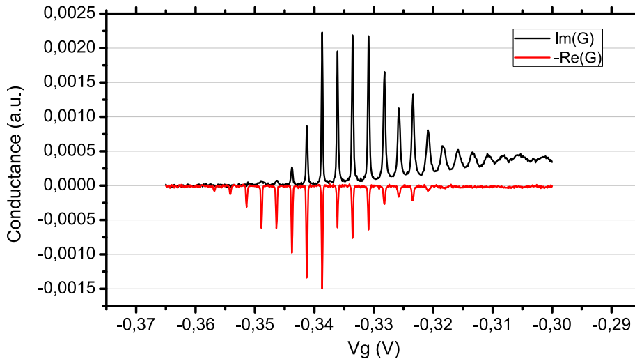
Figure 1.5: Conductance trace at 1.5 GHz as a function of the QPC gate voltage V_g , measured on sample S528-11 . The applied magnetic field ( B \approx 1.8 T ) corresponds to a filling factor \nu = 4 .
