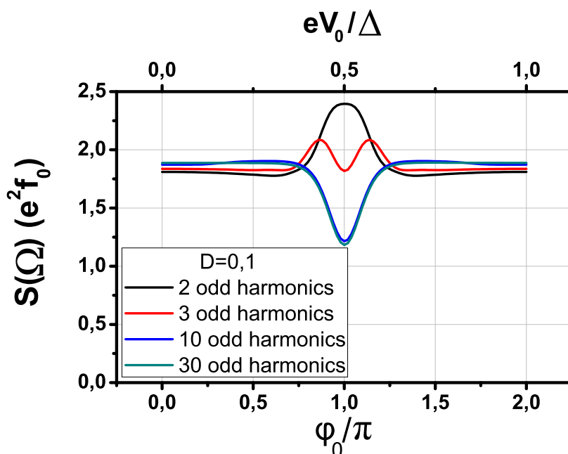
Figure 2.6: Calculated noise as a function of the dot equilibrium potential, for a square excitation signal containing 2, 3, 10 and 30 odd harmonics (resp. black, red, blue and gray line). The temperature is taken equal to 100mK .
