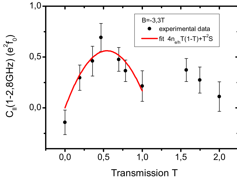
Figure 3.25: High frequency noise in the HTB geometry, measured as a function of the transmission T at B = -3.3T . The fit (red line) yields n_{e/h} = 0.51 \pm 0.07 and S = 0.16 \pm 0.1e^2 f_0 .
