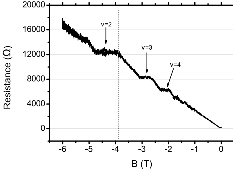
Figure 3.13: Measurement of the two-point resistance between the bias contact and the measurement contact as a function of the magnetic field. For magnetic fields larger than 1T , the resistance presents plateaus corresponding to integer values of the filling factor. We focus our study for B = -3.9T , indicated by the dashed line.
