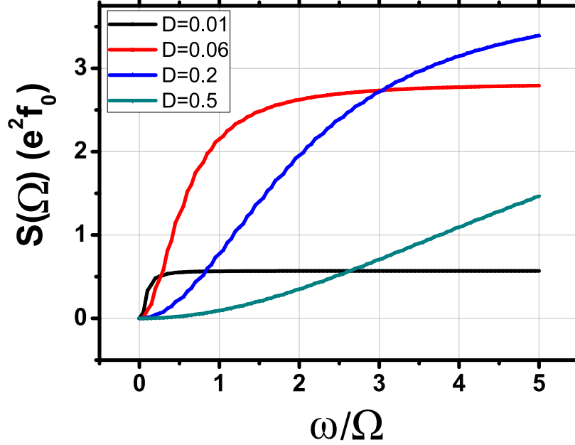
Figure 2.3: Calculated noise as a function of the measurement frequency in the injection regime: 2eV_{exc} = \Delta , \phi_0 = 0 . We have taken f_0 = 1.5GHz (that is \hbar\Omega/k_B = 0.07K ), and \Delta = 4K .
