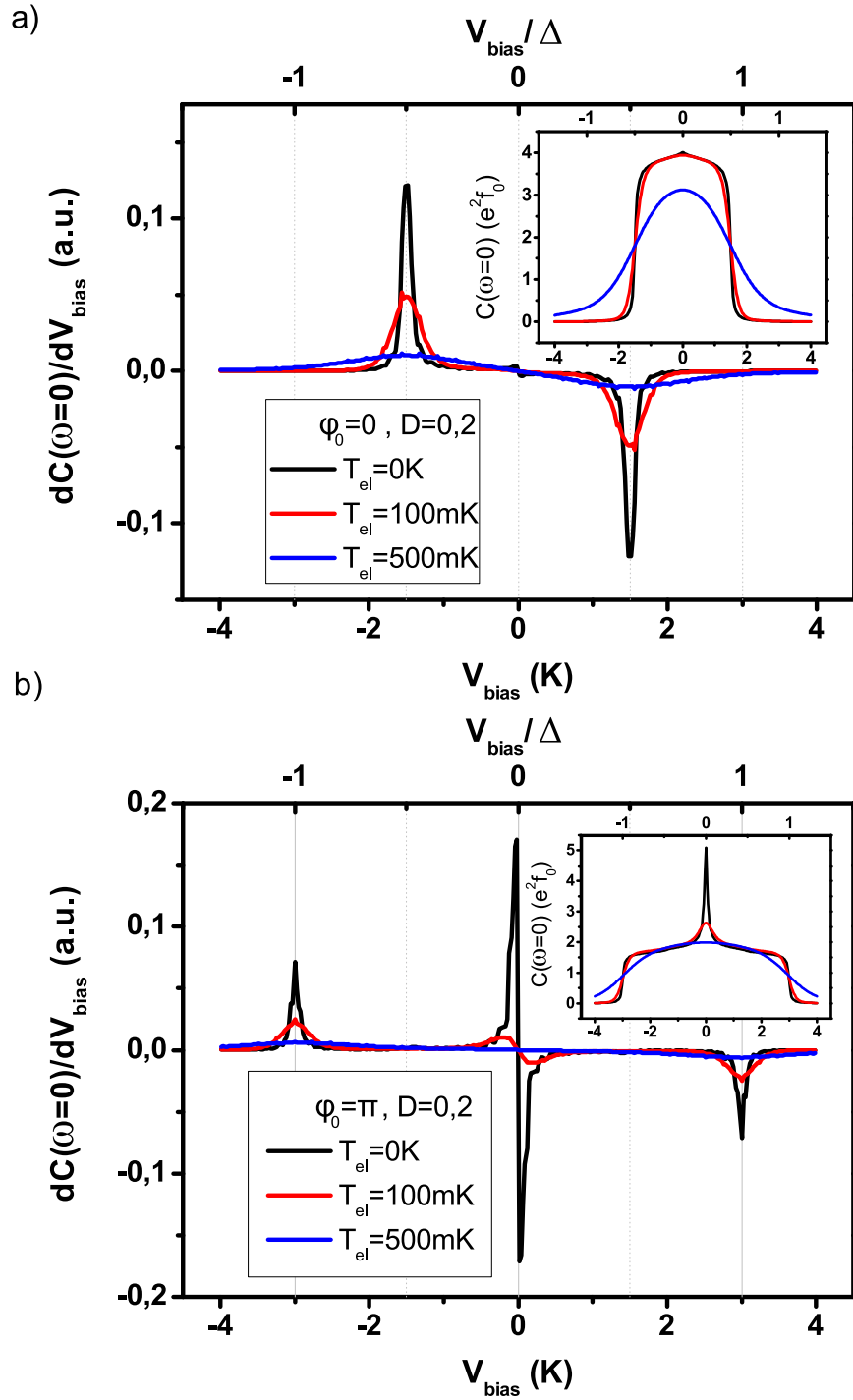
Figure 3.10: \partial C(\omega = 0)/\partial V_{bias} versus V_{bias} , for increasing temperatures: 0K (black), 100mK (red), 500mK (blue). a) anti-resonant case \phi_0 = 0 . b) resonant case \phi_0 = \pi . Insets: variation of C(\omega = 0) with V_{bias} , for the same temperatures.
