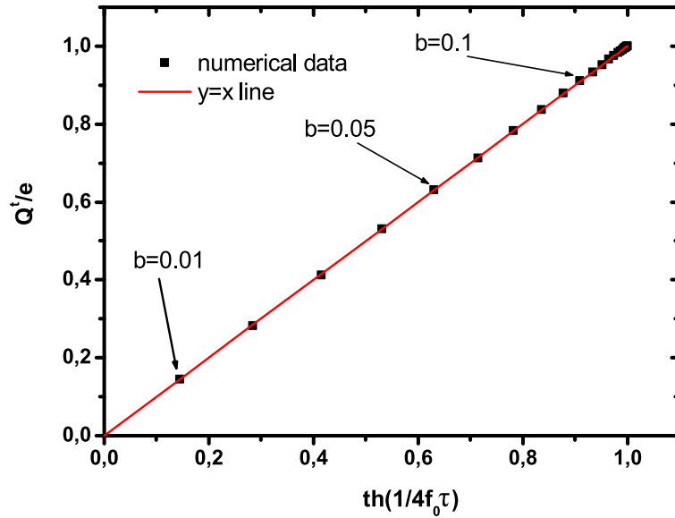
Figure 1.13: Average transferred charge per half-period versus \tanh(1/4f_0\tau) , in the heuristic model. The red line has a unit slope, thus verifying Eq.1.50.
