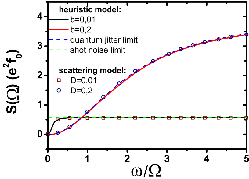
Figure 2.9: Dependence of the noise in the heuristic model (full lines) and in the scattering model for \phi_0 = 0 (hollow symbols) on the measurement frequency \omega . The dashed lines correspond to analytical calculations of the shot noise and quantum jitter limit, using Eqs.2.25 and 2.27.
