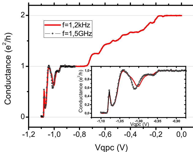
Figure 3.15: Measured transmission of the central QPC as a function of V_{qpc} , at \nu = 2 . Red line: low-frequency measurement ( 1.2kHz ). Black circles: RF measurement ( 1.5GHz ). Inset: close-up view of the transmission of the outer channel versus V_{qpc} .
