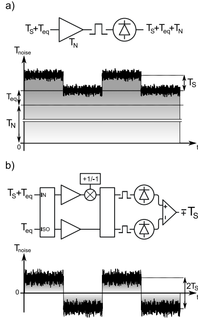
Figure 4.2: a) Direct amplification technique: the signal is amplified, filtered and applied to the square law detector, measuring the sum of the noise temperature of the signal and the measurement load T_S + T_{eq} and the noise temperature of the amplifier T_N . Below is a schematic representation of the measured lock-in voltage as a function of time: the value of the lock-in voltage alternatively switches between T_{eq} + T_N and T_S + T_{eq} + T_N . The peak-peak amplitude of the detected square voltage is equal to T_S . b) Our setup detects and modulates the difference between the two input noises T_S + T_{eq} and T_{eq} , that is \mp T_S . The lock-in voltage is then centered on zero while its peak-peak amplitude is equal to 2T_S . The standard deviation is however \sqrt{2} times larger in our setup.
